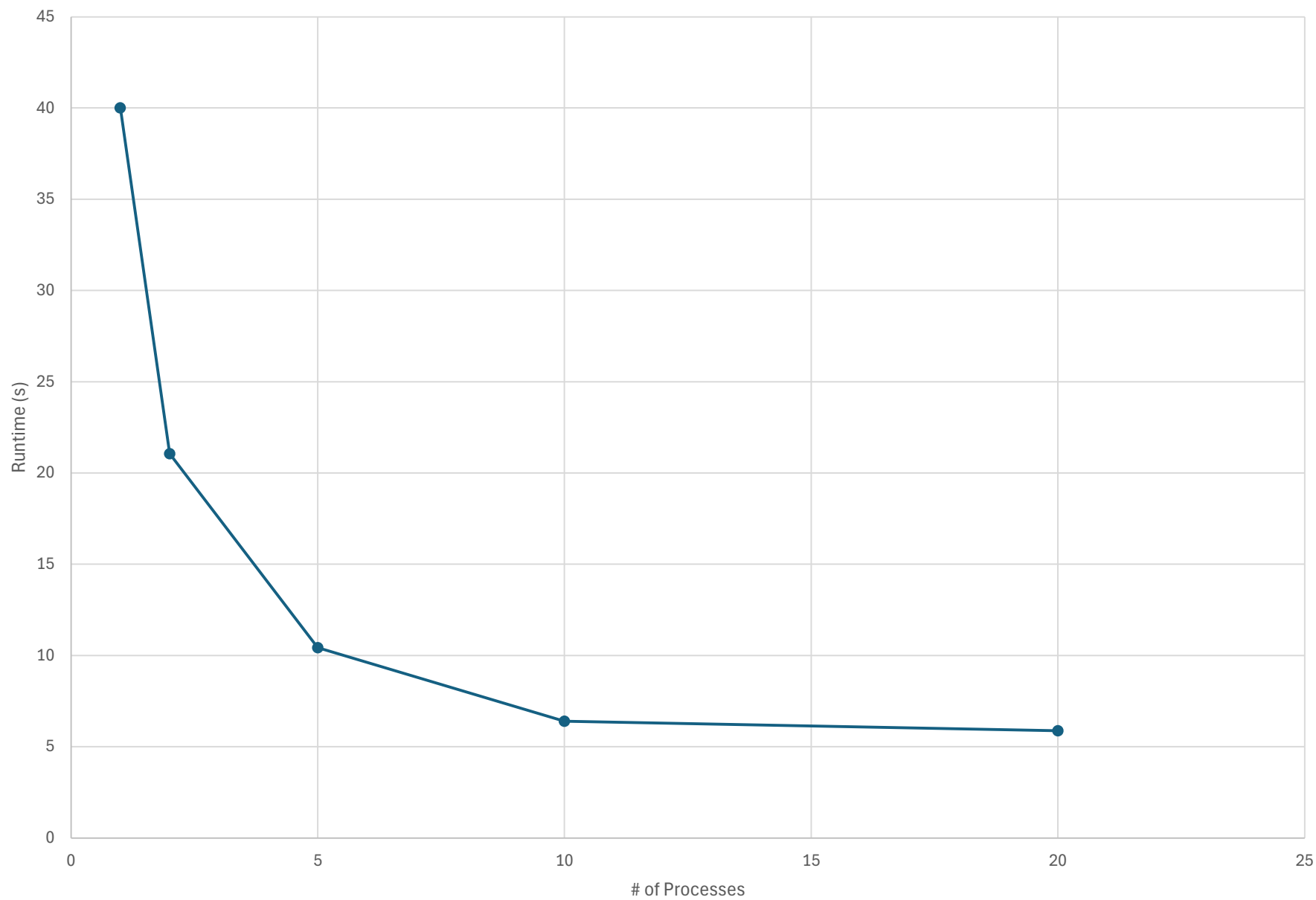
Mandel Image Process Time as a Function of the Number of Processes Allocated
