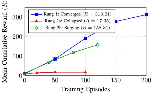
Fig. 4. Mean cumulative episode reward progression. Rung 1 steadily converges to 313.21, Rung 2a suffers catastrophic reward collapse (94.5% reduction), while Rung 2b demonstrates a steep trajectory, achieving 158.31 at episode 120.
