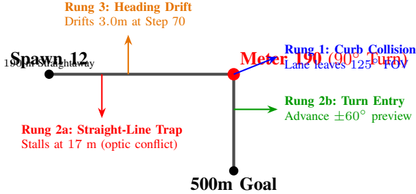
Fig. 6. Trajectory bottleneck map in CARLA Town01. The 90° unbanked right turn at Meter 190 acts as the decisive failure boundary between perceptual configurations.
