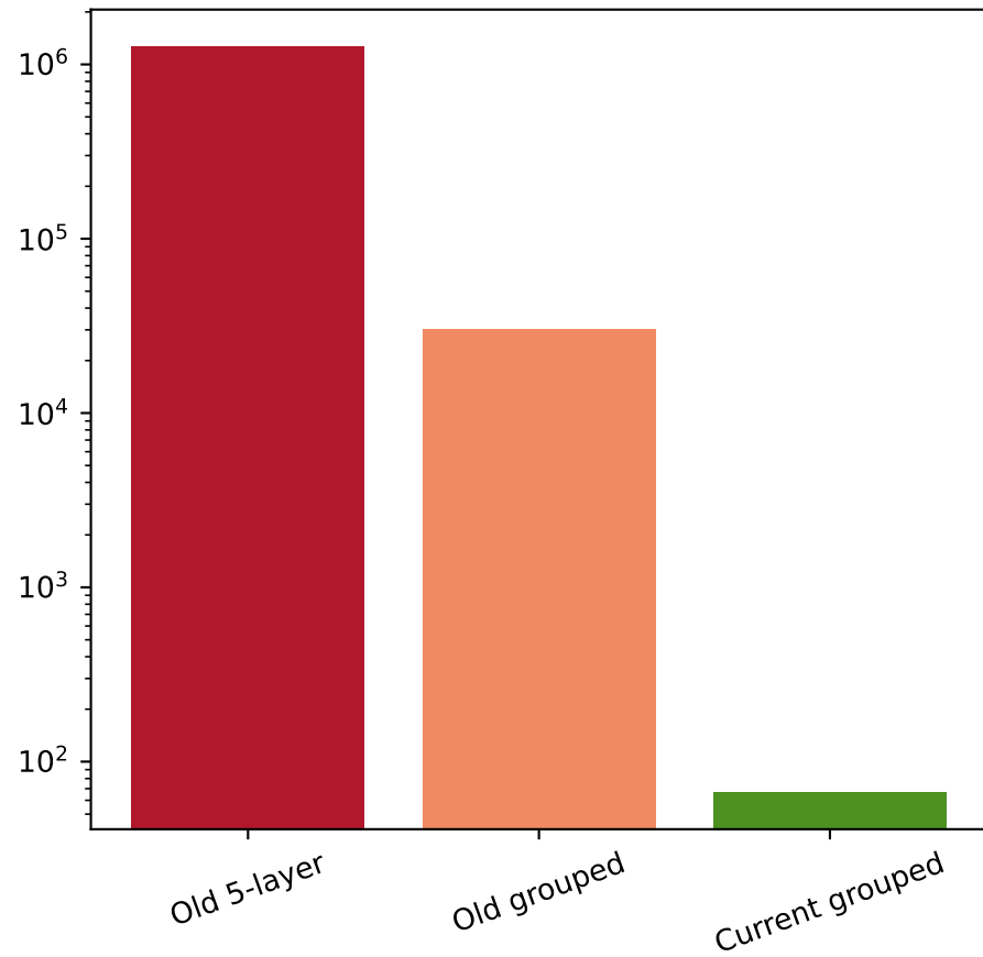
Column-scale spread
