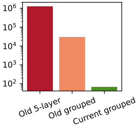
Column-scale spread
