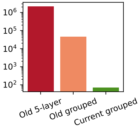
Operator condition number
