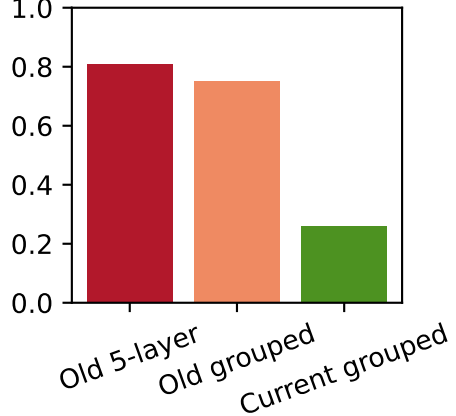
Max off-diagonal |corr|
