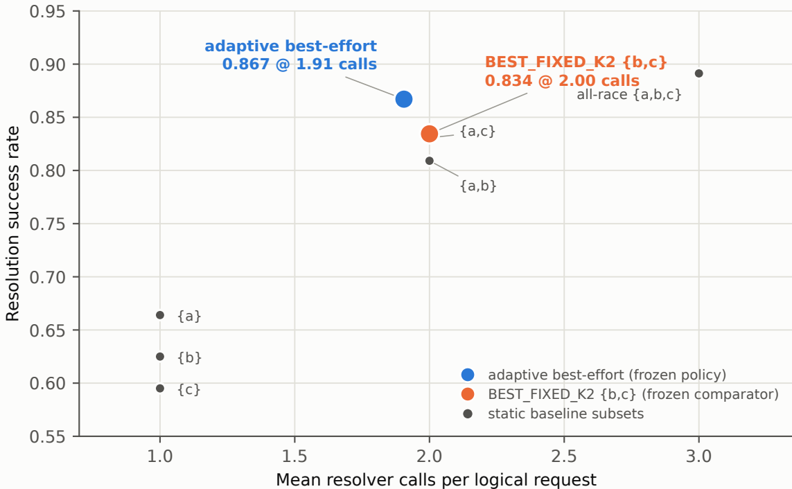
V4 confirmatory: success vs cost (controlled local environment)
