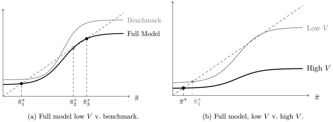
Figure 6: Endogenous effort attenuates the societal feedback sustaining tipping dynamics (Panel (a), Proposition 9). As V increases, this attenuation eliminates the high-bias steady state entirely (Panel (b), Proposition 10)
