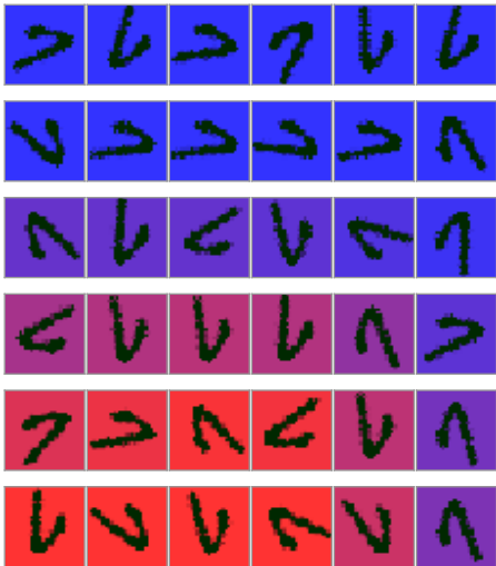
Colour world
