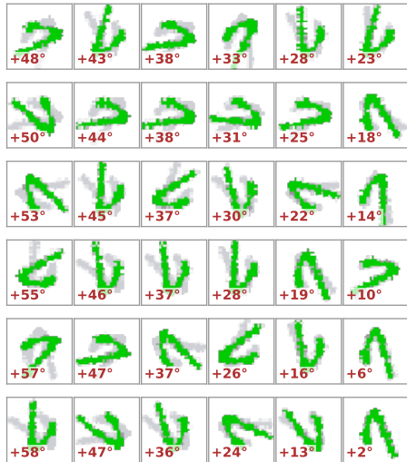
Offset world
