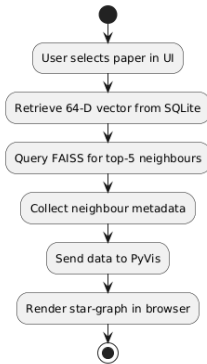
Figure 4: Activity diagram for the runtime query.
