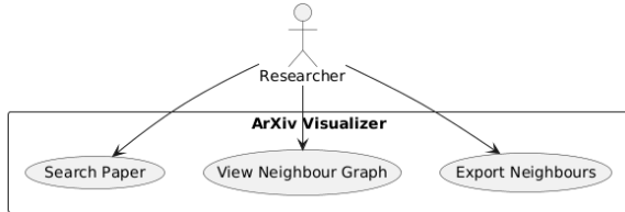
Figure 3: Use-case diagram for the ArXiv Visualizer.
