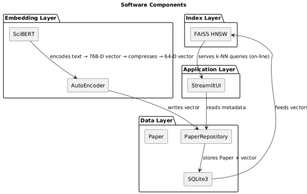
Figure 2: UML Components of the ArXiv Visualizer.
