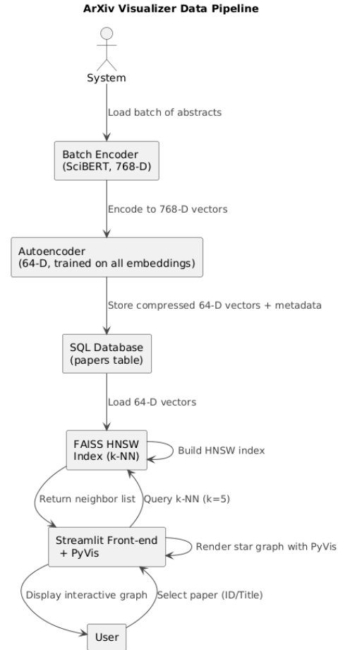
Figure 1: Data-pipeline of the ArXiv Visualizer.
