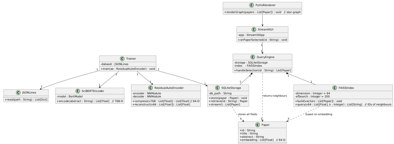
Figure 5: UML Class Diagram of the ArXiv Visualizer.
