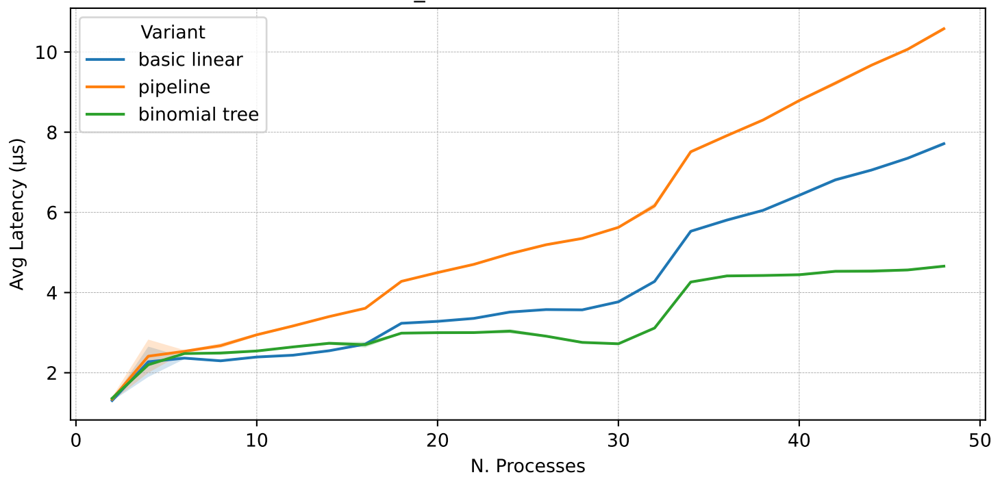
osu_bcast - fixed size 65536 B
