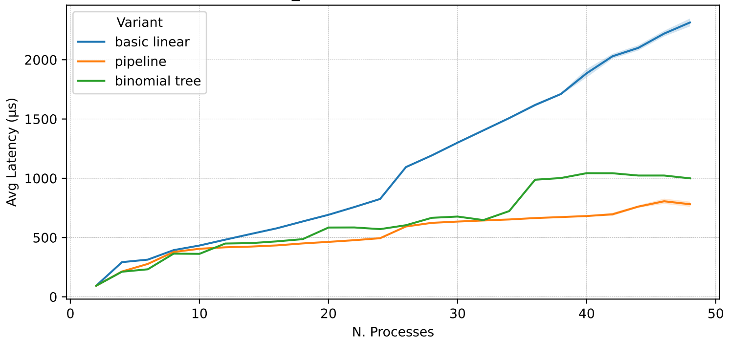
osu_bcast - fixed size 1048576 B
