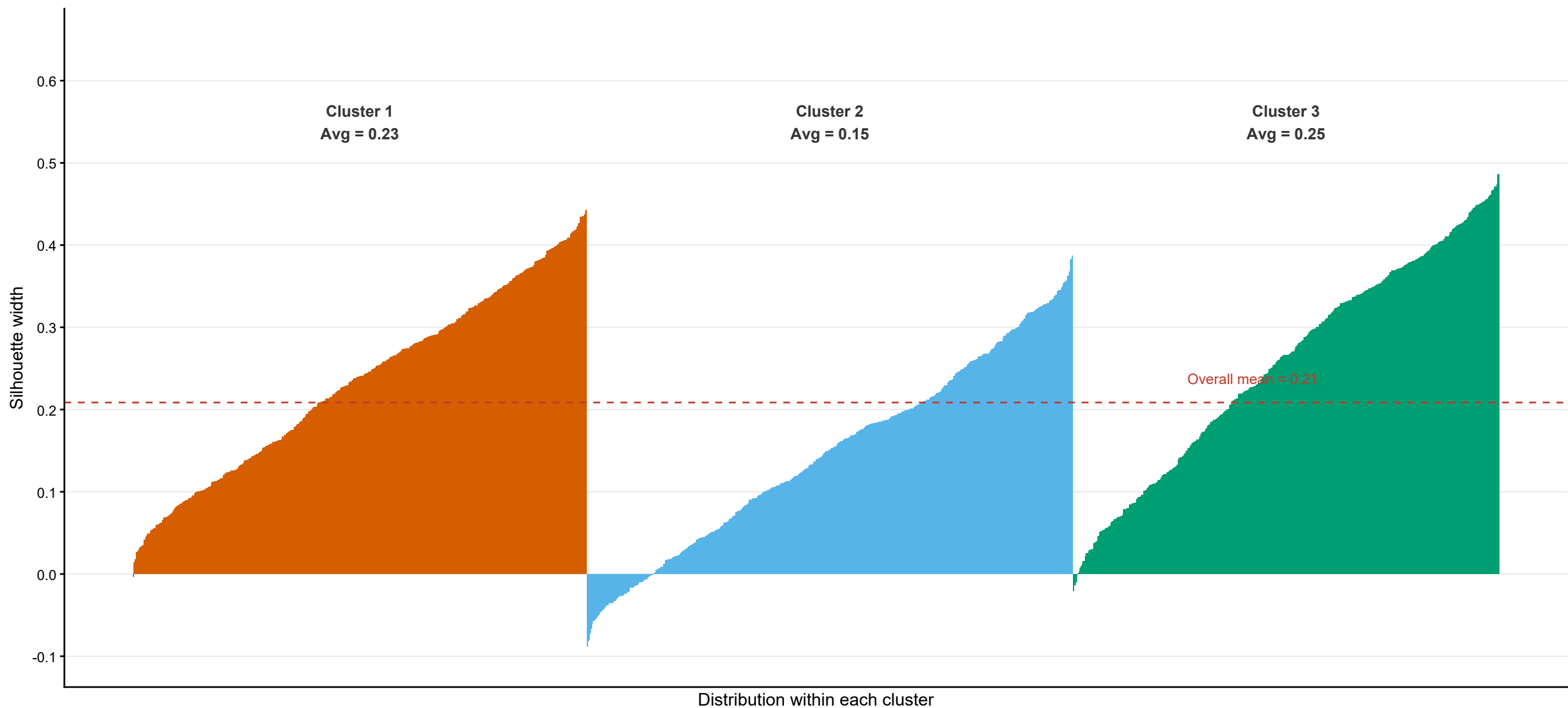
Appendix figure B-1: Silhouette plot for the three cluster solution. Colored profiles show the distribution of silhouette widths within each cluster. Cluster labels indicate the mean silhouette width, and the dashed line the overall mean.
