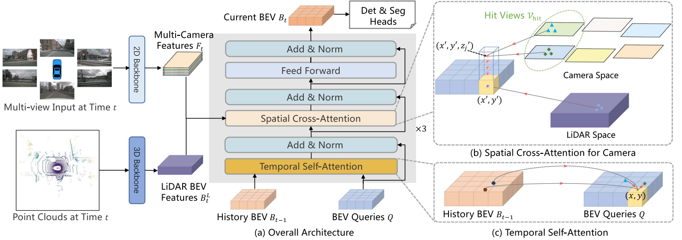
Fig. 3. Overall architecture of BEVFormer. (a) The encoder layer of BEVFormer contains grid-shaped BEV queries, temporal self-attention, and spatial cross-attention. (b) In spatial cross-attention, each BEV query only interacts with spatial features in the regions of interest. (c) In temporal self-attention, each BEV query interacts with two features: the BEV queries at the current timestamp and the BEV features at the previous timestamp.
