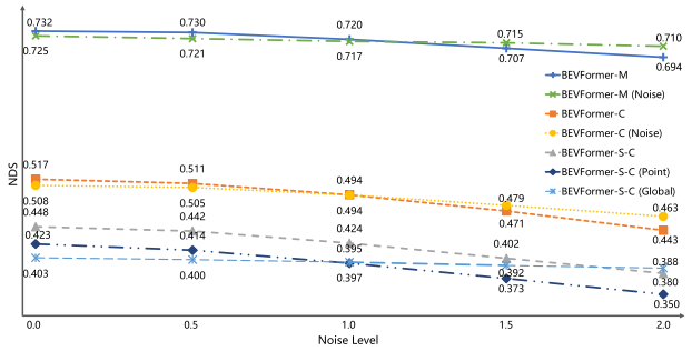
Fig. 9. NDS of methods on nuScenes val set subjected to different levels of camera extrinsics noises. For i th level noises, the rotation noises are sampled from a normal distribution with mean equals 0 and variance equals i (rotation noise are in degrees, and the noise of each axis is independent), and the translation noises are sampled from a normal distribution with mean equals 0 and variance equals 5i (translation noises are in centimeters, and the noise of each direction is independent). “BEVFormer-M” is our default fusion model and “BEVFormer-M (Noise)” is trained with noisy extrinsics under noise level 1. “BEVFormer-C” is our default version for camera-only input. “BEVFormer-C (noise)” is trained with noisy extrinsics (noise level=1). “BEVFormer-S-C” is our static version of BEVFormer-C with the spatial cross-attention implemented by deformable attention [20]. “BEVFormer-S-C (global)” is BEVFormer-S with the spatial cross-attention implemented by global attention (i.e., vanilla multi-head attention) [54]. “BEVFormer-S-C (point)” is BEVFormer-S-C with point spatial cross-attention where we degrade the interaction targets of deformable attention from the local region to the reference points only by removing the predicted offsets and weights.
