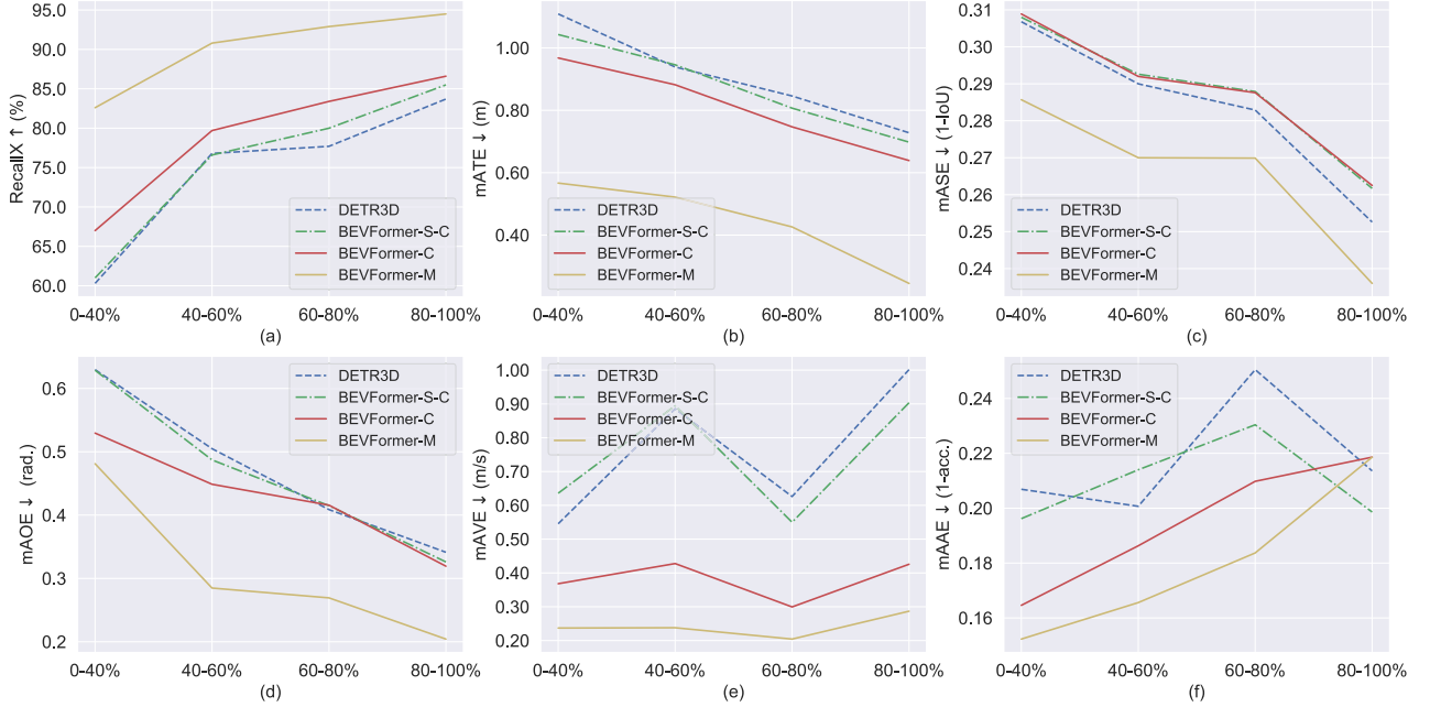
Fig. 6. The detection results of subsets with different visibilities. We divide the nuScenes val set into four subsets based on the visibility that {0-40%, 40-60%, 60-80%, 80-100%} of objects can be visible. (a): Enhanced by the temporal information, BEVFormer-C has a higher recall on all subsets, especially on the subset with the lowest visibility (0-40%) compared to BEVFormer-S-C. The fusion model BEVFormer-M gets much higher recall for occluded objects compared to the vision-only model BEVFormer-C. (b), (d) and (e): For vision-only models, temporal information benefits translation, orientation, and velocity accuracy. We also can observe that the fusion model BEVFormer-M has no obvious advantage in predicting the orientation of occluded objects. (c) and (f): For vision-only models, the scale and attribute error gaps among different methods are minimal. Temporal information does not work to benefit an object's scale prediction.
