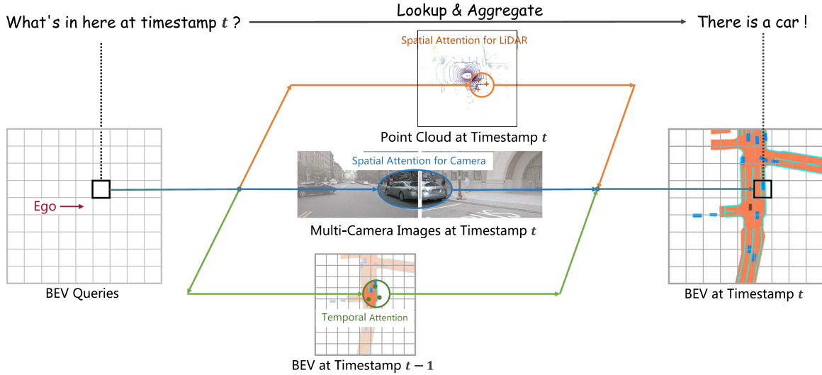
Fig. 1. We propose BEVFormer , a paradigm for autonomous driving that applies both transformer and temporal structures to generate bird's-eye-view (BEV) features from LiDAR-camera inputs. BEVFormer leverages queries to lookup spatial/temporal space and aggregate spatiotemporal information correspondingly, hence benefiting stronger representations for perception tasks.
