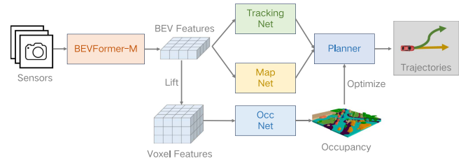
Fig. 5. Architecture of End-to-End Autonomous Driving. Tracking Net and Map Net are query-based networks. After the Planner generates initial prediction results, it utilizes the Occupancy results for optimization to avoid collisions.
