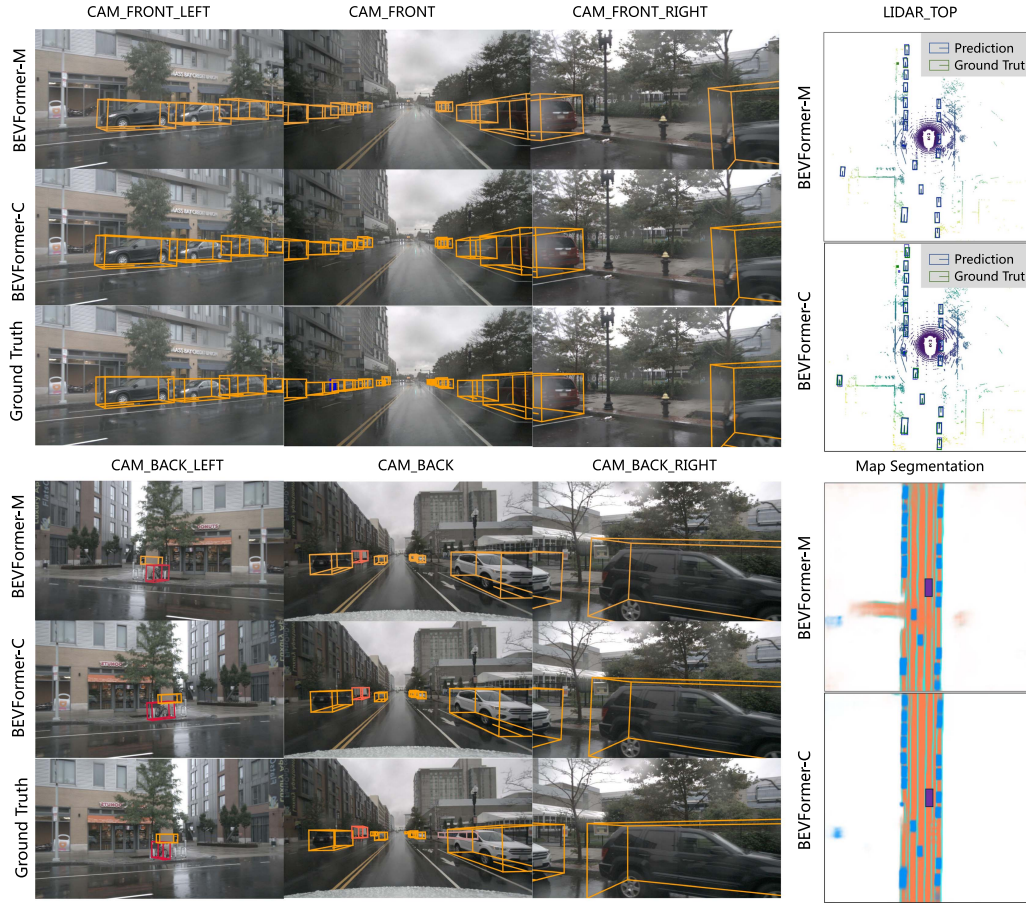
Fig. 8. Visualization results of both object detection and map segmentation tasks. We show vehicle, road, and lane segmentation in blue, orange, and green, respectively.
