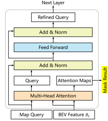
Fig. 4. Segmentation head (mask decoder) of BEVFormer.
