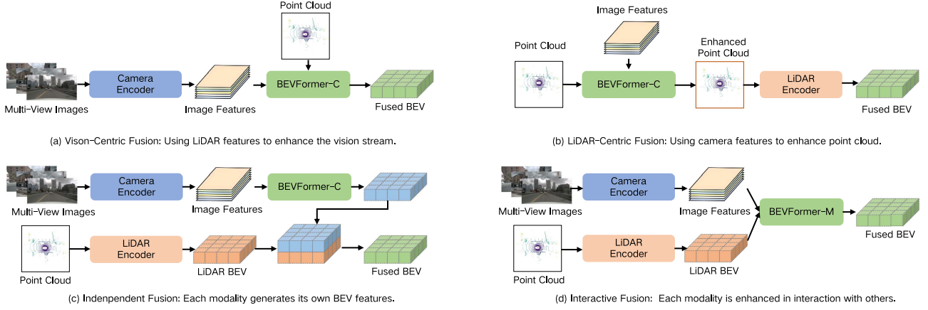
Fig. 2. To extend BEVFormer from a vision-only model in the conference version to a multi-modality model, we designed and compared the performance of various fusion strategies. (a) Version-A: Utilizing LiDAR information to enhance vision-centric BEV generation. In this implementation, We use the point cloud to keep valid 3D sampling points of BEVFormer. (b) Enhancing point cloud features using image information, exemplified by PointPainting [6] and PointAugmenting [11]. For each point cloud, we extract the corresponding image features to serve semantic clues in this implementation. (c) Independently generating BEV features for each modality and then fusing them through simple feature stacking, as demonstrated by BEVFusion-MIT [4] and BEVFusion-PKU [5]. This implementation is basically following BEVFusion-MIT. (d) Our proposed interactive modality fusion approach, where each modality is interlinked and mutually enhances the others, thereby achieving superior performance.
