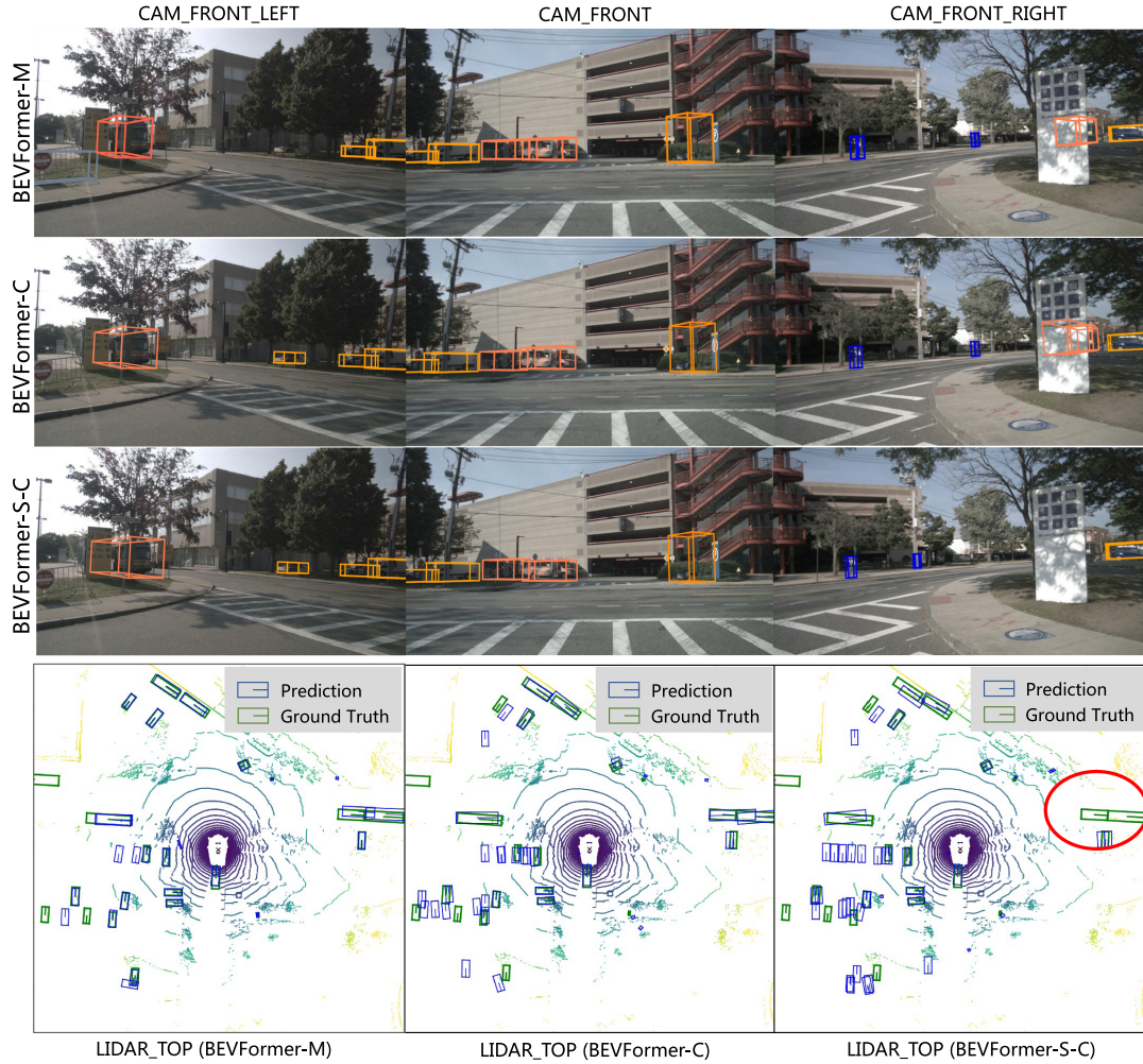
Fig. 7. Comparison of BEVFormer-M, BEVFormer-C and BEVFormer-S-C on nuScenes val set. We can observe that both BEVFormer-M and BEVFormer-C can detect highly occluded objects, and these objects are missed in the prediction results of BEVFormer-S-C (in red circle).
