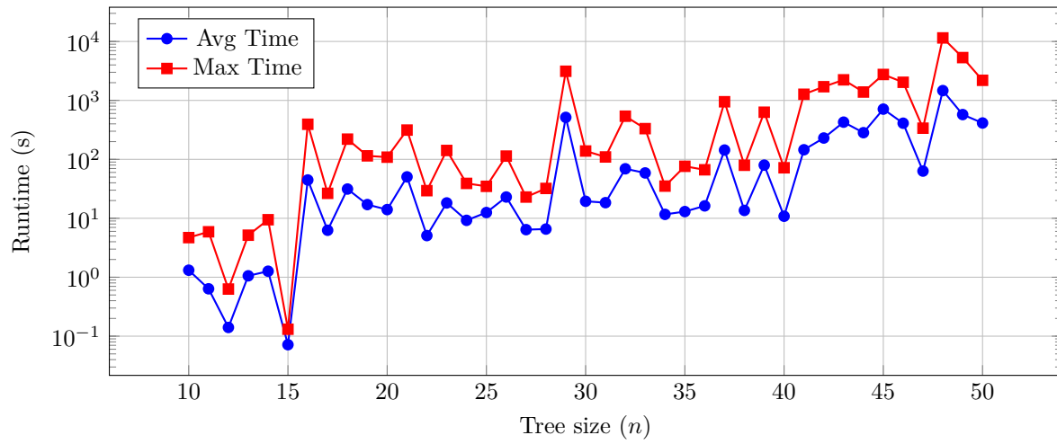
Figure 4.60: Random bounded diameter trees with binomial costs - O(\sqrt{\log n}) -approximation algorithm: runtime
