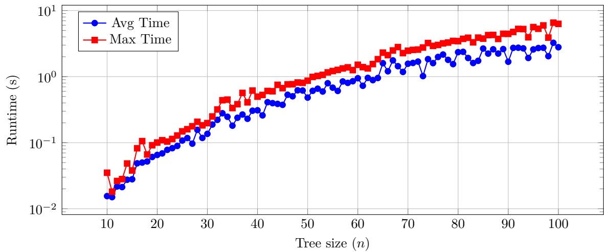
Figure 4.65: Random bounded diameter trees with exponential costs - O(\log n / \log \log n) -approximation algorithm: runtime
