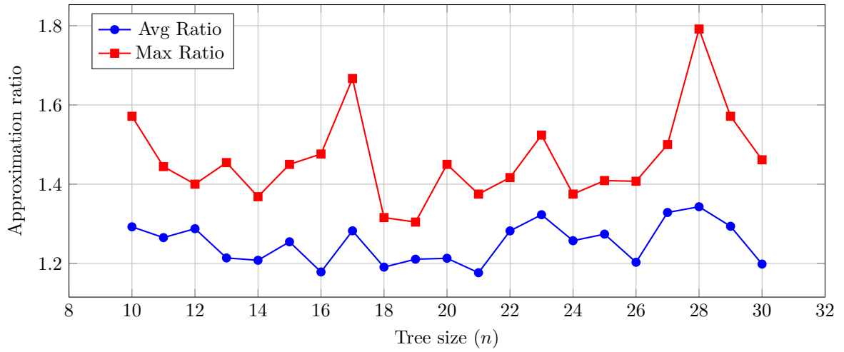
Figure 4.17: Random trees with binomial costs - O(\sqrt{\log n}) -approximation algorithm: approximation quality
