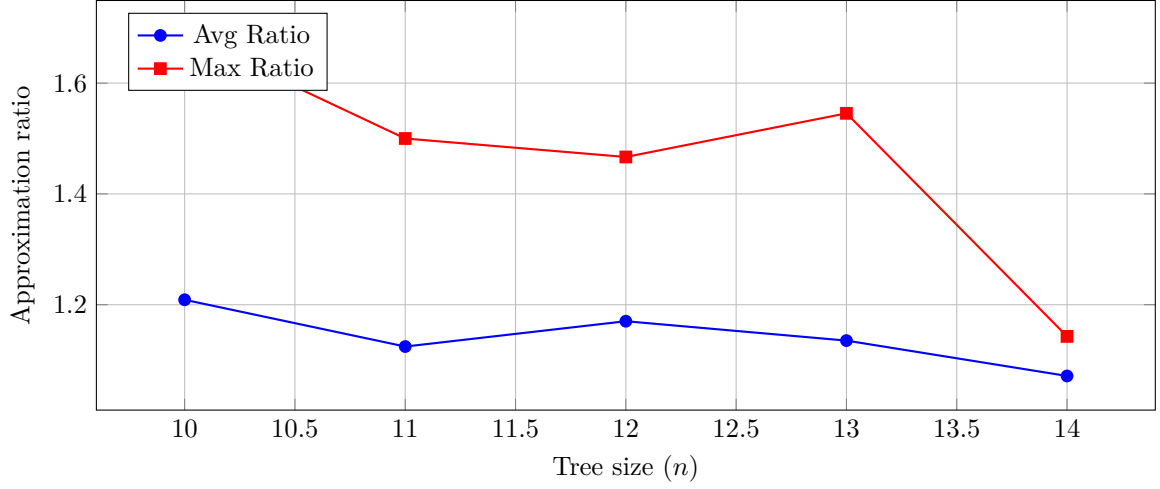
Figure 4.61: Random bounded diameter trees with binomial costs - O(\log \log n) -approximation algorithm: approximation quality
