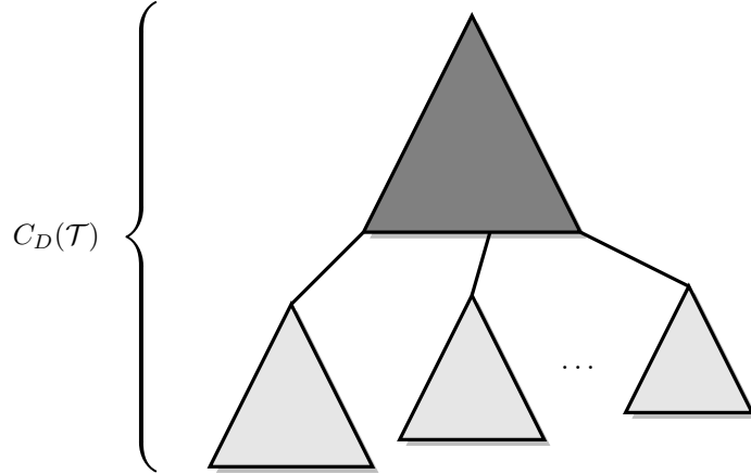
Figure 3.7: The structure of the decision tree D , built by the Algorithm 3. The dark gray subtree represents the decision tree D_{\mathcal{Z}} , obtained by calling the Exact procedure for \mathcal{T}_{\mathcal{Z}} and c . Light gray subtrees represent decision trees D_L , built for each H \in \mathcal{T} - \mathcal{Z} , by recursively calling DECISIONTREE with H and c .
