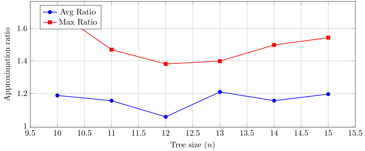
Figure 4.54: Random bounded diameter trees with uniform costs - O(\log \log n) -approximation algorithm: approximation quality
