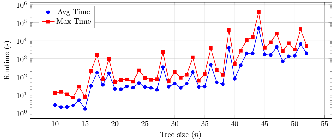
Figure 4.18: Random trees with binomial costs - O(\sqrt{\log n}) -approximation algorithm: runtime
