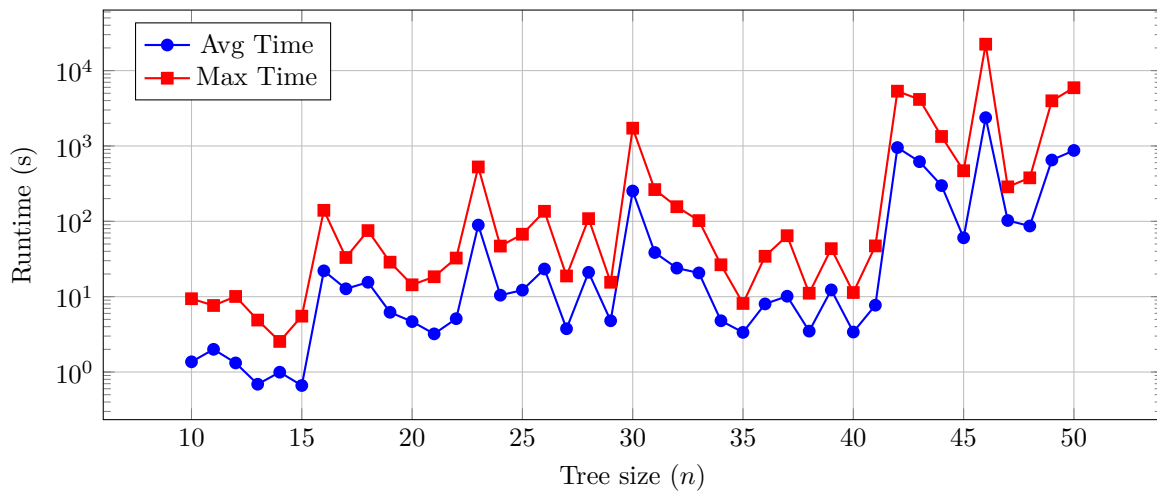
Figure 4.67: Random bounded diameter trees with exponential costs - O(\sqrt{\log n}) -approximation algorithm: runtime
