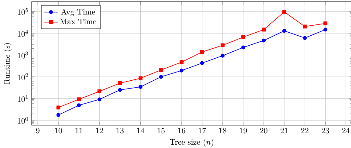
Figure 4.56: Random bounded diameter trees with binomial costs - exact algorithm: runtime comparison
