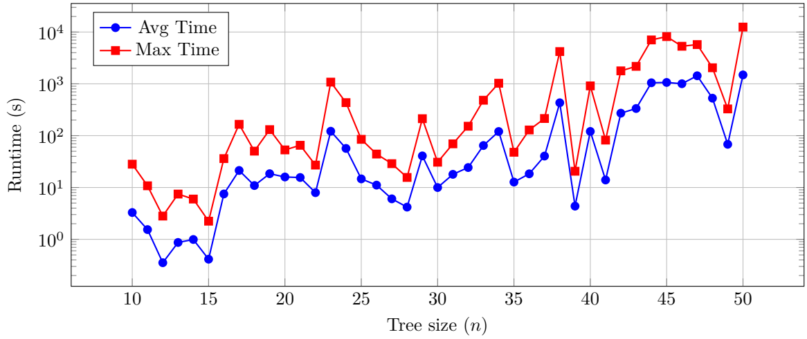
Figure 4.53: Random bounded diameter trees with uniform costs - O(\sqrt{\log n}) -approximation algorithm: runtime
