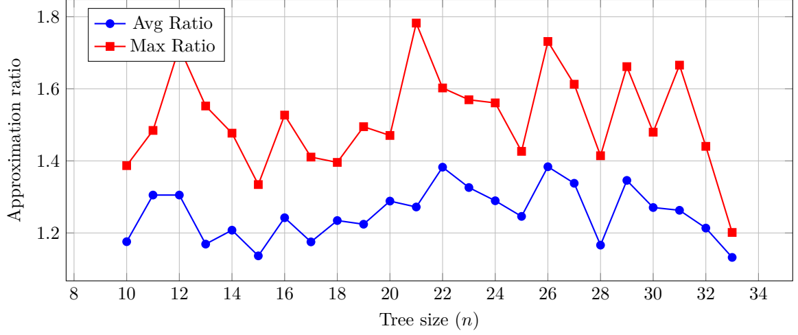
Figure 4.10: Random trees with uniform costs - O(\sqrt{\log n}) -approximation algorithm: approximation quality
