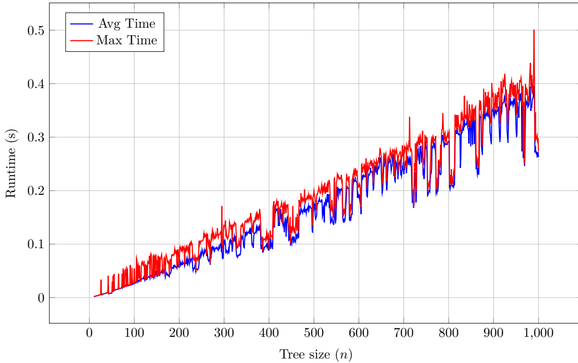
Figure 4.4: Runtime for bounded degree trees (uniform query costs)
