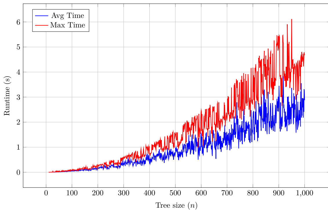
Figure 4.6: Runtime for bounded diameter trees (uniform query costs)
