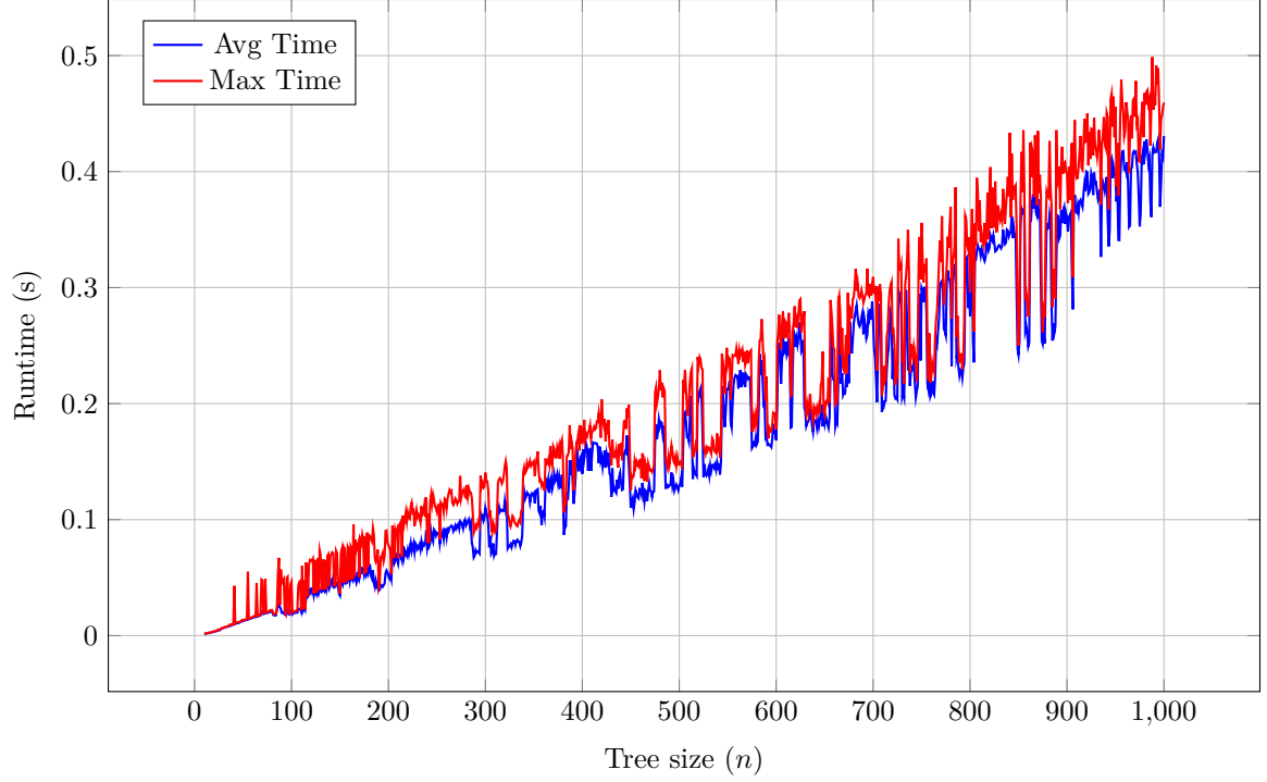
Figure 4.2: Runtime for random trees (uniform query costs)
