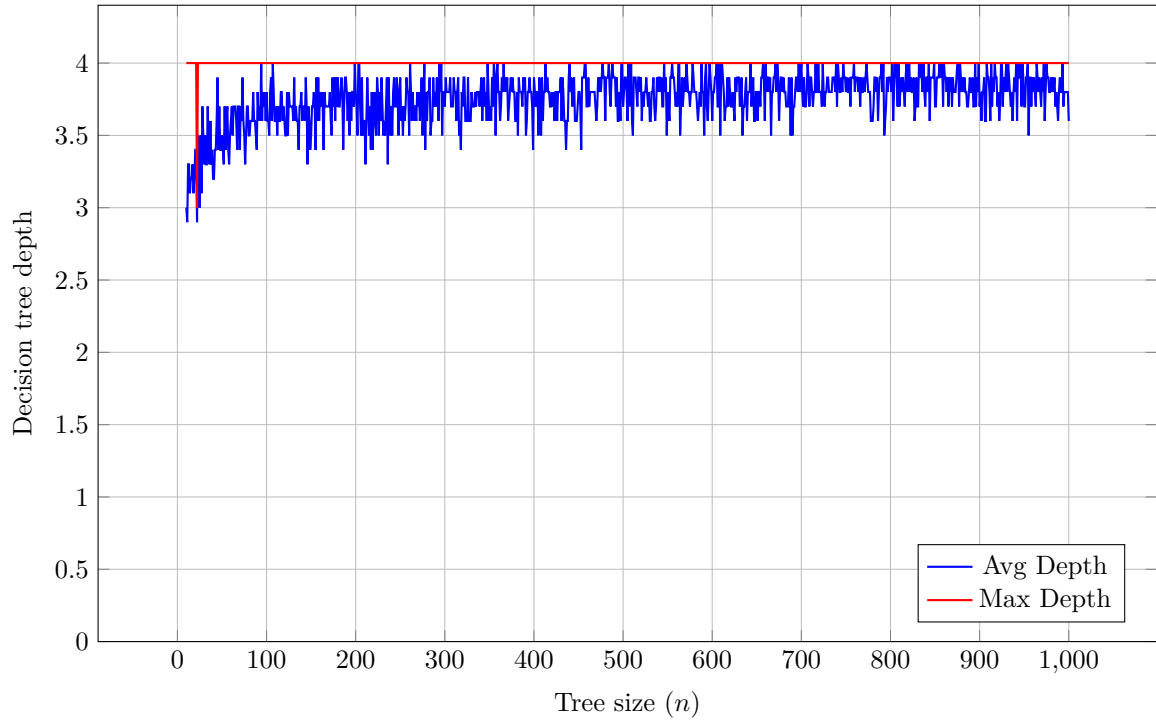
Figure 4.5: Decision tree depth for bounded diameter trees (uniform query costs)
