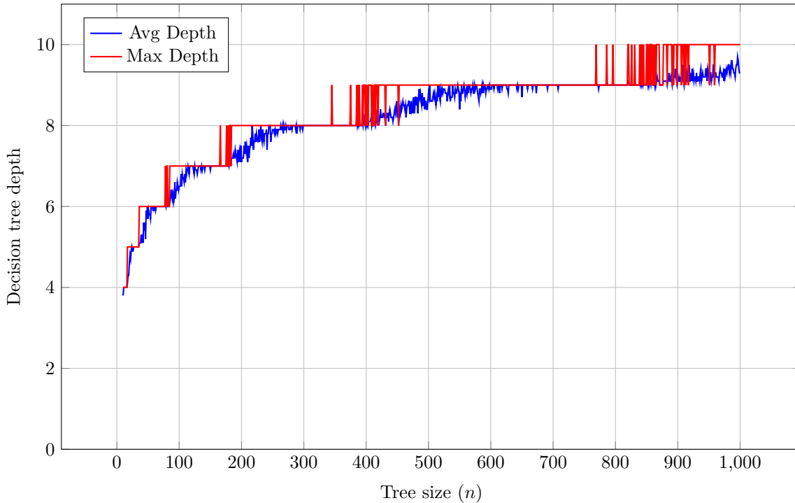
Figure 4.1: Decision tree depth for random trees (uniform query costs)
