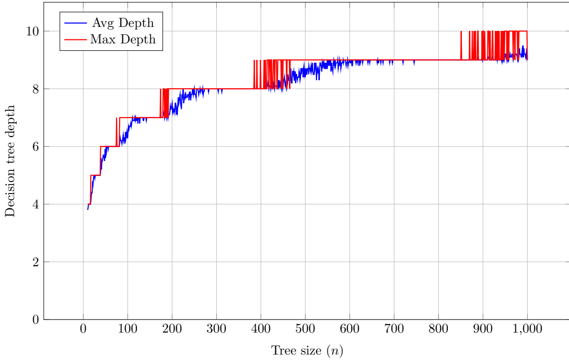
Figure 4.3: Decision tree depth for bounded degree trees (uniform query costs)
