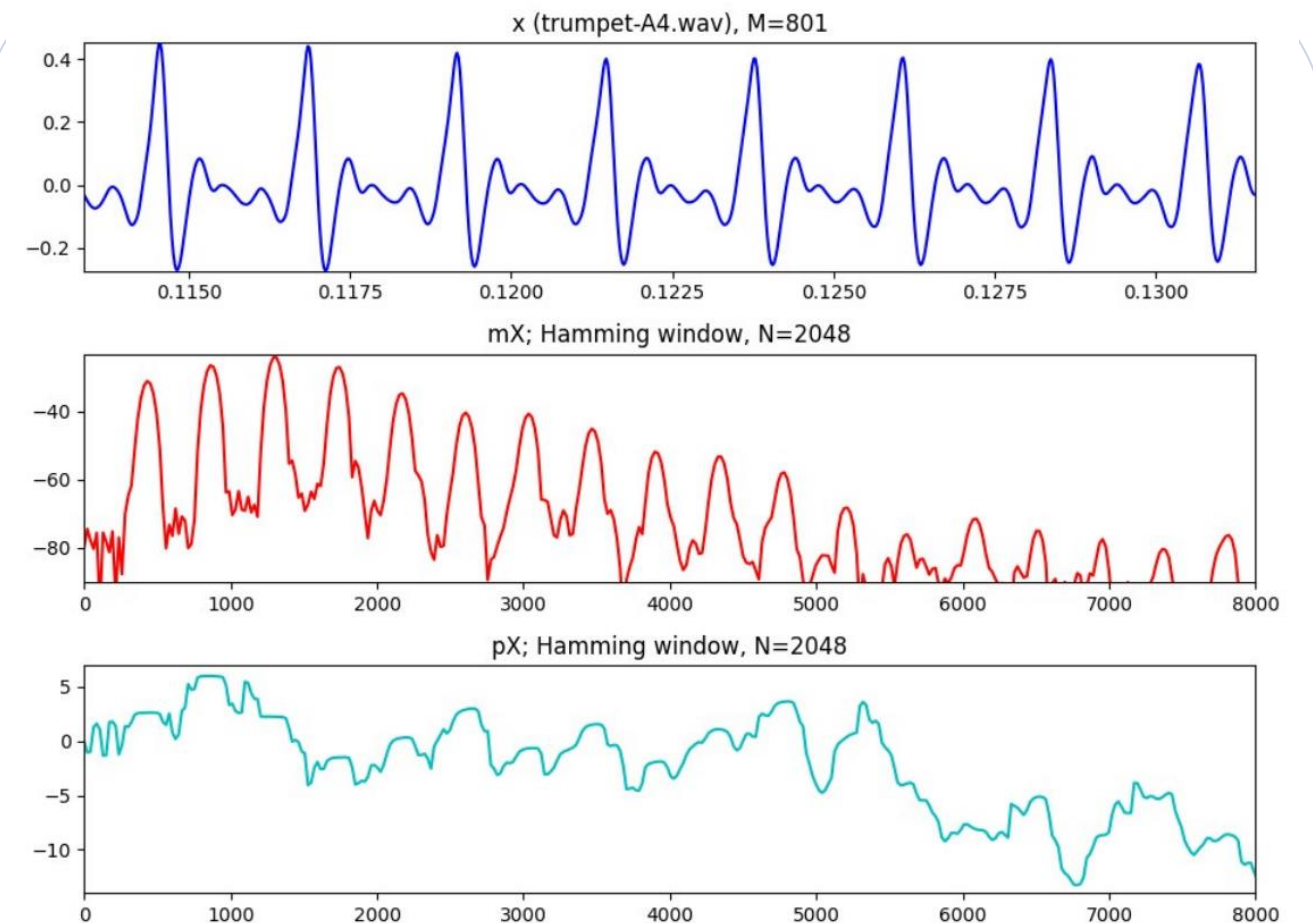
trumpet: spectral peaks and phase
