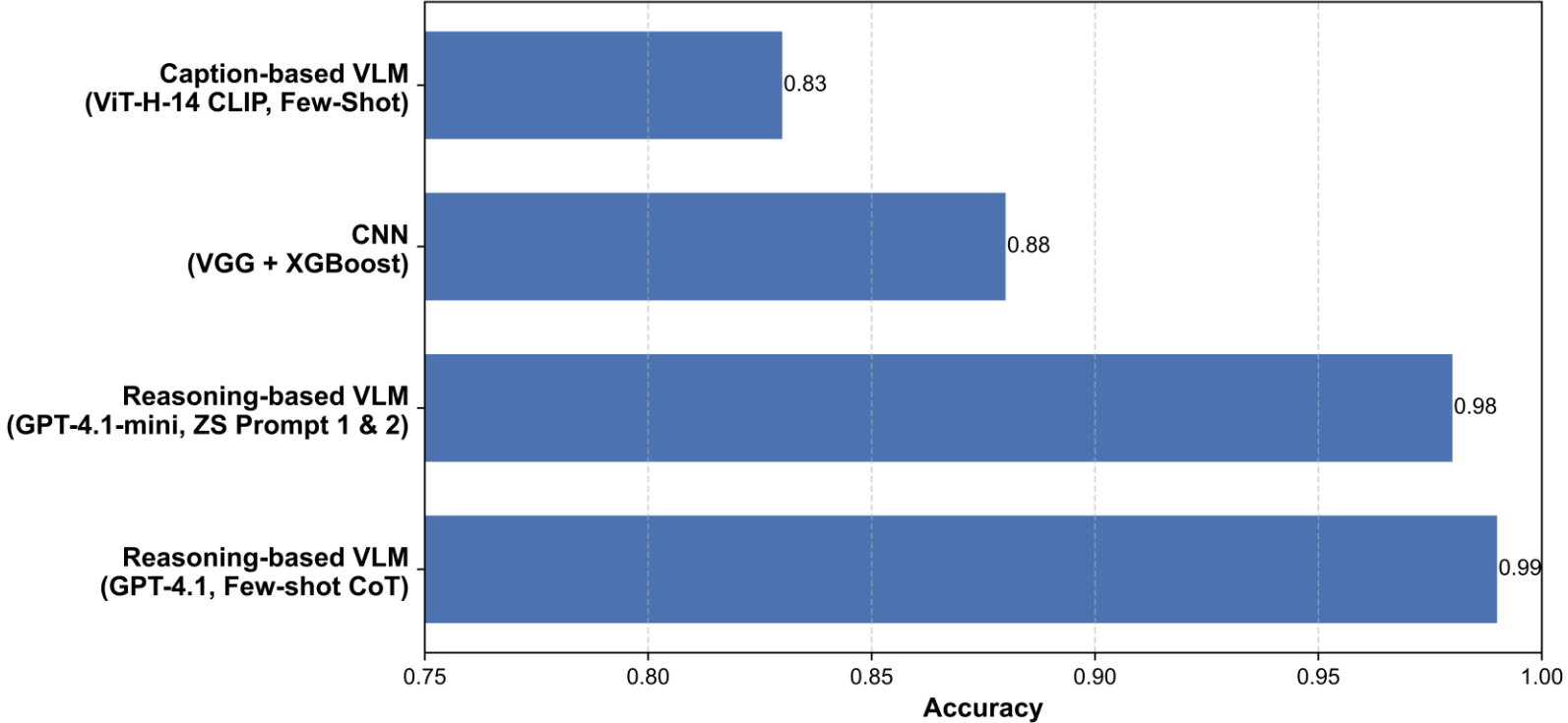
Best Model Performance on Safety Barrier Detection
