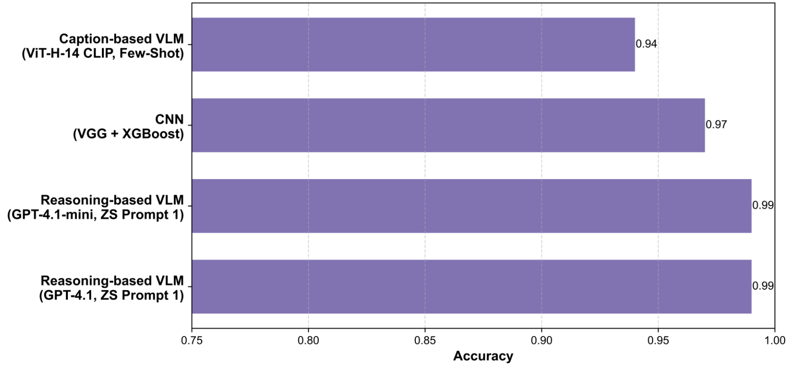
Best Model Performance on Rigid Object Detection
