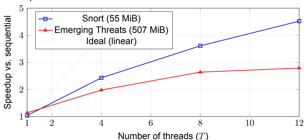
Figure 4: Speedup of text parallelism versus thread count, for a moderate dictionary (Snort, 55 MiB) and a memory-bound dictionary (Emerging Threats, 507 MiB), on the \sim 10.6 GiB corpus.
