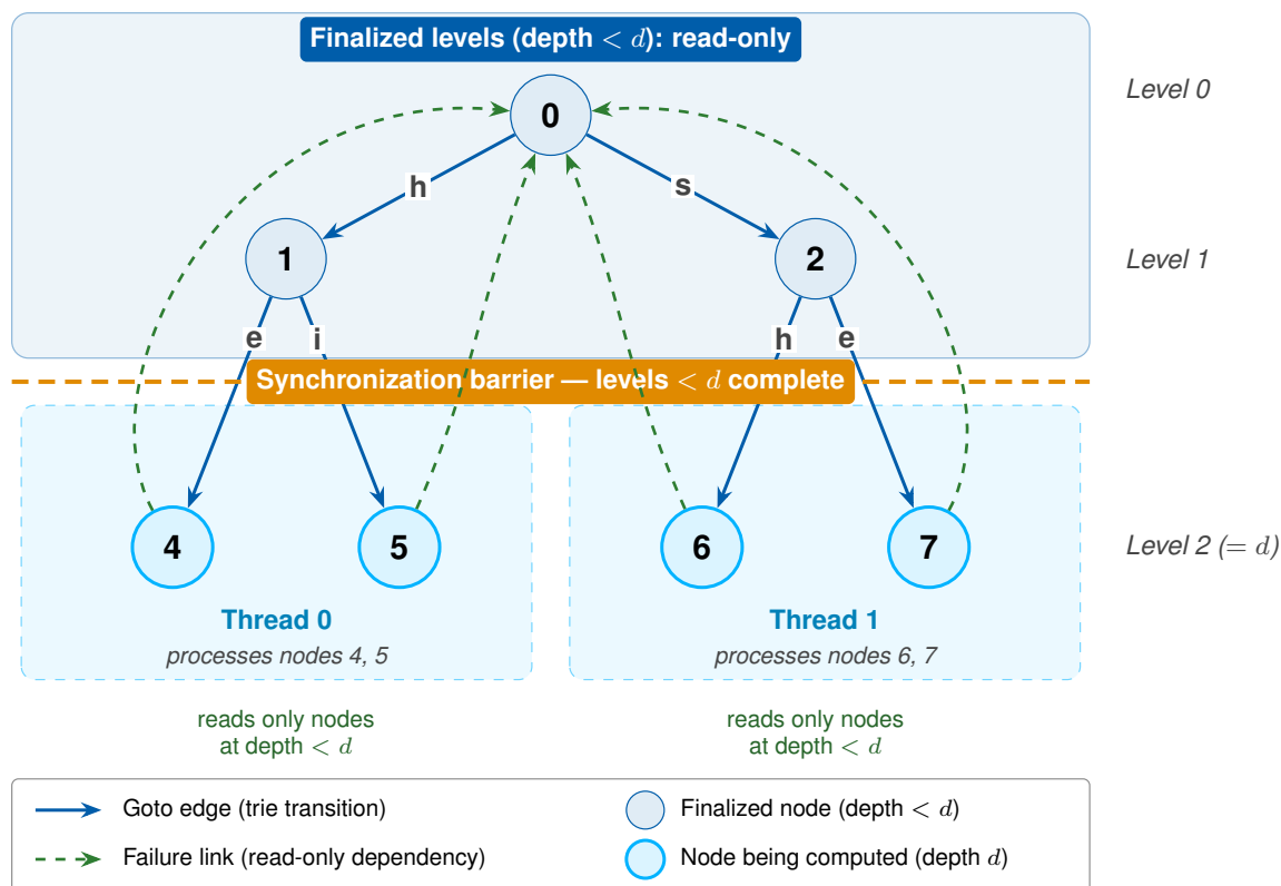
Figure 11: Level-synchronous parallel construction of the failure function. Threads compute the failure links of all states at one BFS level in parallel, reading only already-finalized links from shallower levels (green), and meet at a barrier before advancing to the next level.
