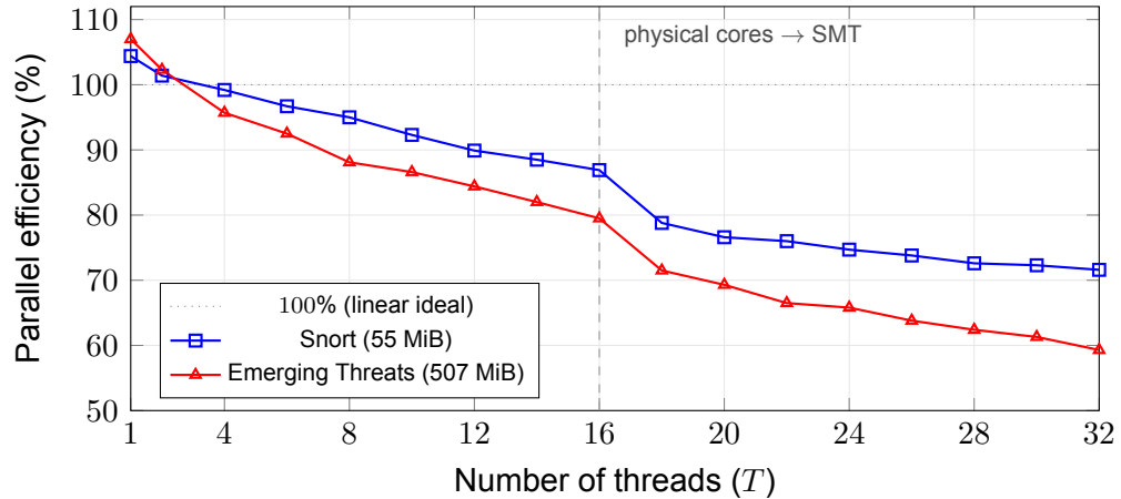
Figure 14: Parallel efficiency—speedup divided by thread count (Eq. 4)—for the winning strategy ( pthread_dynamic_flat ) on the canonical Enron corpus, restating the curves of Figure 13. While the speedup itself rises monotonically to T = 32 , the efficiency view exposes the saturation of the parallel gain: each added thread contributes less, and the largest single loss occurs when the sweep crosses the dashed line at sixteen threads and the first SMT siblings begin to share physical cores. The memory-bound dictionary runs eight to twelve percentage points below the moderate one throughout, consistent with the memory-bandwidth contention discussed above. Values marginally above 100% at one and two threads reflect the flat emission layout of the measured searcher, which is slightly faster than the chained sequential baseline used as the reference (Table 8).
