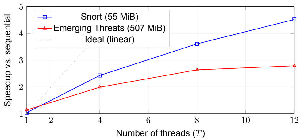
Figure 4: Speedup of text parallelism versus thread count, for a moderate dictionary (Snort, 55 MiB) and a memory-bound dictionary (Emerging Threats, 507 MiB), on the \sim 10.6 GiB corpus.
