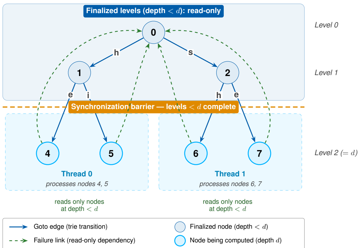
Figure 9: Level-synchronous parallel construction of the failure function. Threads compute the failure links of all states at one breadth-first level in parallel, reading only already-finalized links from shallower levels (green), and meet at a barrier before advancing to the next level.
