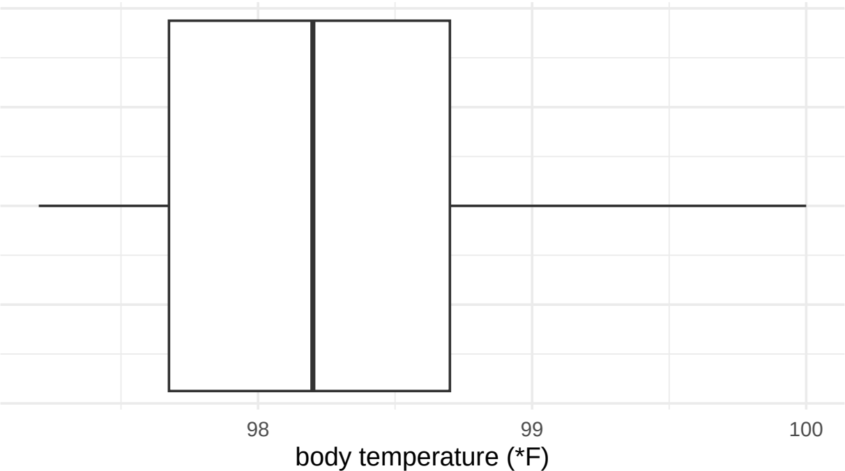
Boxplot of Body Temperatures for Stat 216 Students
