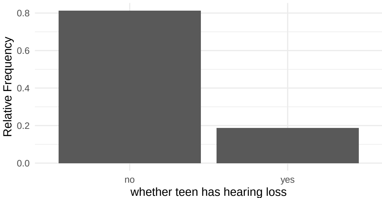
Relative Frequency Bar Plot of Hearing Loss Status for US Teens
