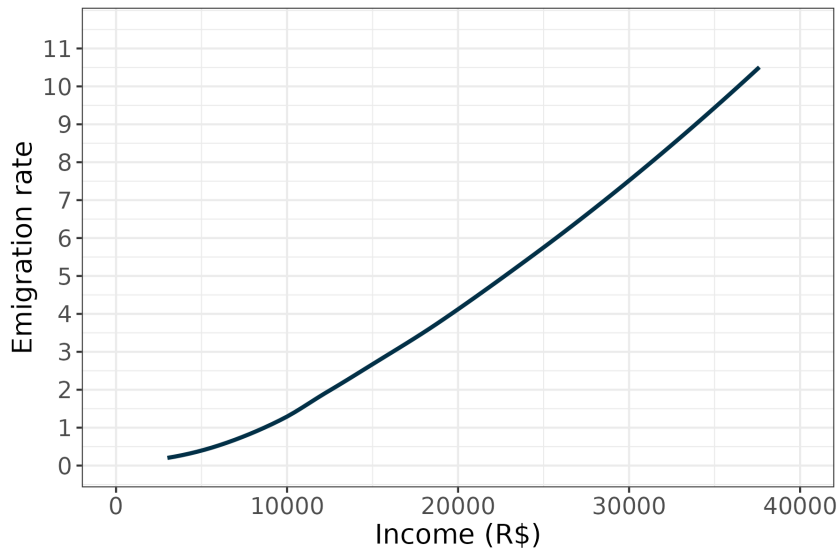
FIGURE D.7 Migration probabilities by income (model)
