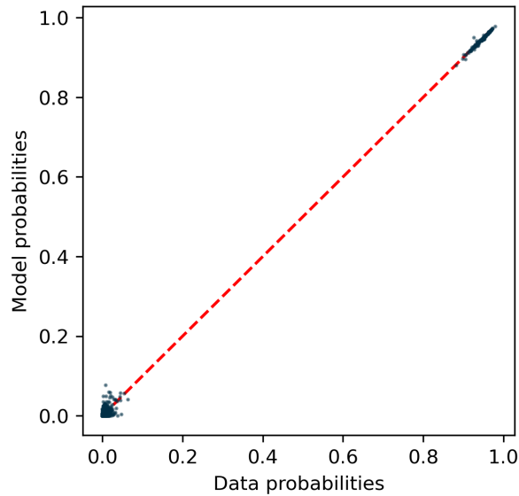
FIGURE D.6 Migration probabilities: Model vs. data
