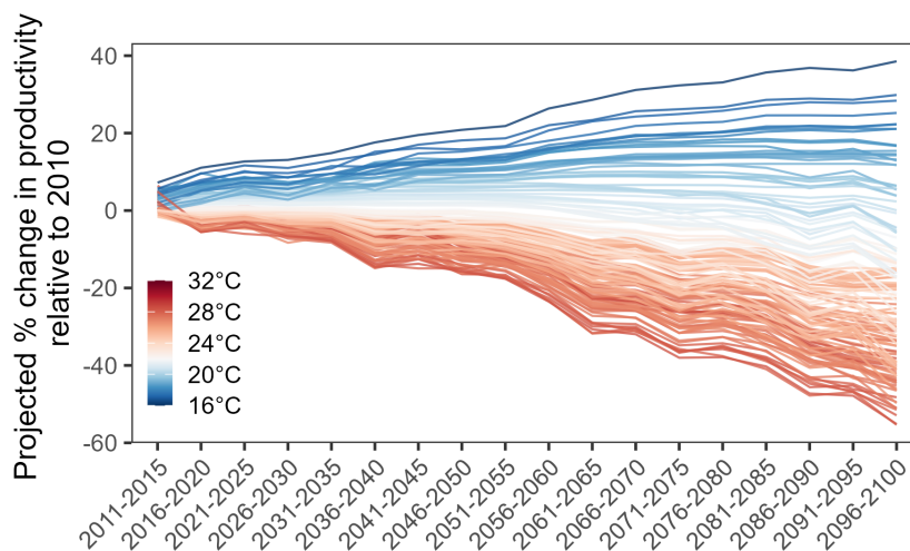
FIGURE D.5 Counterfactual agricultural productivity paths
