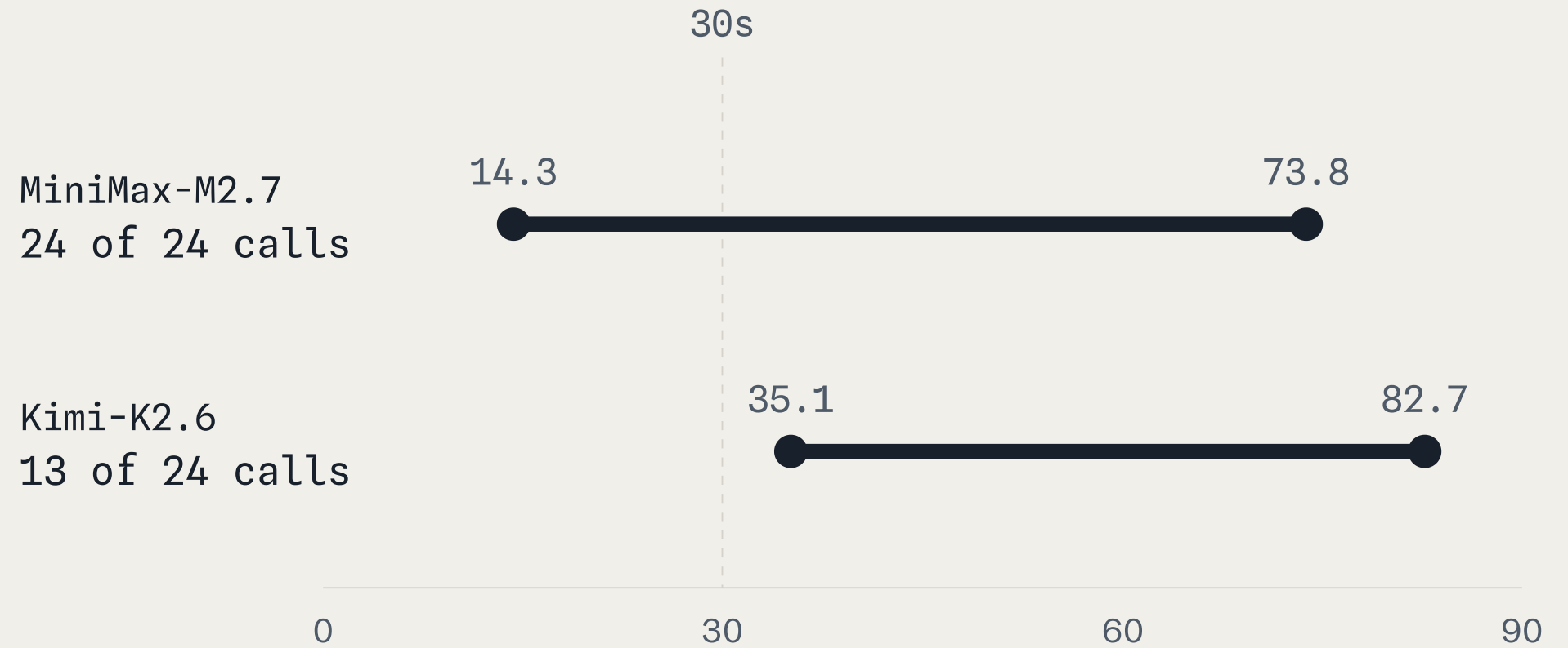
SECONDS TO A COMPLETED CALL, 3 SEP BENCHMARK
