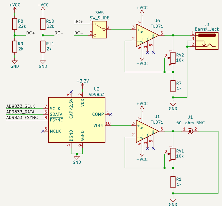
Signal Generation & Amplification
