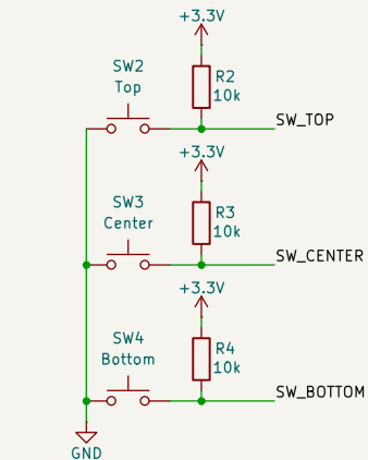
Pushbuttons
