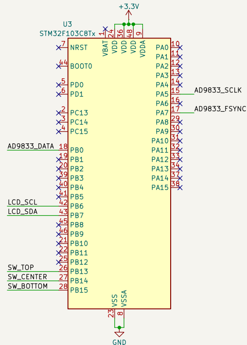
Microcontroller
