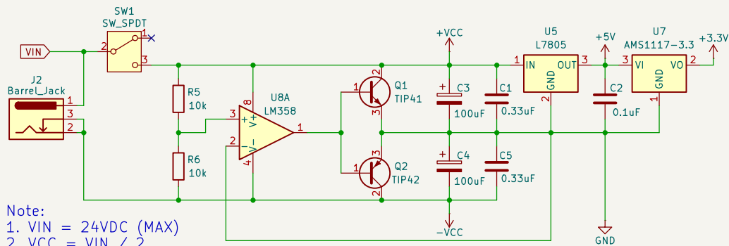
Power Section (Rail Splitter)
