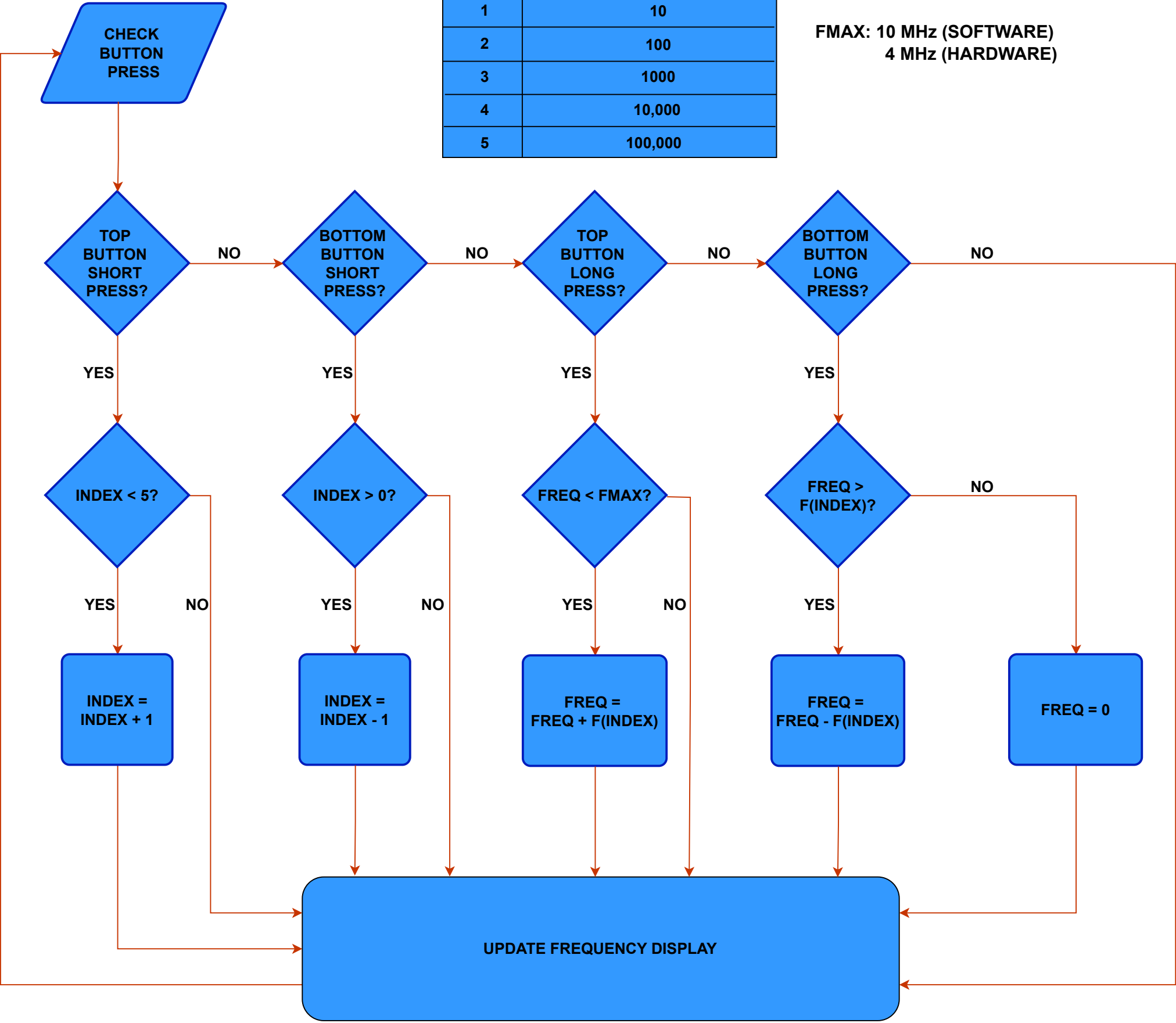
FLOWCHART FOR FREQUENCY SELECTION LOGIC
