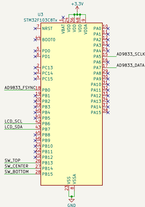
Microcontroller
