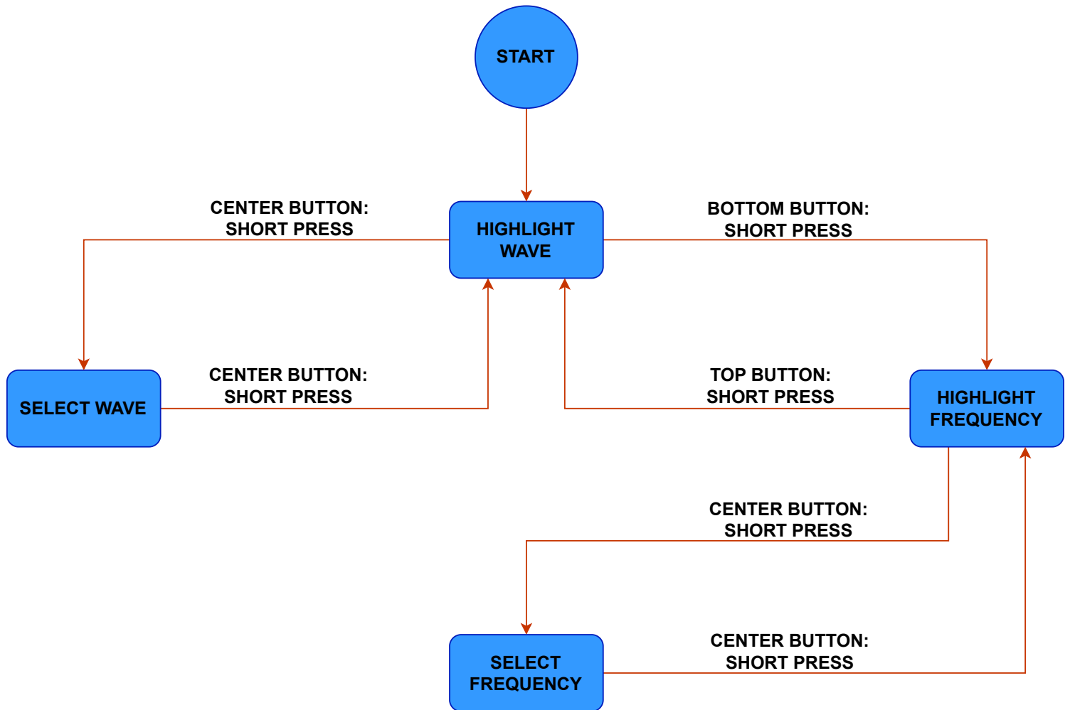
STATE DIAGRAM FOR USER INTERFACE
