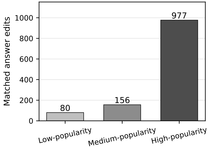
Python
