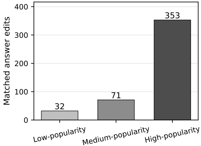
JavaScript
