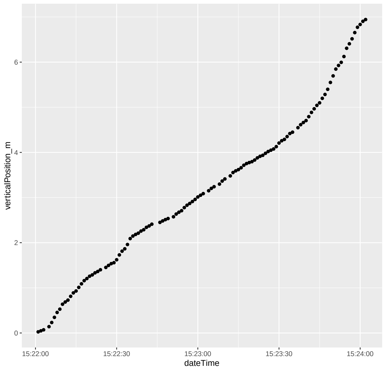
270_2026_06_22_Level1.csv ****Depth vs. time
