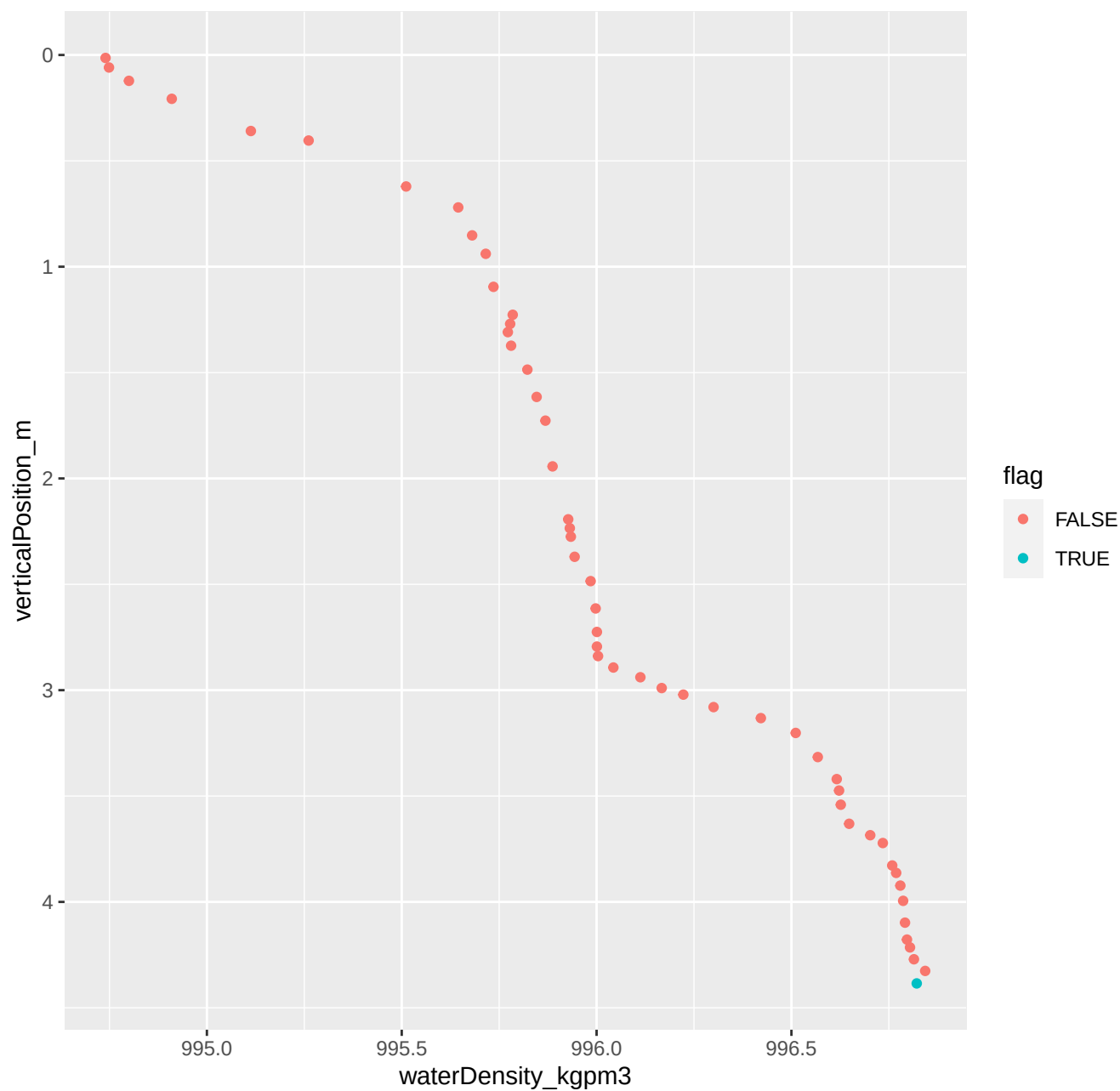
091_2026_07_06_Level1.csv ****Non-monotonic densities
