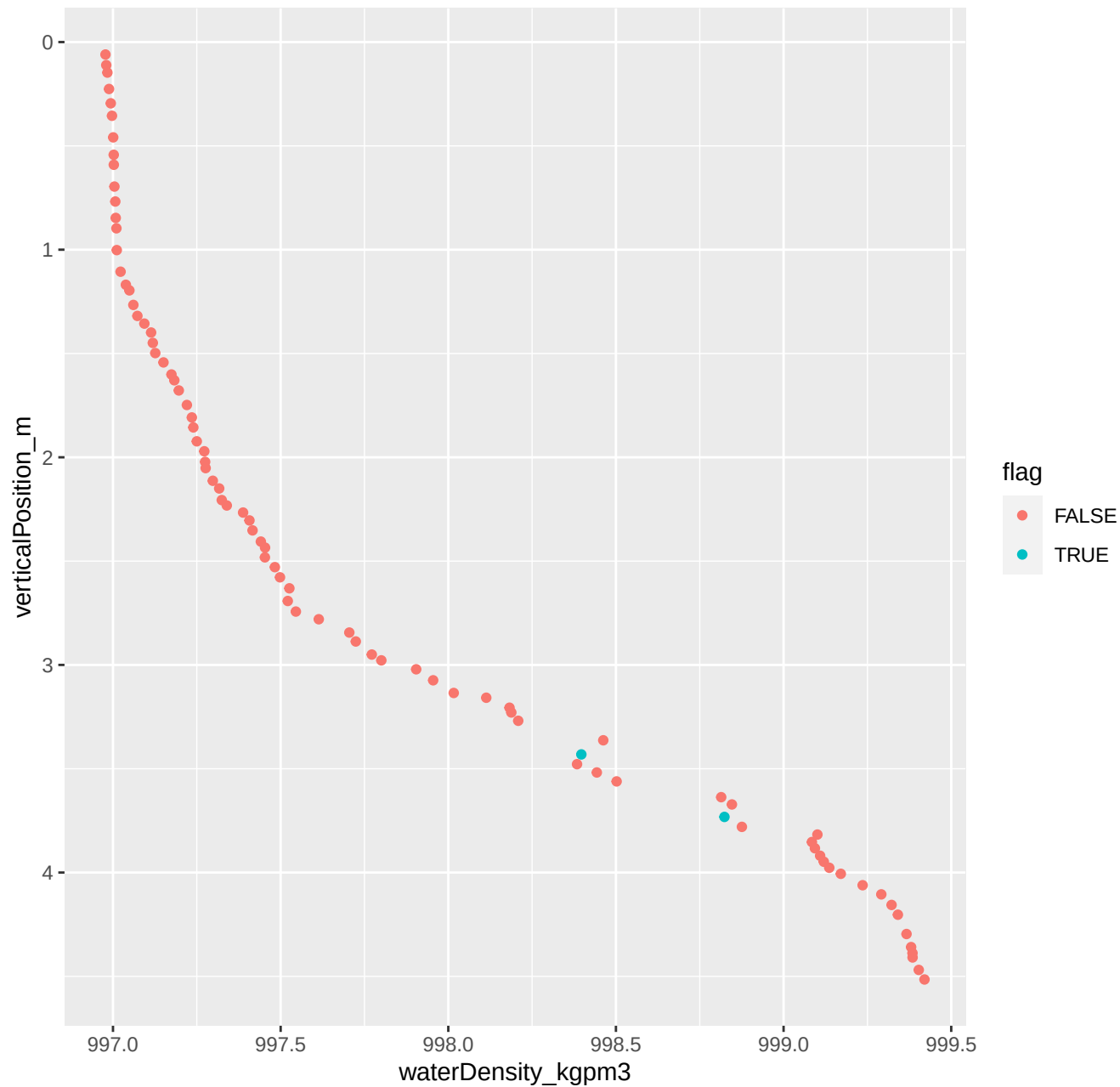
440_2026_08_06_Level1.csv ****Non-monotonic densities
