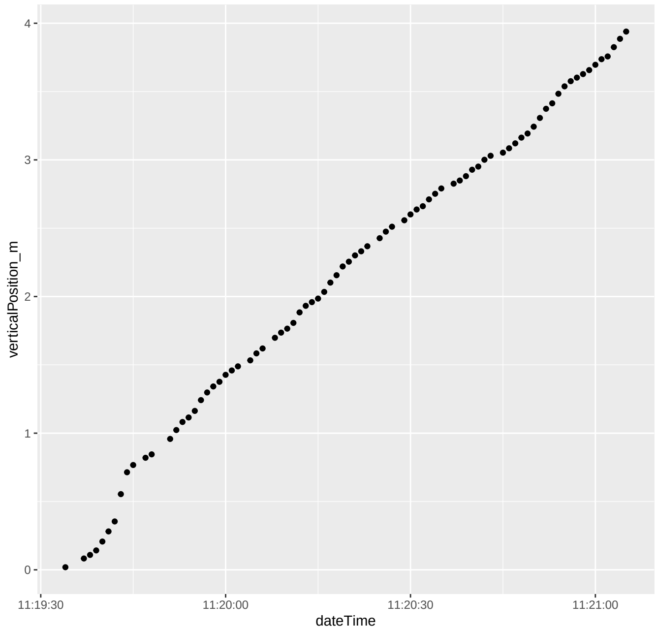
183_2026_06_16_Level1.csv ****Depth vs. time
