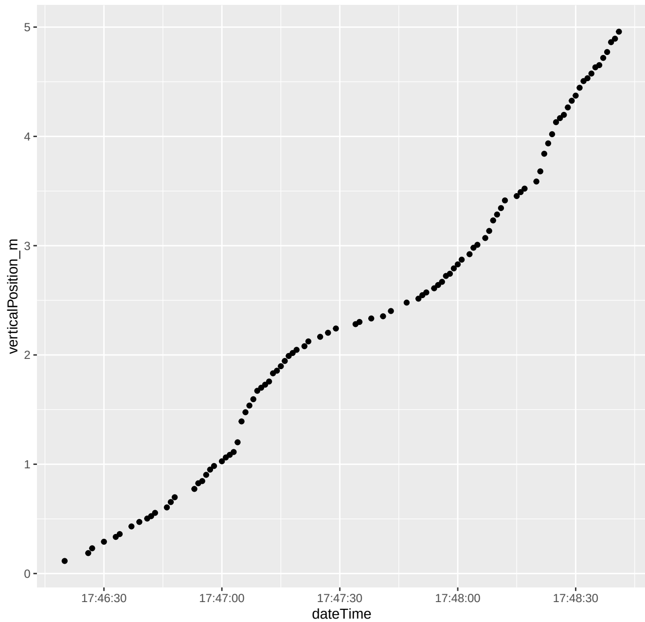
024_2026_06_02_Level1.csv ****Depth vs. time
