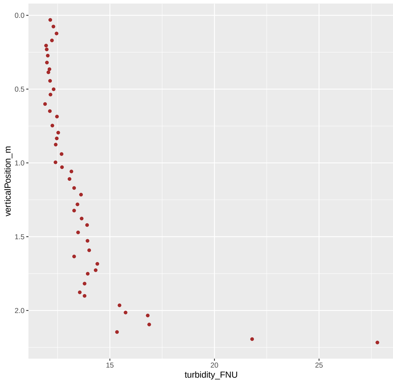
163_2023_05_22_Level1.csv ****Turbidity jumps
