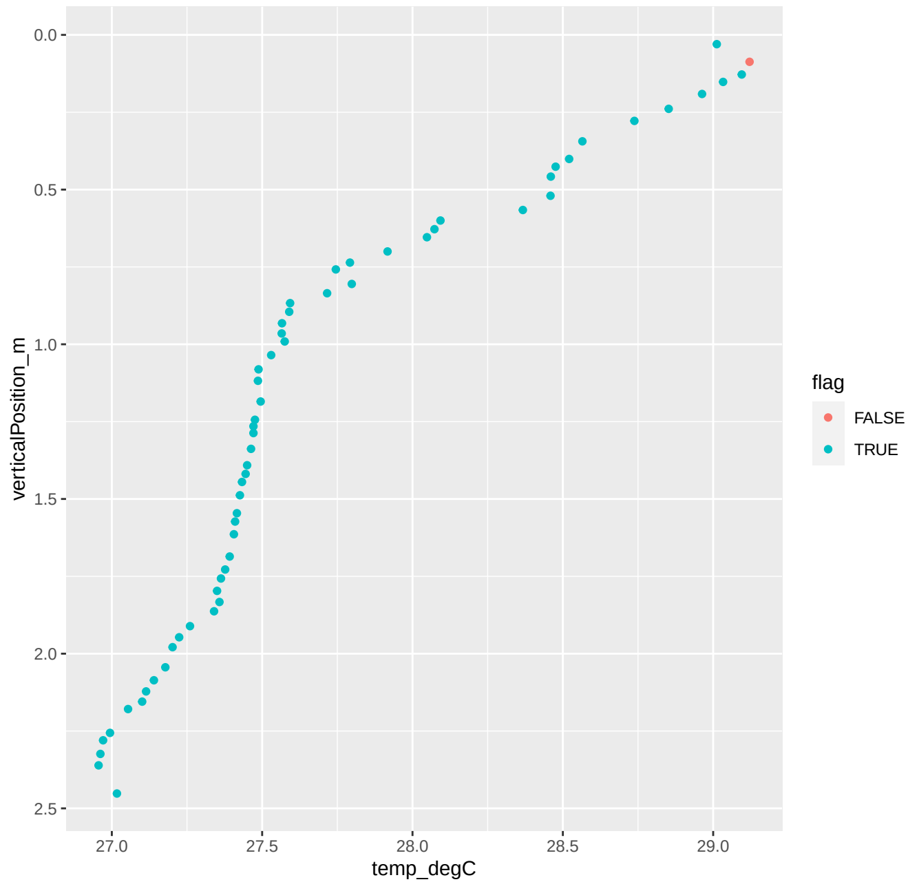
165_2023_08_09_Level1.csv ****Non-decreasing temps
