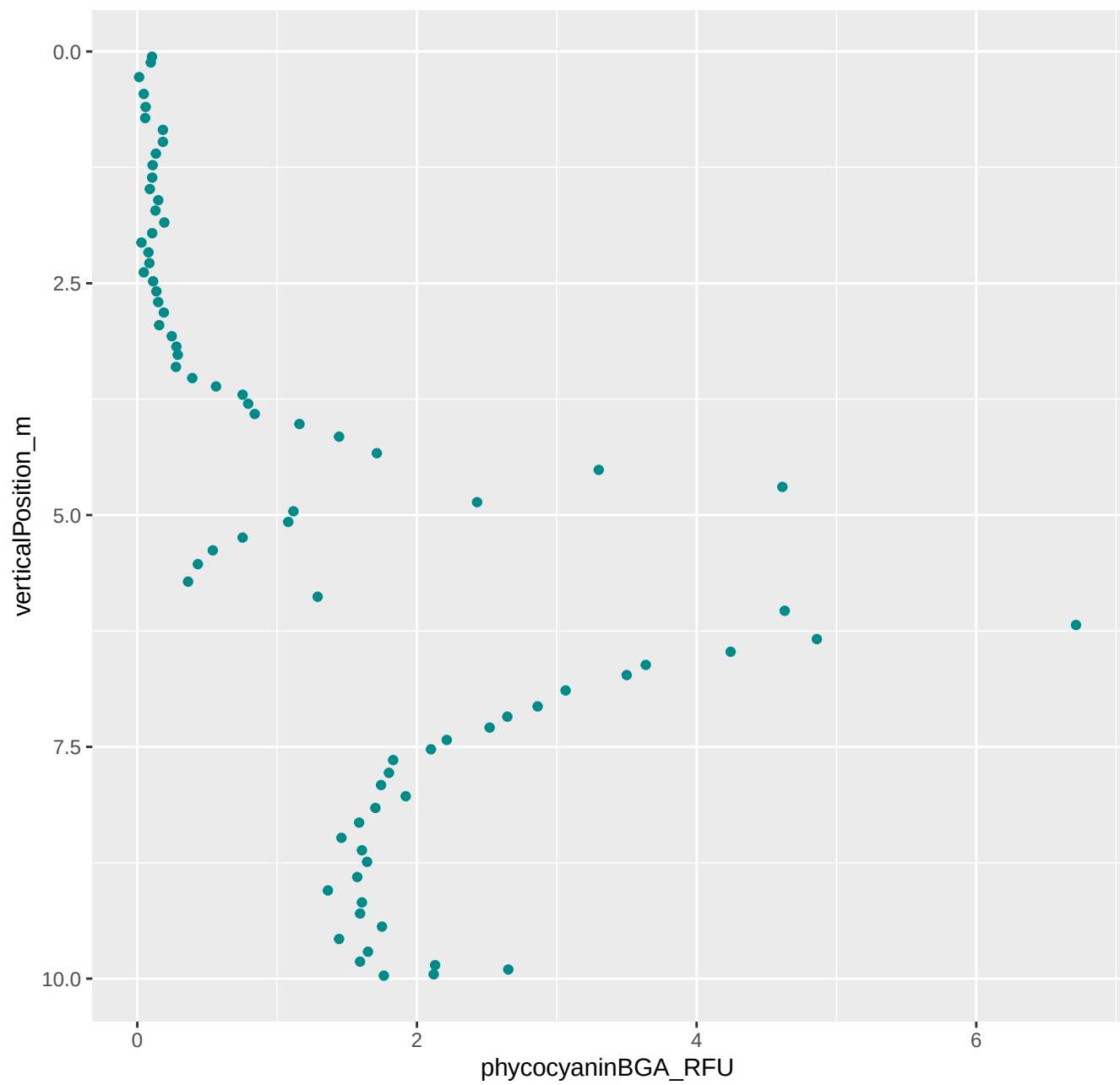
182_2023_07_12_Level1.csv ****bga jumps
