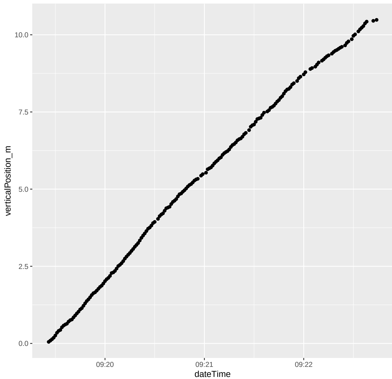
182_2023_08_02_Level1.csv ****Depth vs. time
