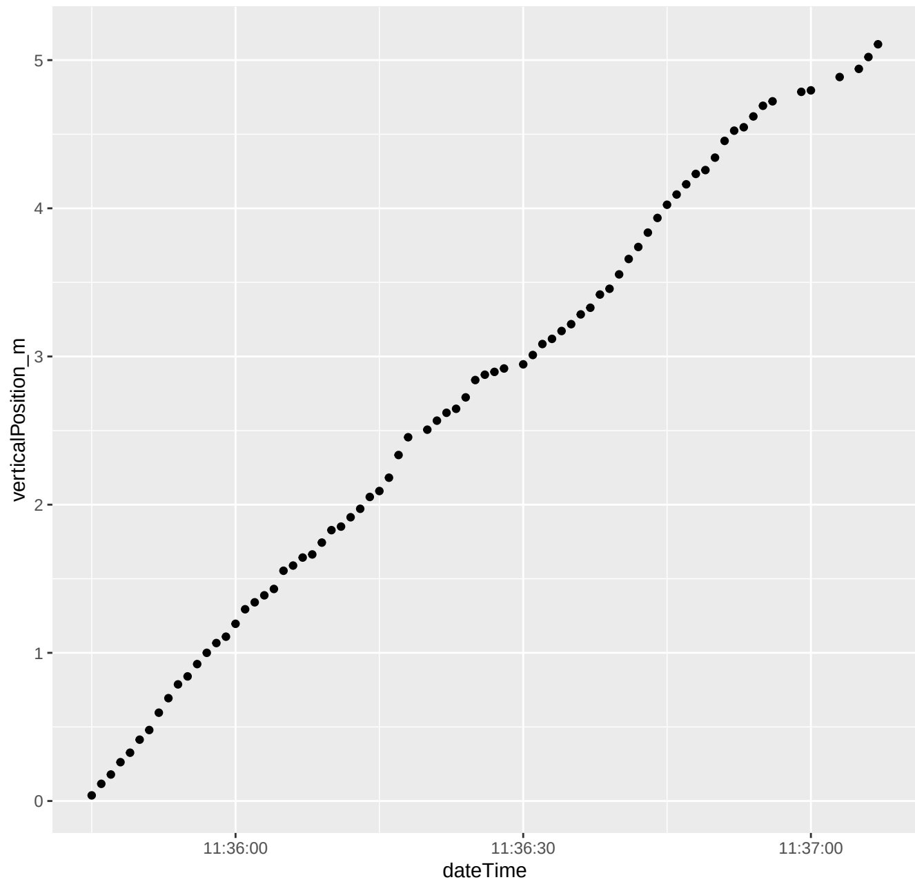
276_2023_08_10_Level1.csv ****Depth vs. time
