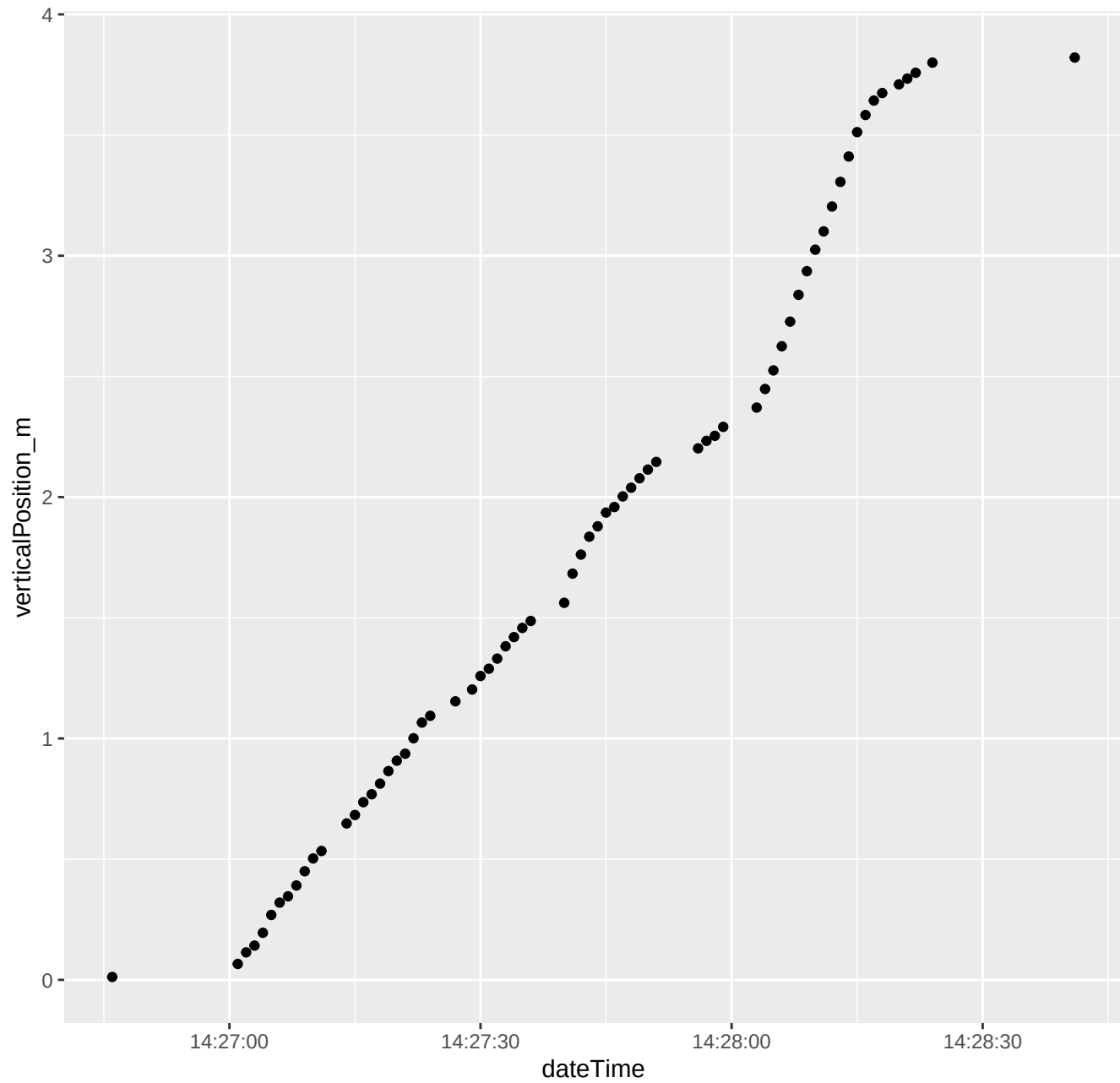
195_2025_08_04_Level1.csv ****Depth vs. time
