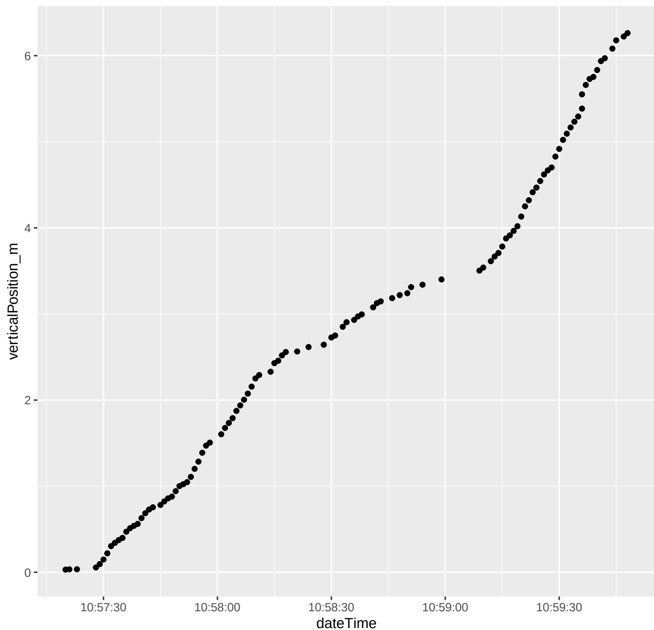
185_2025_07_15_Level1.csv ****Depth vs. time
