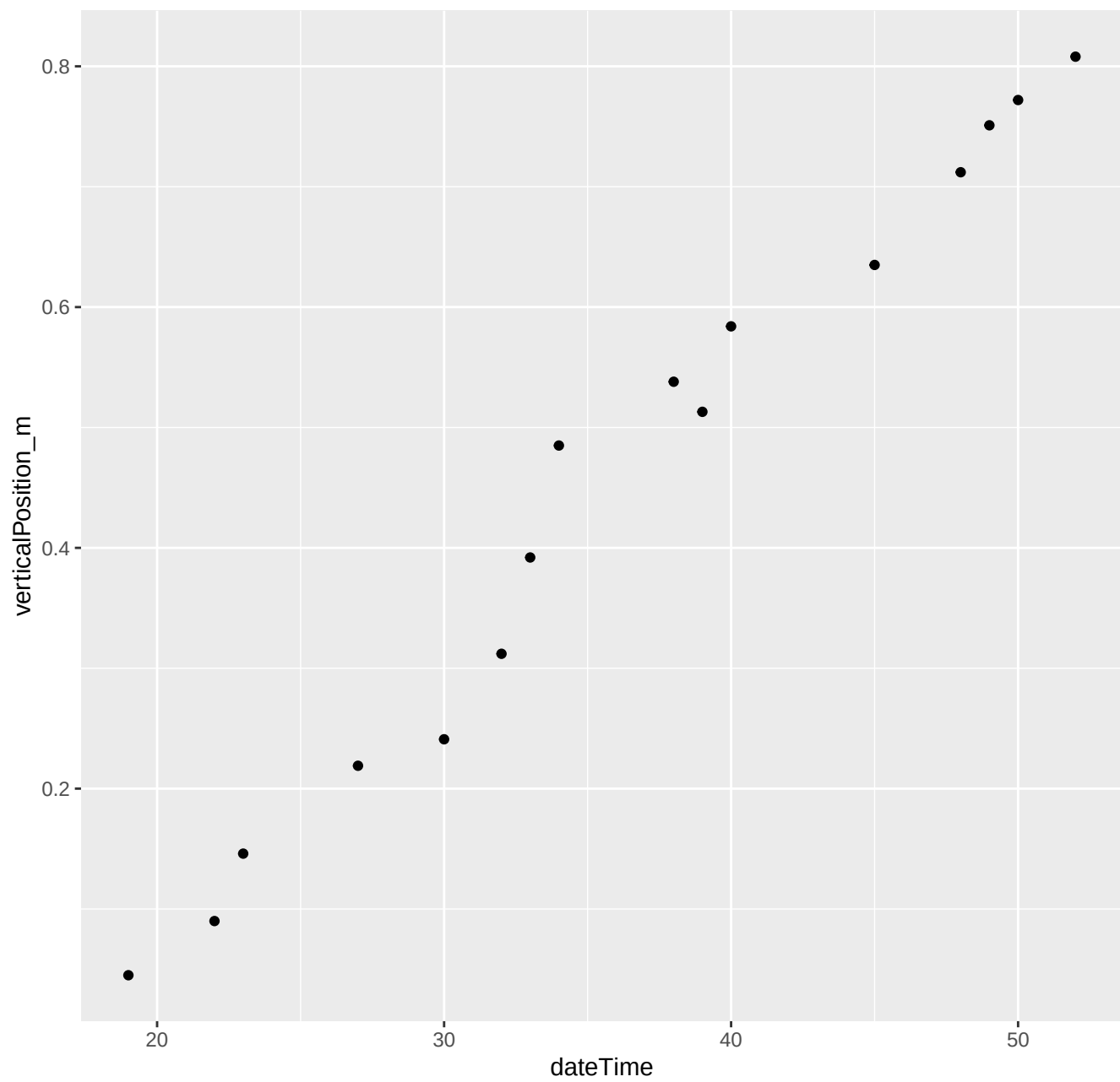
111-C8-0182_2025_10_10_Level1.csv ****Depth vs. time
