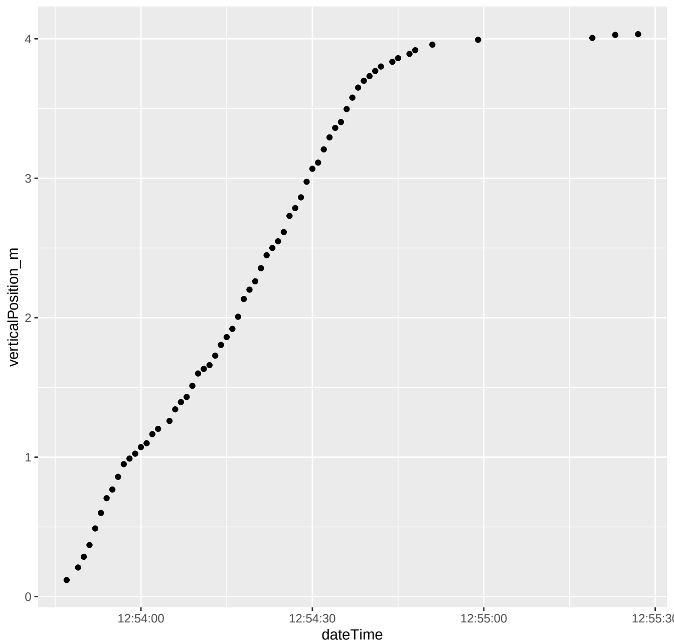
440_2025_04_21_Level1.csv ****Depth vs. time
