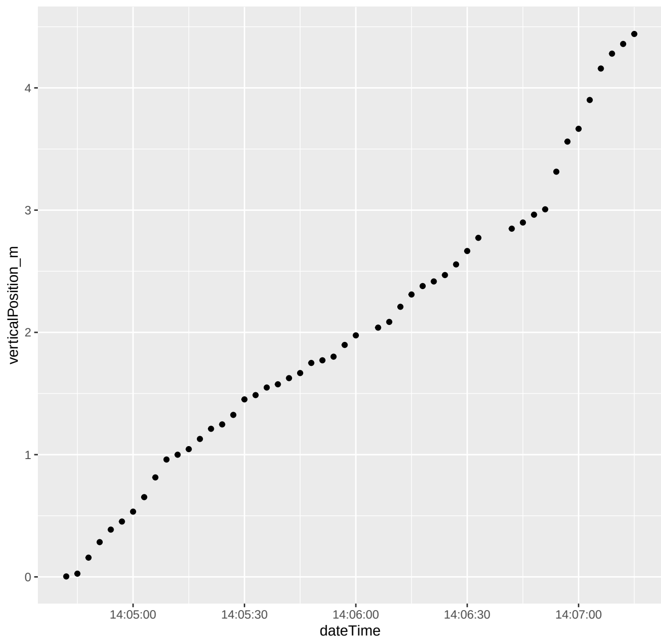
150_2025_07_01_Level1.csv ****Depth vs. time
