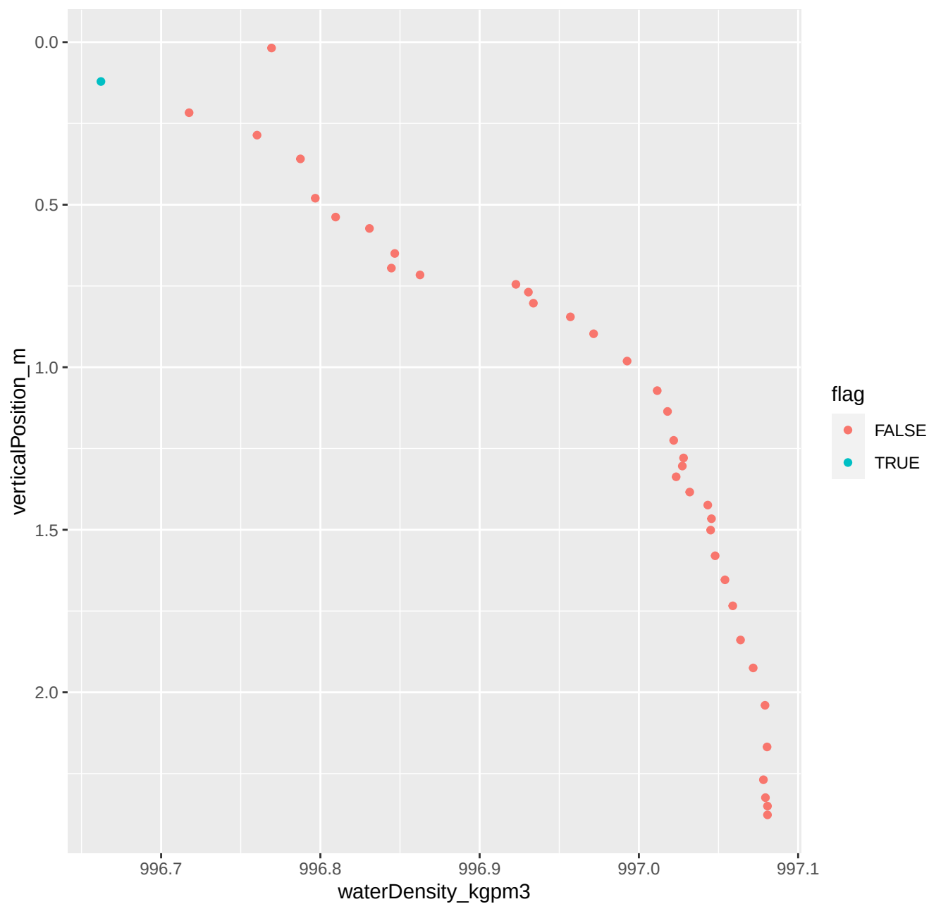
163_2025_08_04_Level1.csv ****Non-monotonic densities
