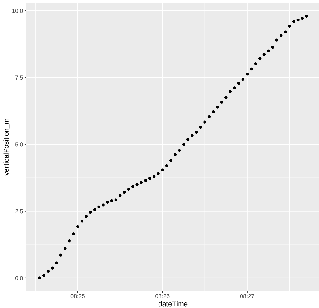
181_2025_08_05_Level1.csv ****Depth vs. time
