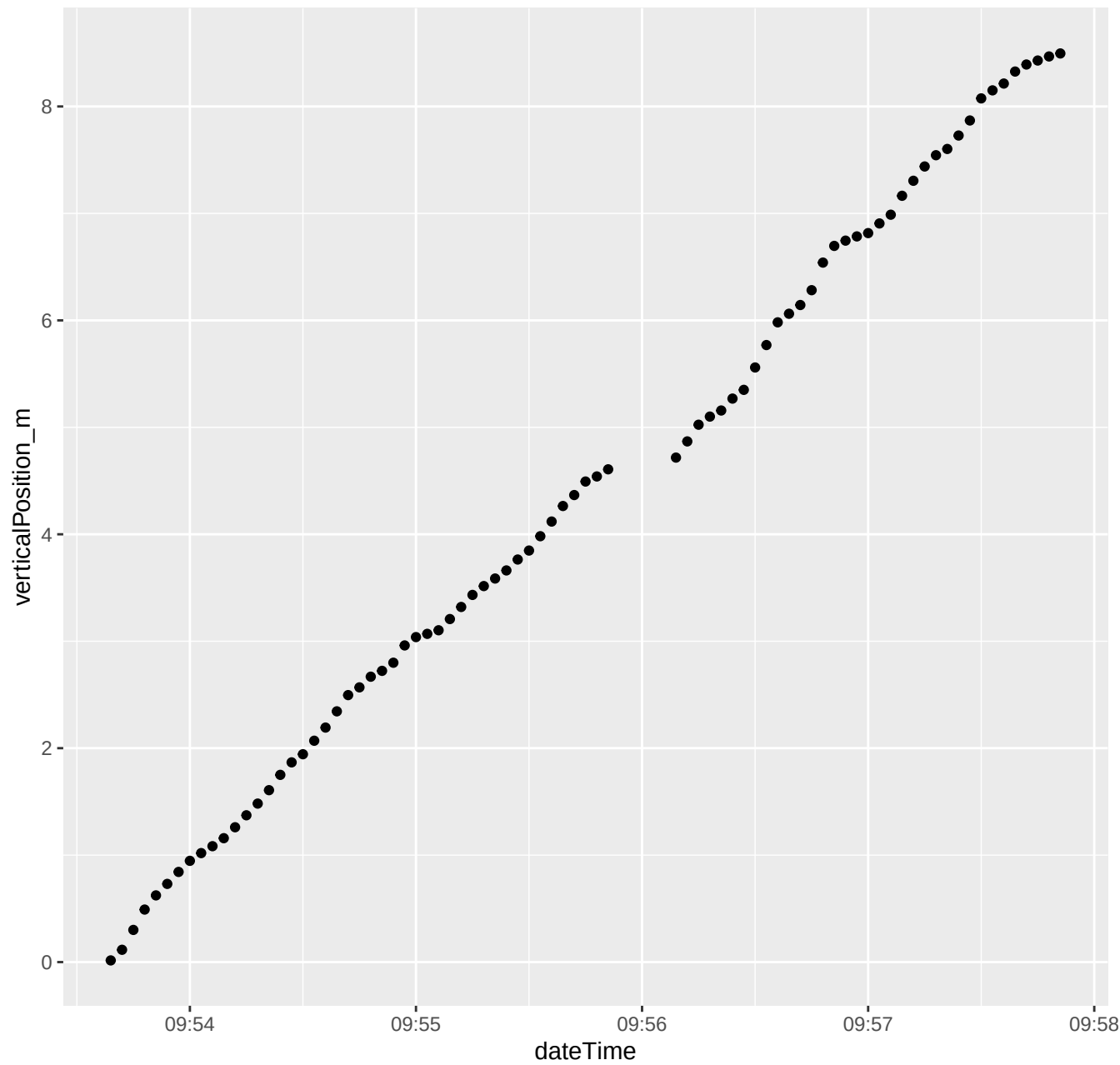
184_2025_06_30_Level1.csv ****Depth vs. time
