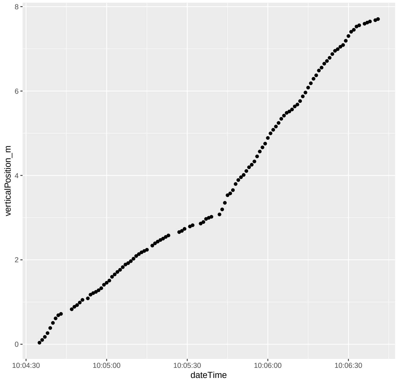
081_2025_08_13_Level1.csv ****Depth vs. time
