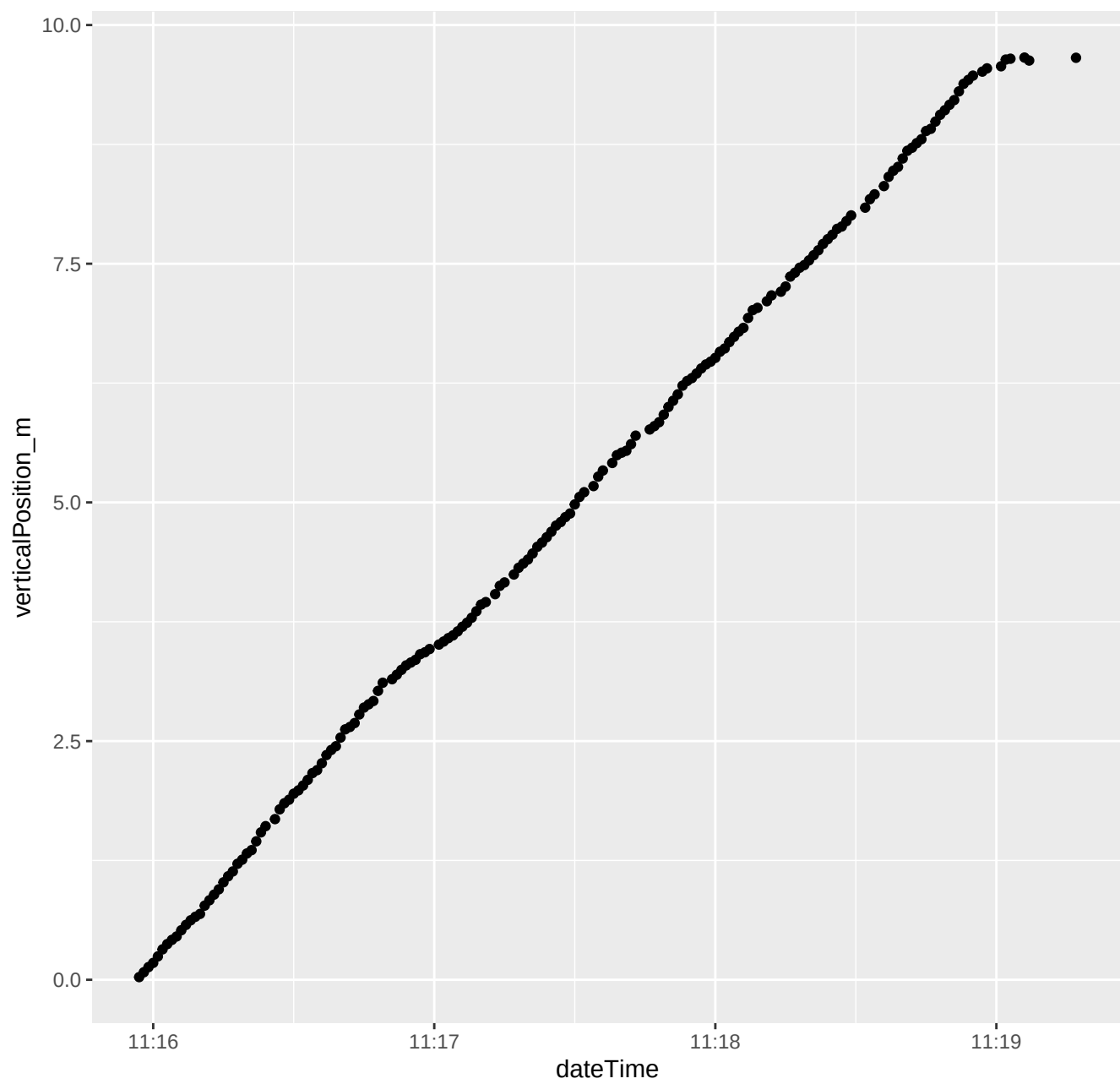
087_2025_07_10_Level1.csv ****Depth vs. time
