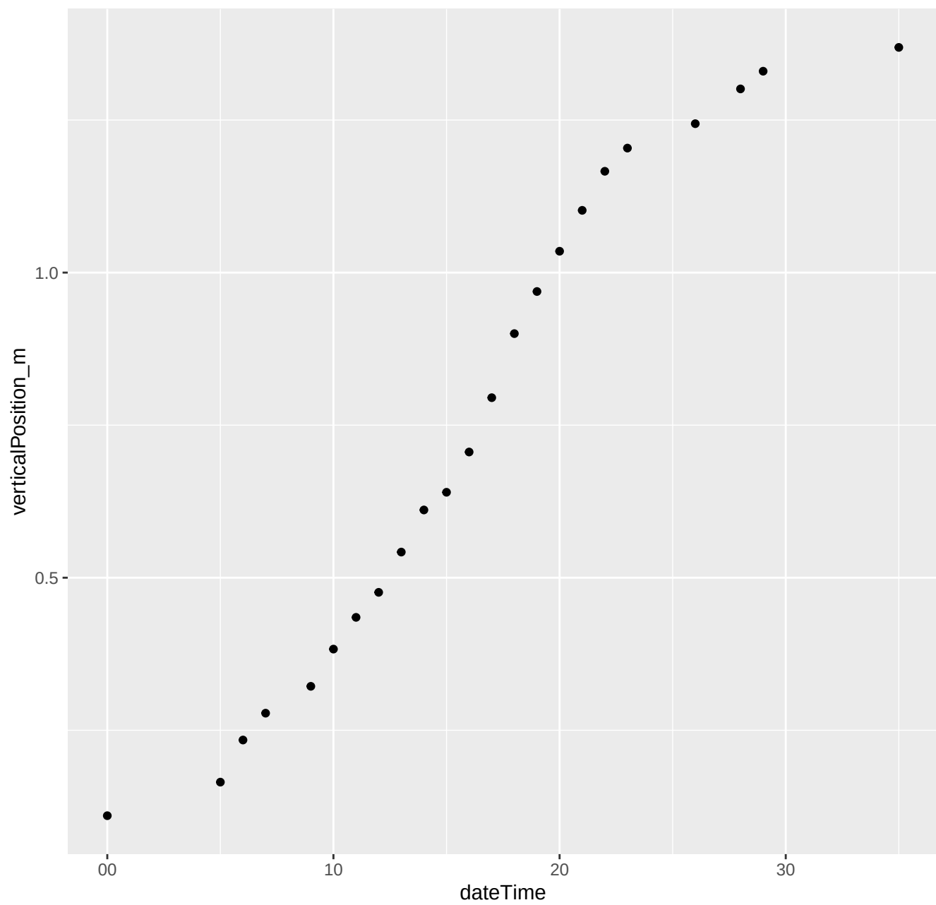
111-C8-0182_2025_06_09_Level1.csv ****Depth vs. time
