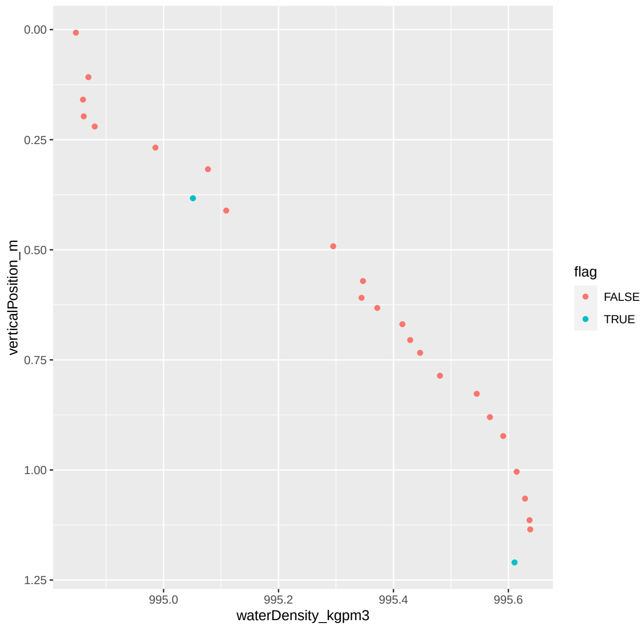
272_2025_07_28_Level1.csv ****Non-monotonic densities
