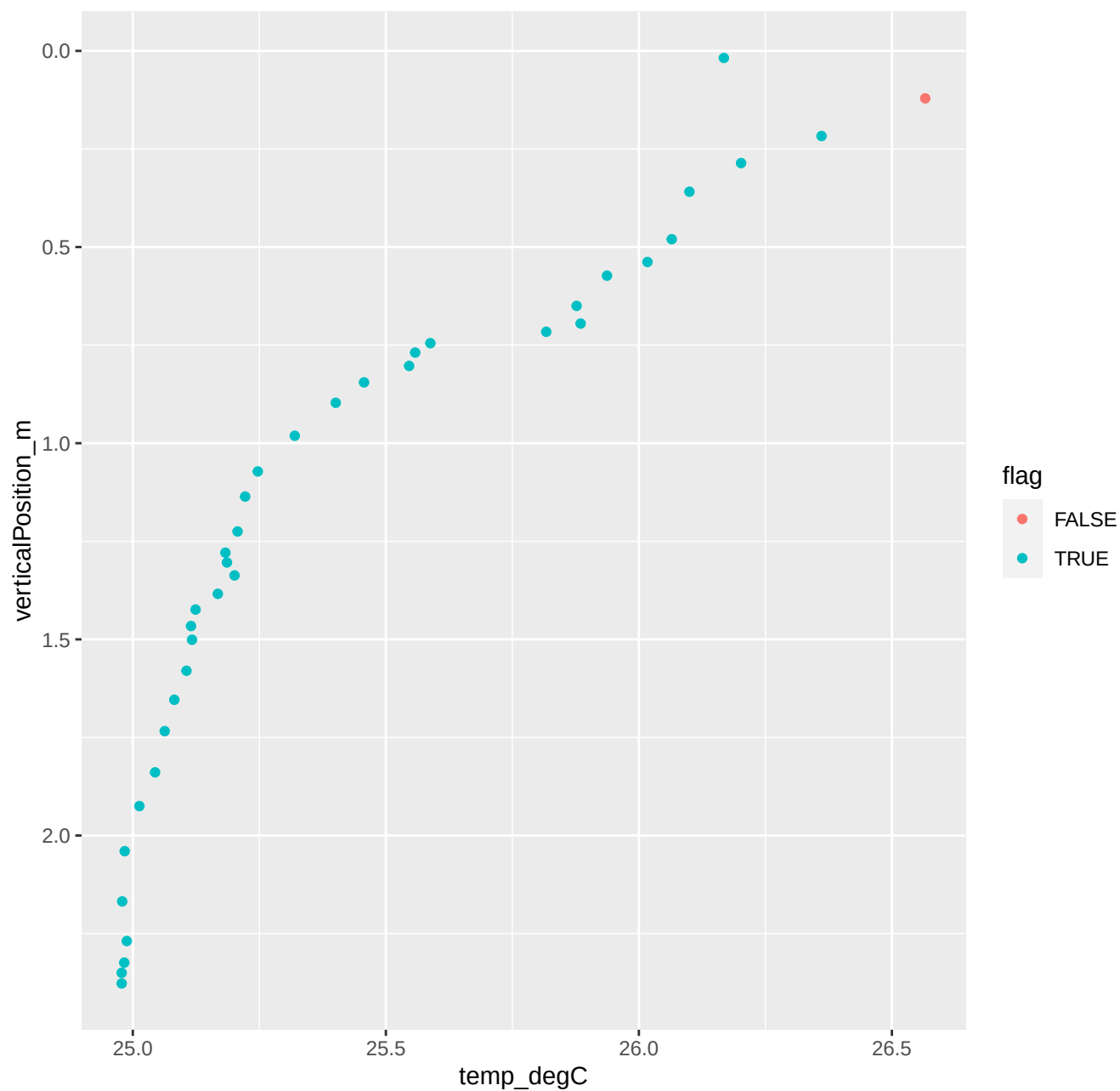
163_2025_08_04_Level1.csv ****Non-decreasing temps
