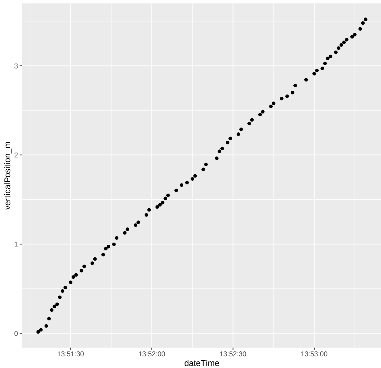
219_2025_04_16_Level1.csv ****Depth vs. time
