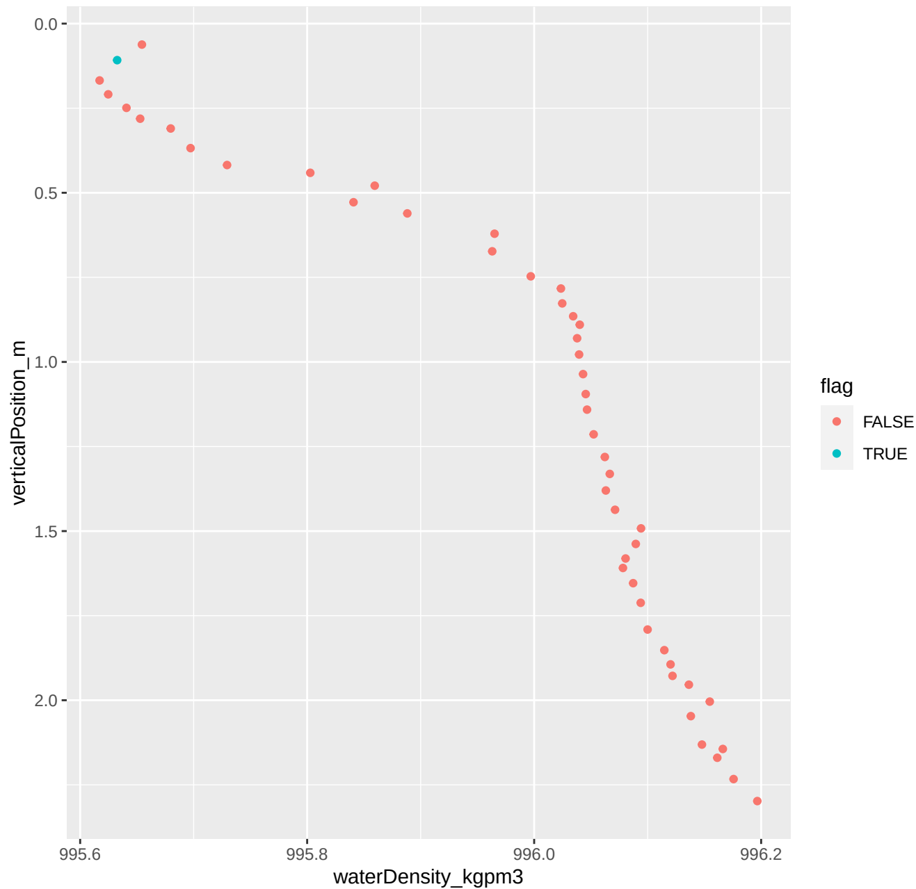
163_2025_07_14_Level1.csv ****Non-monotonic densities
