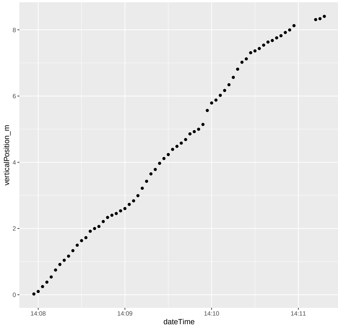
238_2025_07_28_Level1.csv ****Depth vs. time
