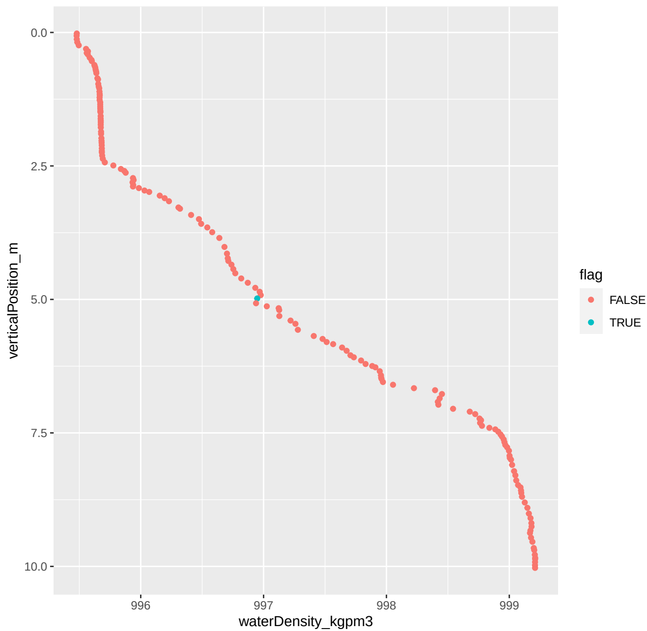
087_2025_07_29_Level1.csv ****Non-monotonic densities
