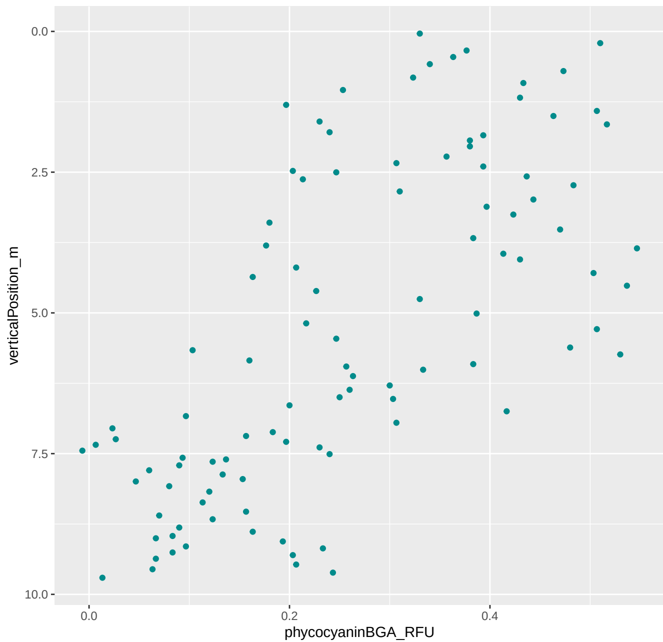
181_2025_06_24_Level1.csv ****bga jumps
