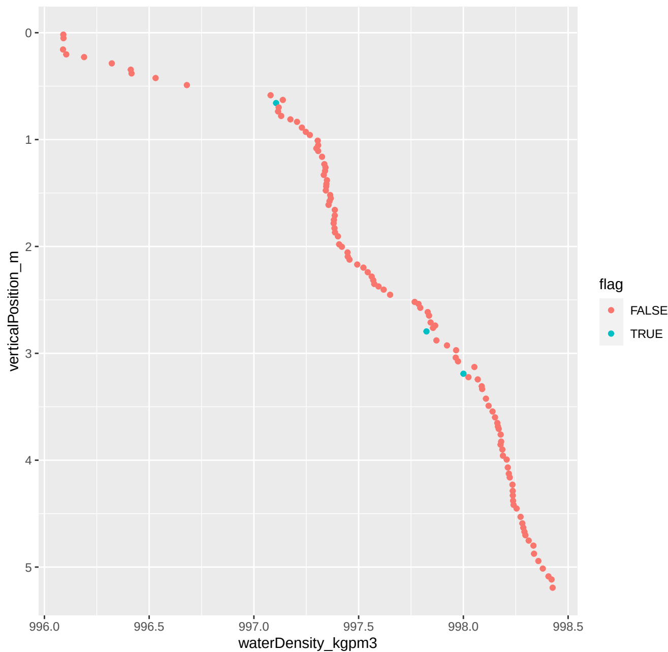
024_2025_06_17_Level1.csv ****Non-monotonic densities
