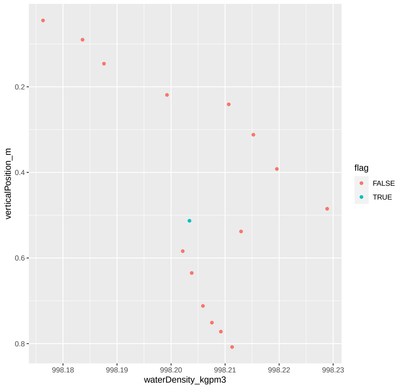
111-C8-0182_2025_10_10_Level1.csv ****Non-monotonic densities
