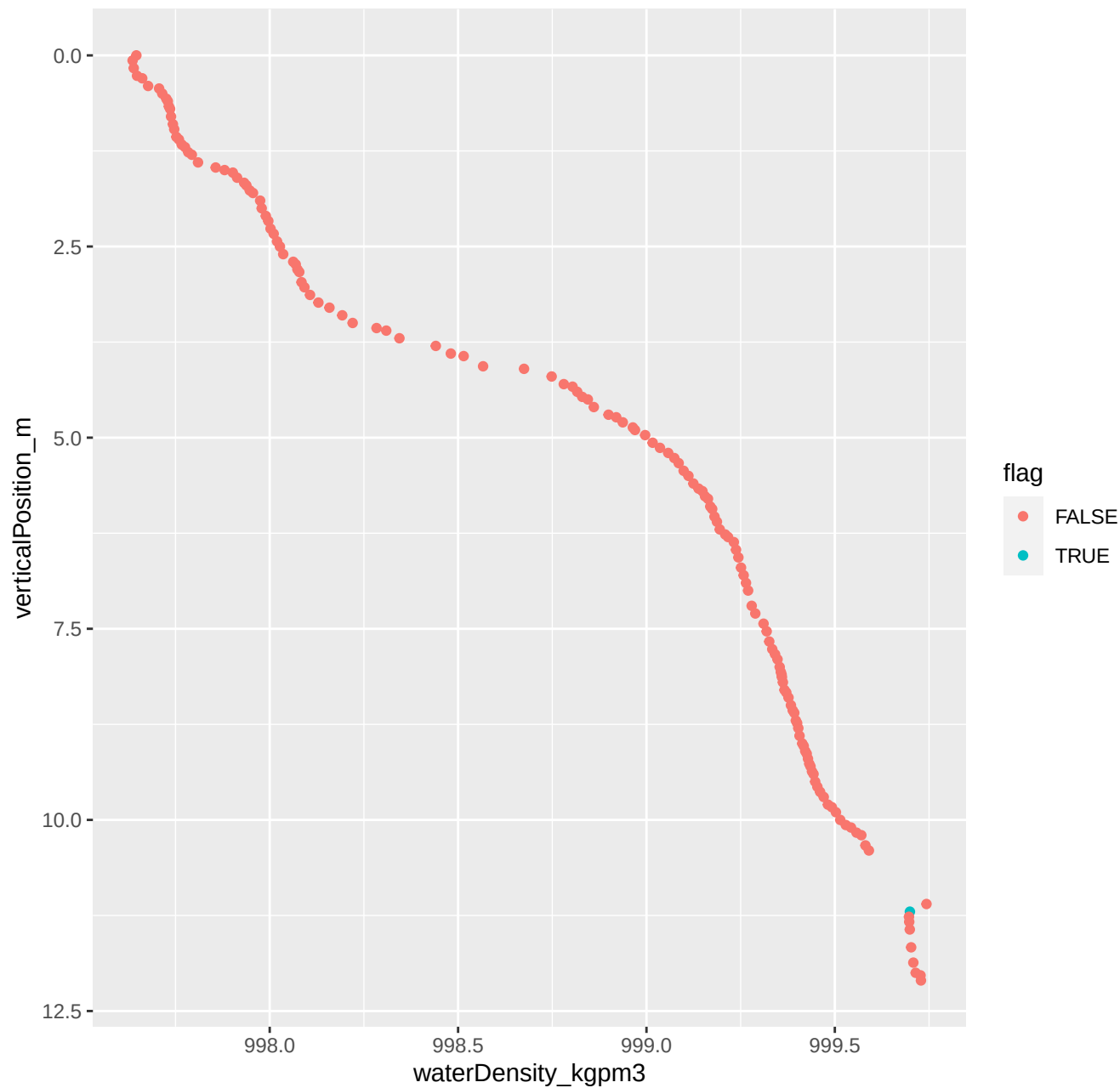
039_2017_05_30_Level1.csv ****Non-monotonic densities
