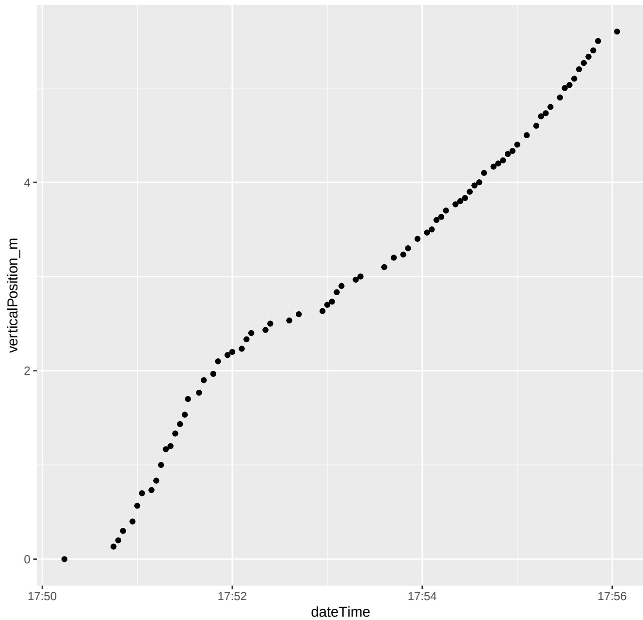
184_2017_05_24_Level1.csv ****Depth vs. time
