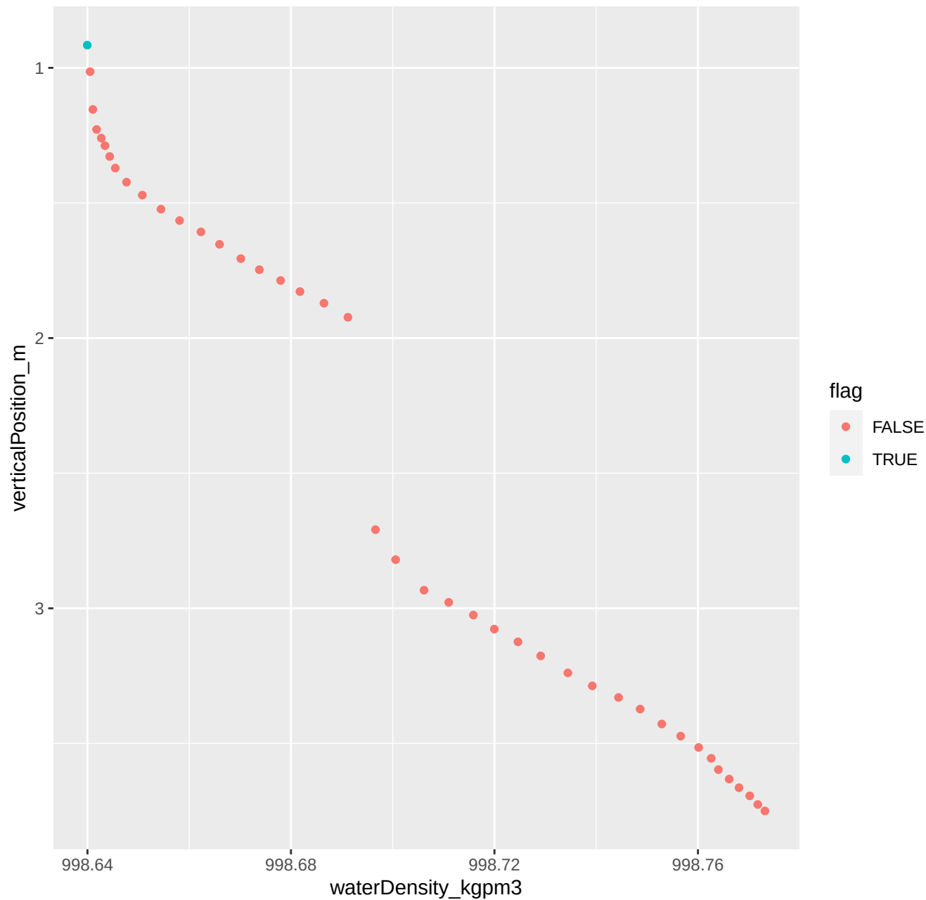
219_2017_10_17_Level1.csv ****Non-monotonic densities
