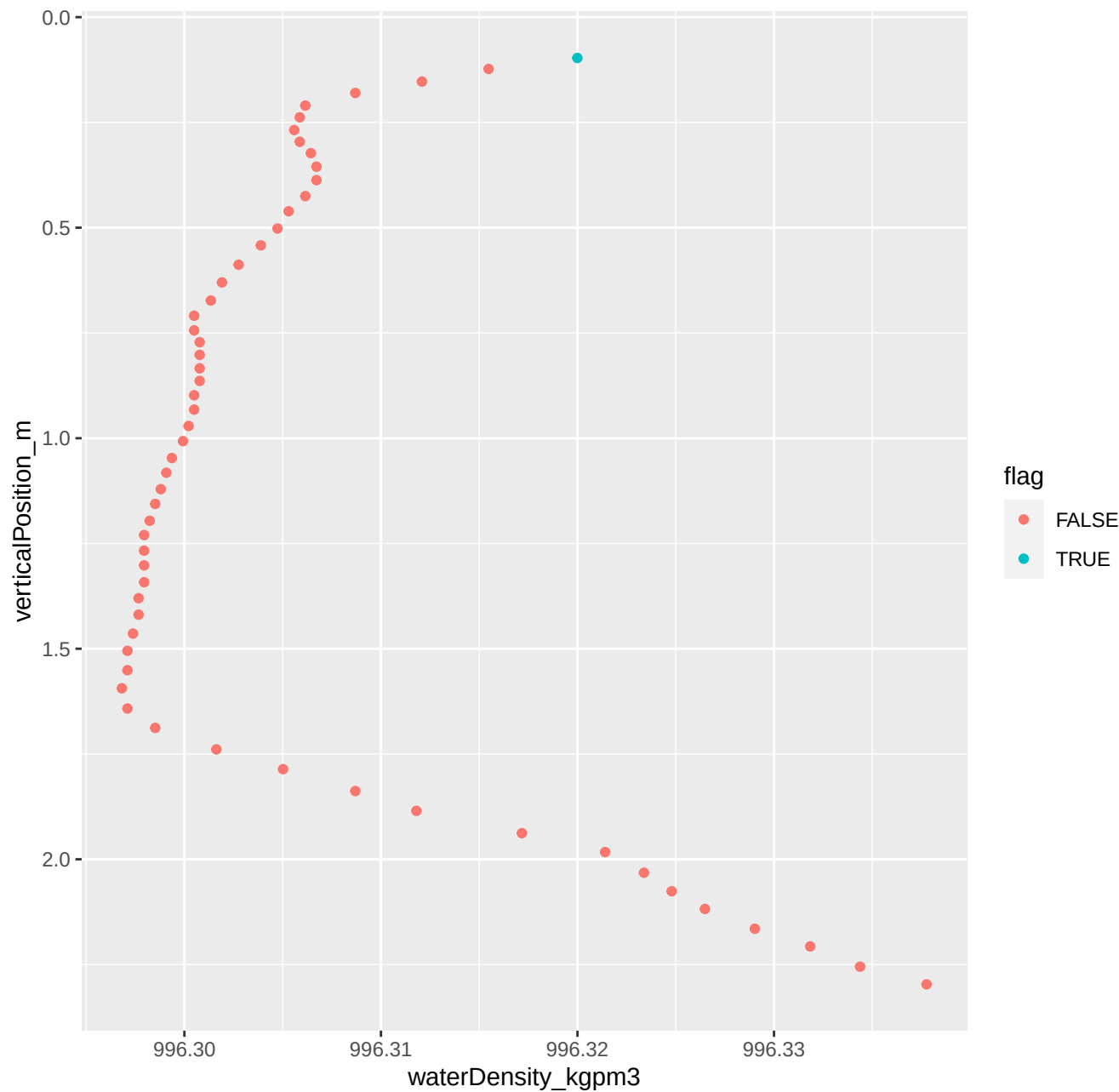
186_2018_07_24_P_Level1.csv ****Non-monotonic densities
