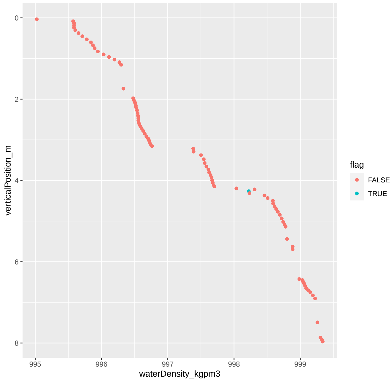
094_2018_06_06_Level1.csv ****Non-monotonic densities
