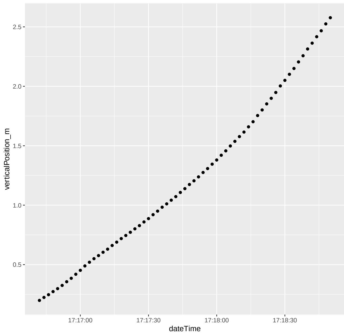
236_2018_06_27_Level1.csv ****Depth vs. time
