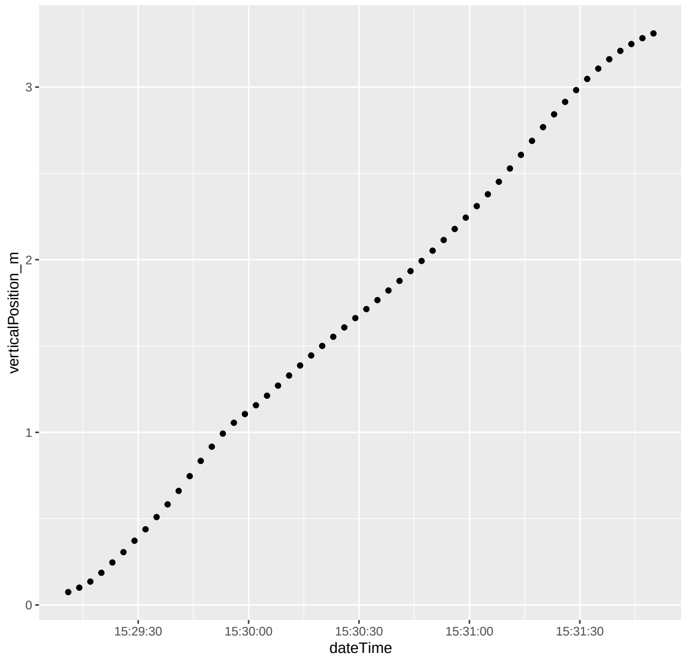
059_2018_08_06_Level1.csv ****Depth vs. time
