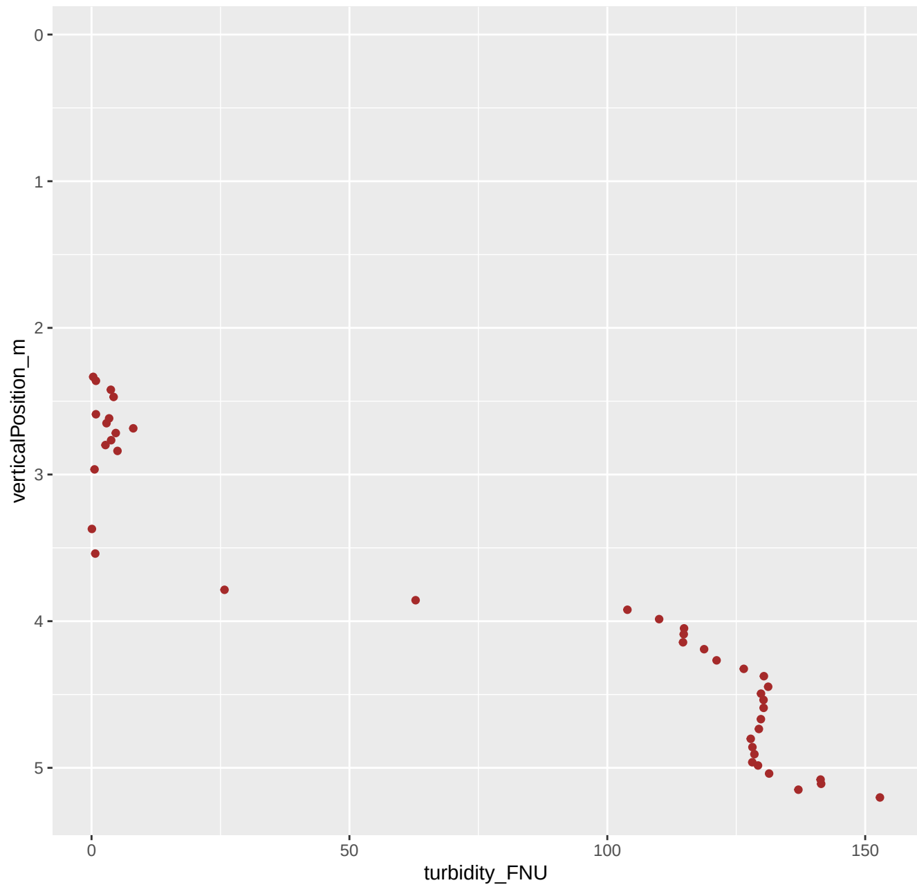
258_2019_06_26_Level1.csv ****Turbidity jumps
