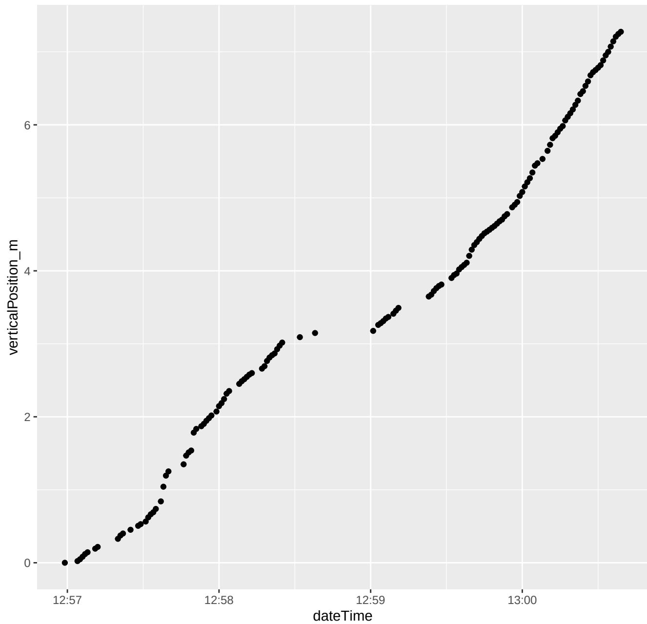
117_2019_07_11_Level1.csv ****Depth vs. time
