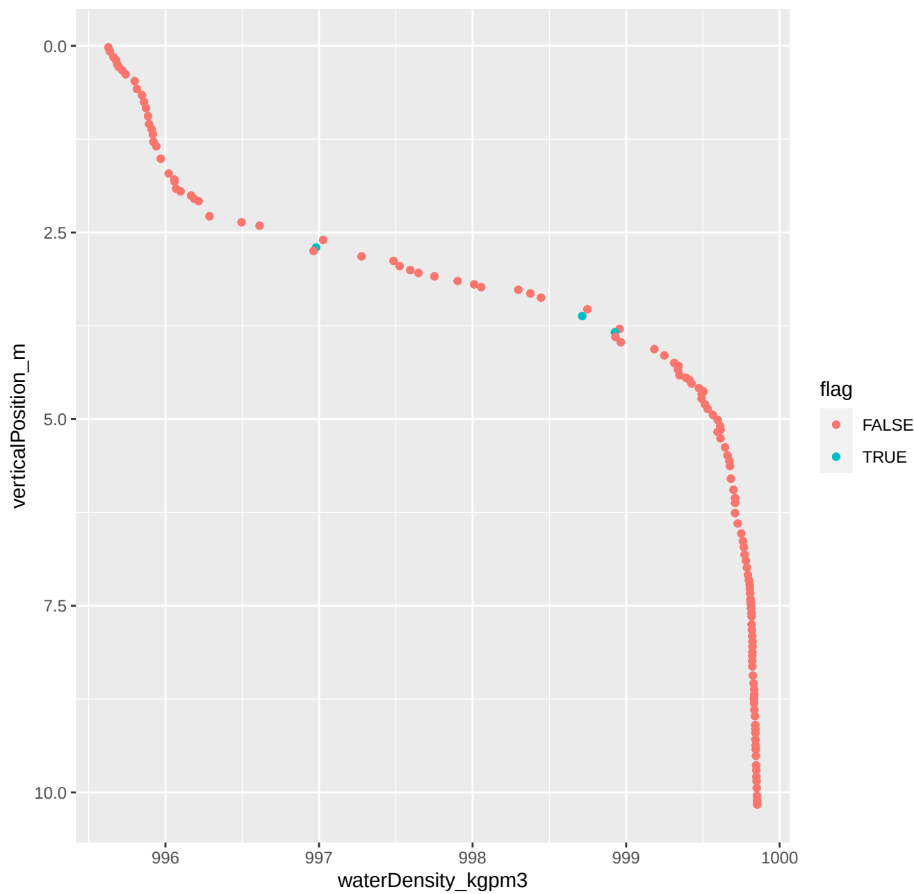
216_2019_08_06_Level1.csv ****Non-monotonic densities
