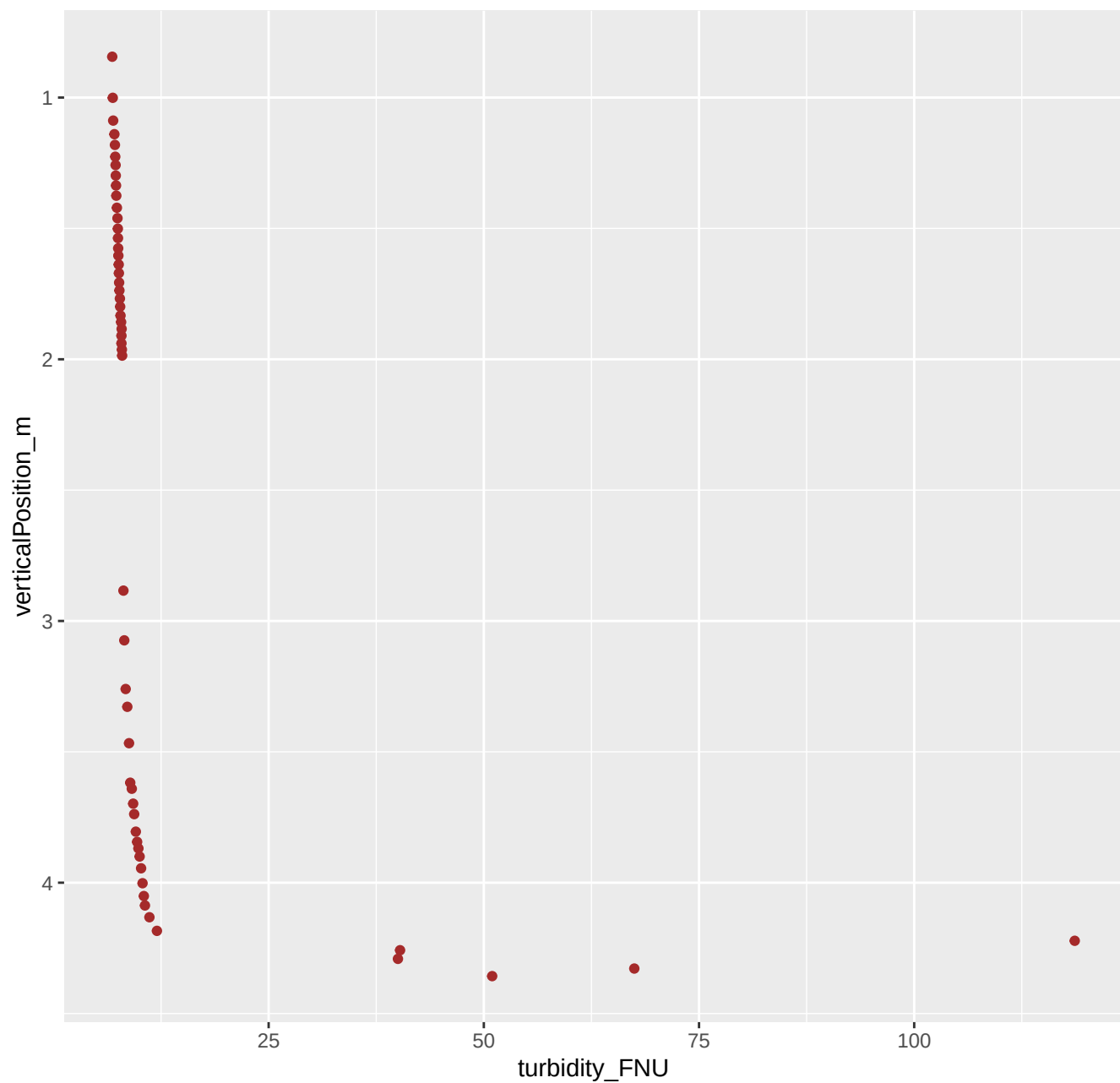
149-GG-03-30_2019_05_29_Level1.csv ****Turbidity jumps
