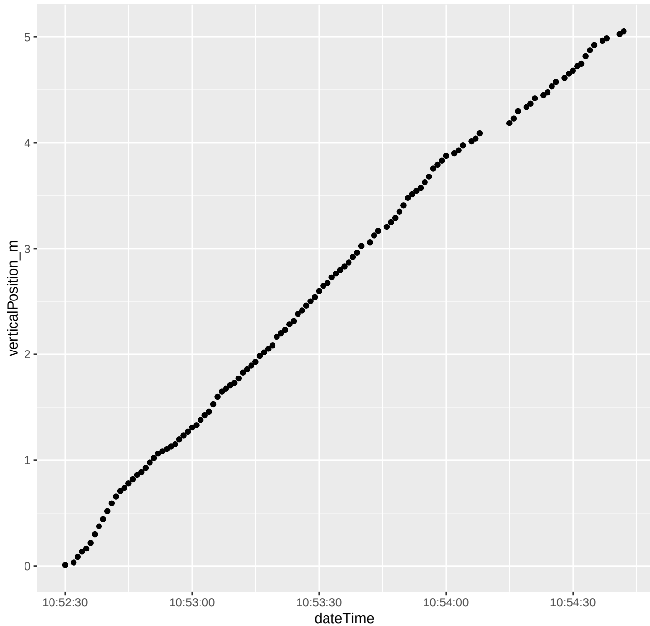
111-C5-0095_2025_08_12_Level1.csv ****Depth vs. time
