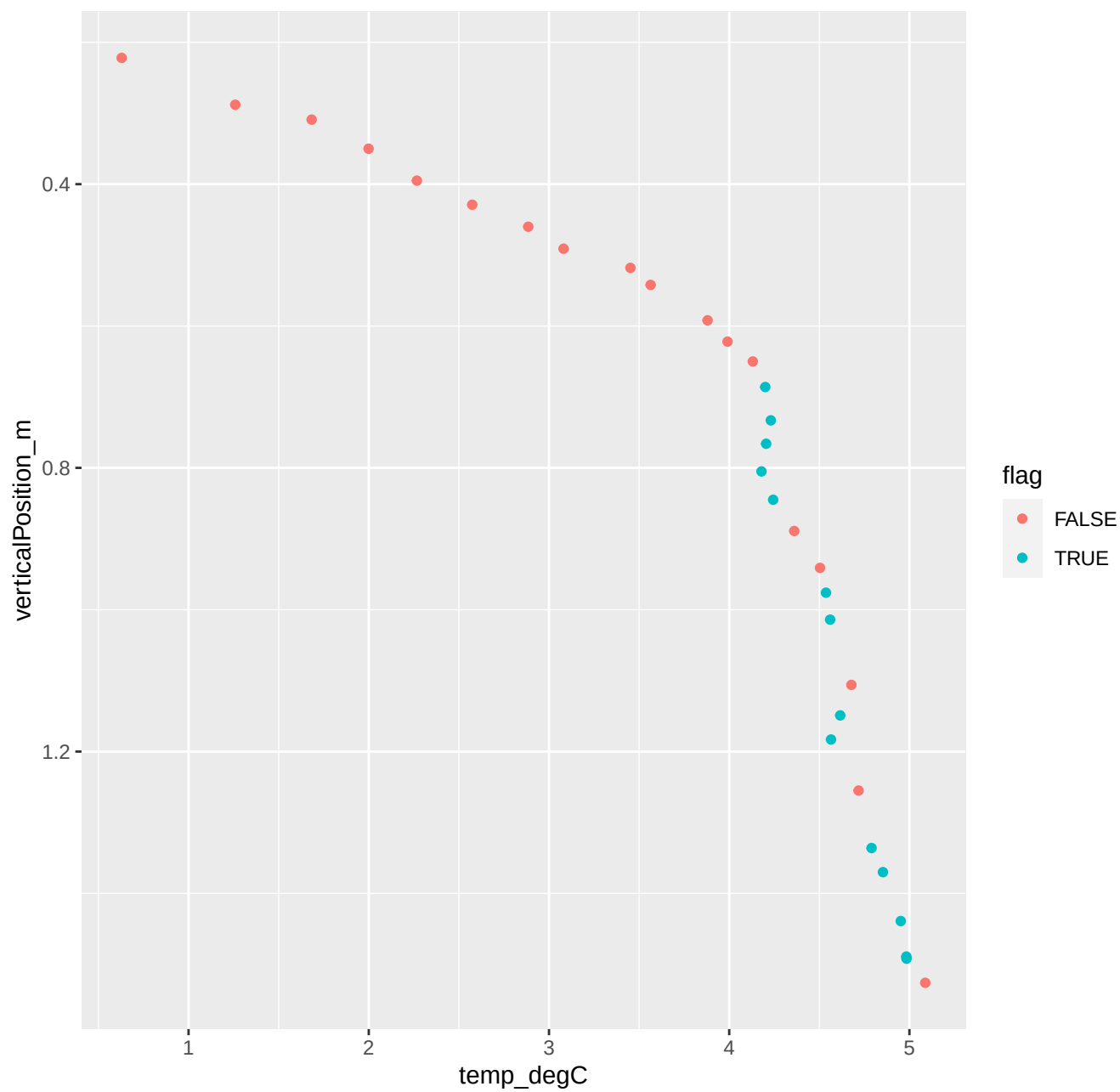
446_2025_01_08_Level1.csv ****Non-decreasing temps
