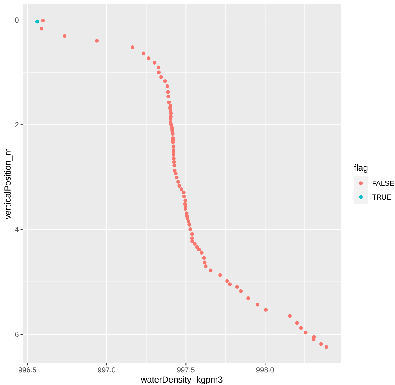
113_2025_06_10_Level1.csv ****Non-monotonic densities
