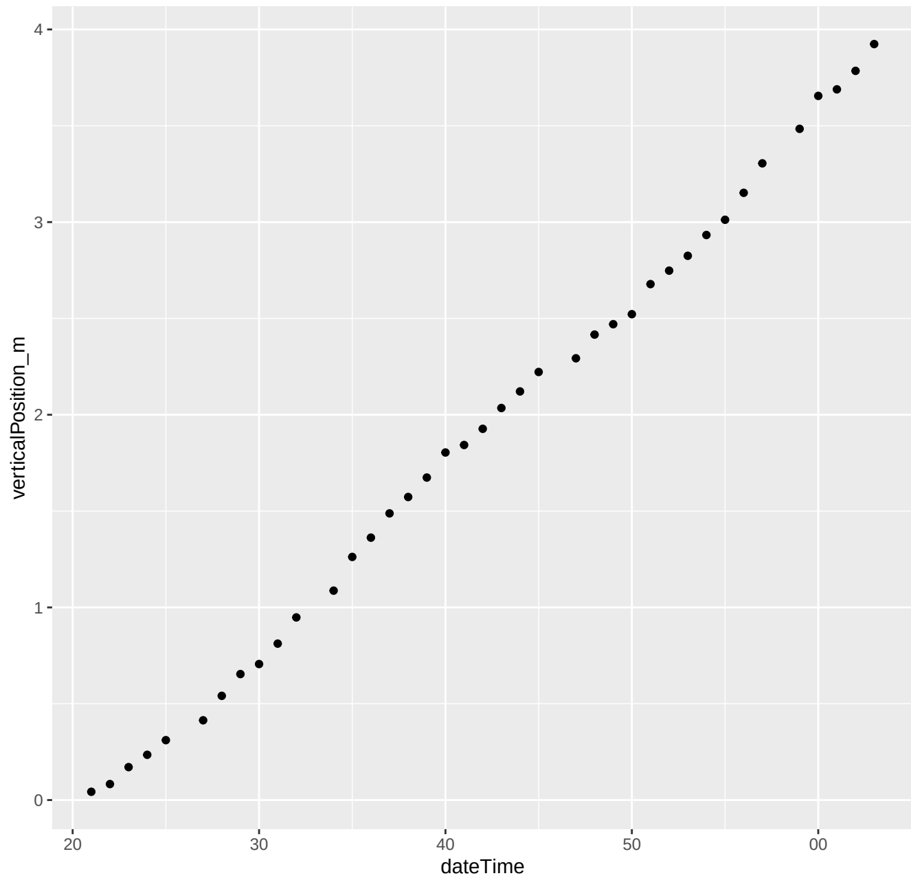
111-C5-0095_2025_05_27_Level1.csv ****Depth vs. time
