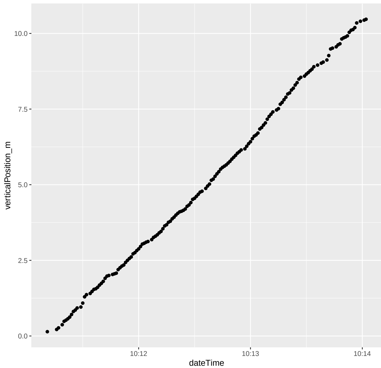
111_2025_09_23_Level1.csv ****Depth vs. time
