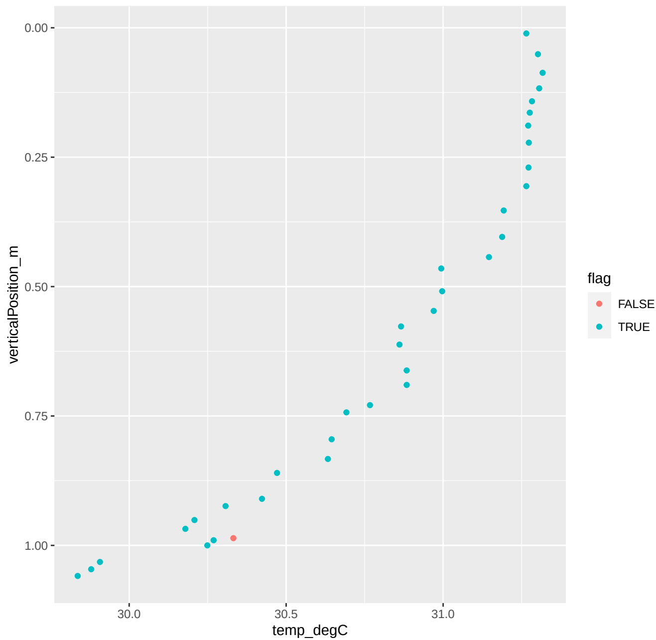
272_2024_06_24_Level1.csv ****Non-decreasing temps
