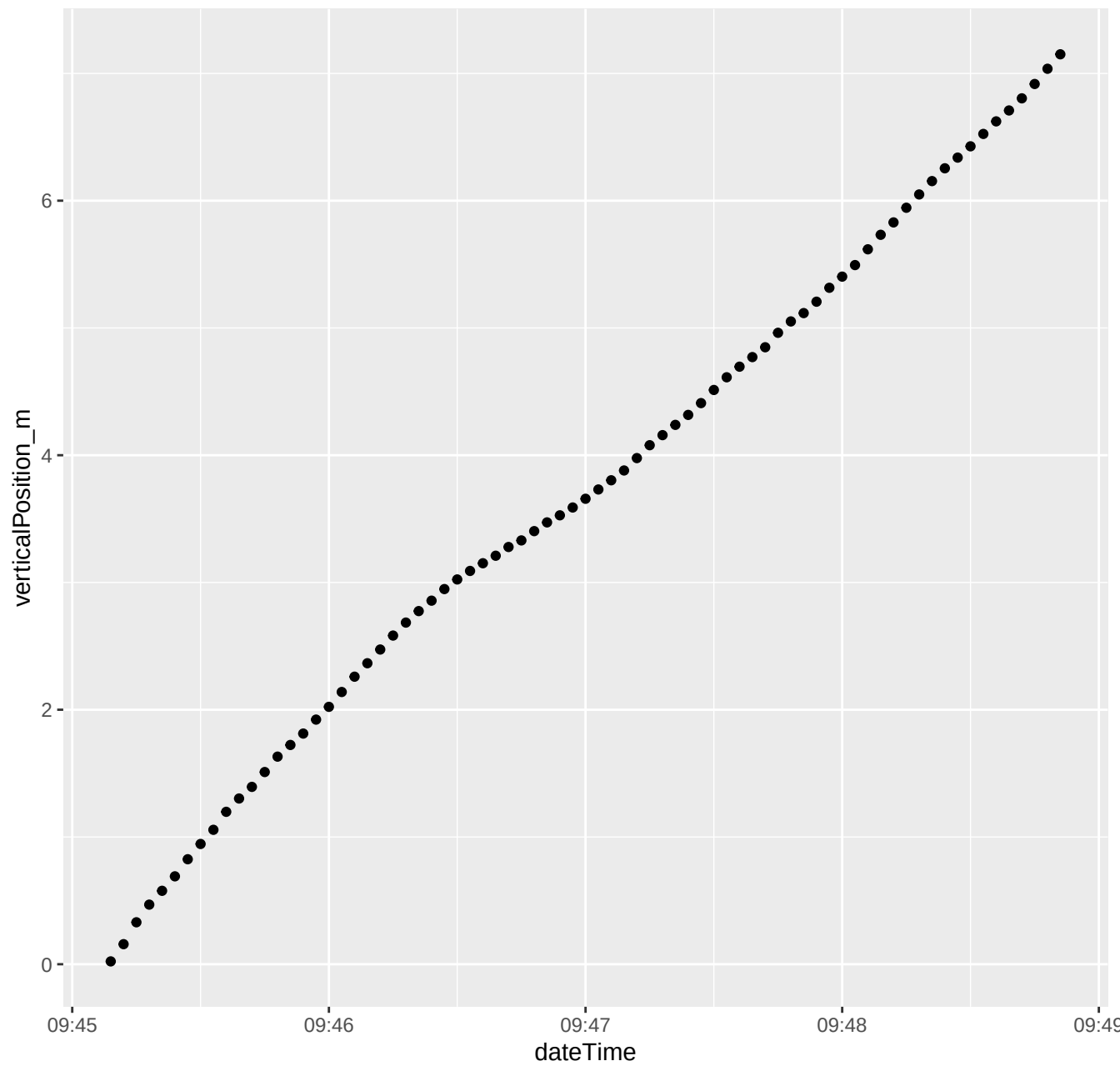
036_2024_08_14_Level1.csv ****Depth vs. time
