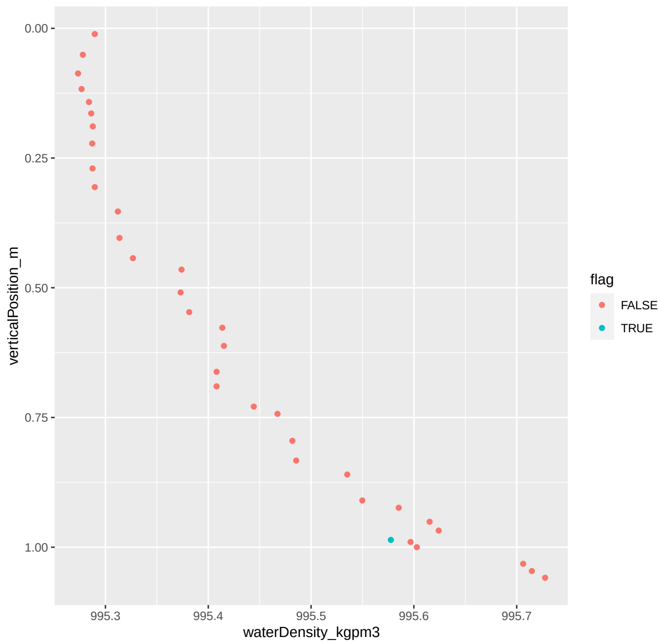
272_2024_06_24_Level1.csv ****Non-monotonic densities
