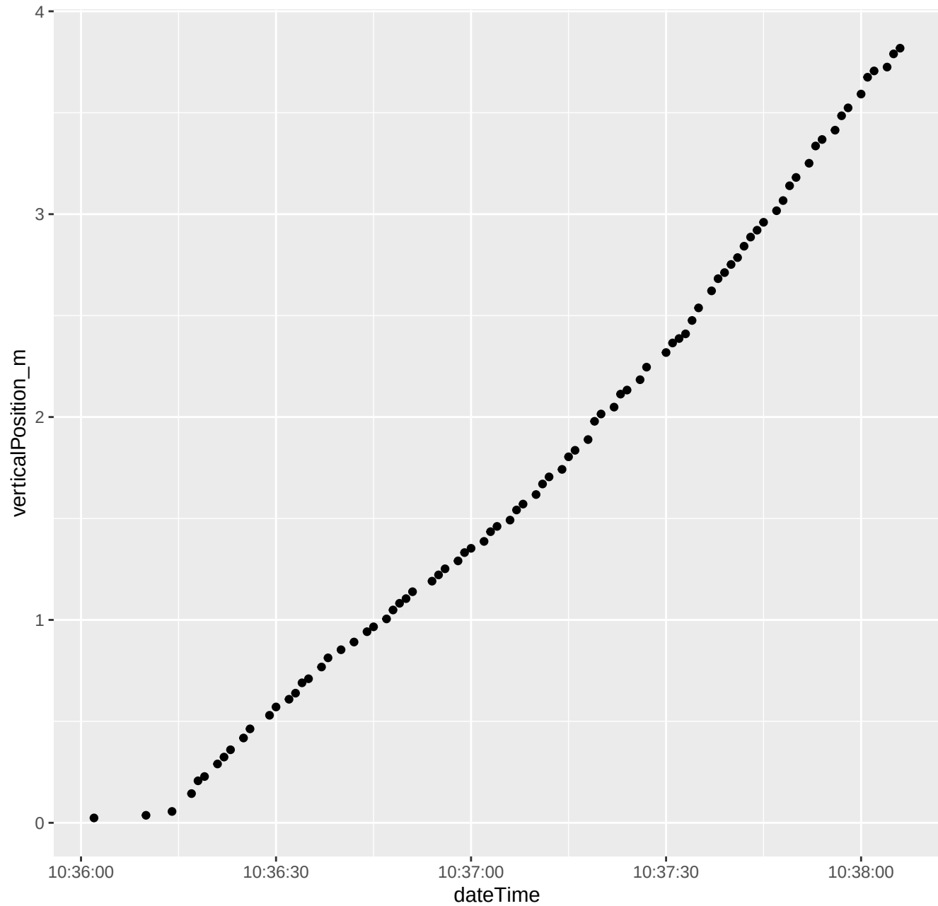
317_2024_06_20_Level1.csv ****Depth vs. time
