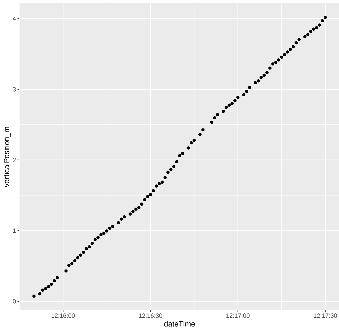
219_2024_11_13_Level1.csv ****Depth vs. time
