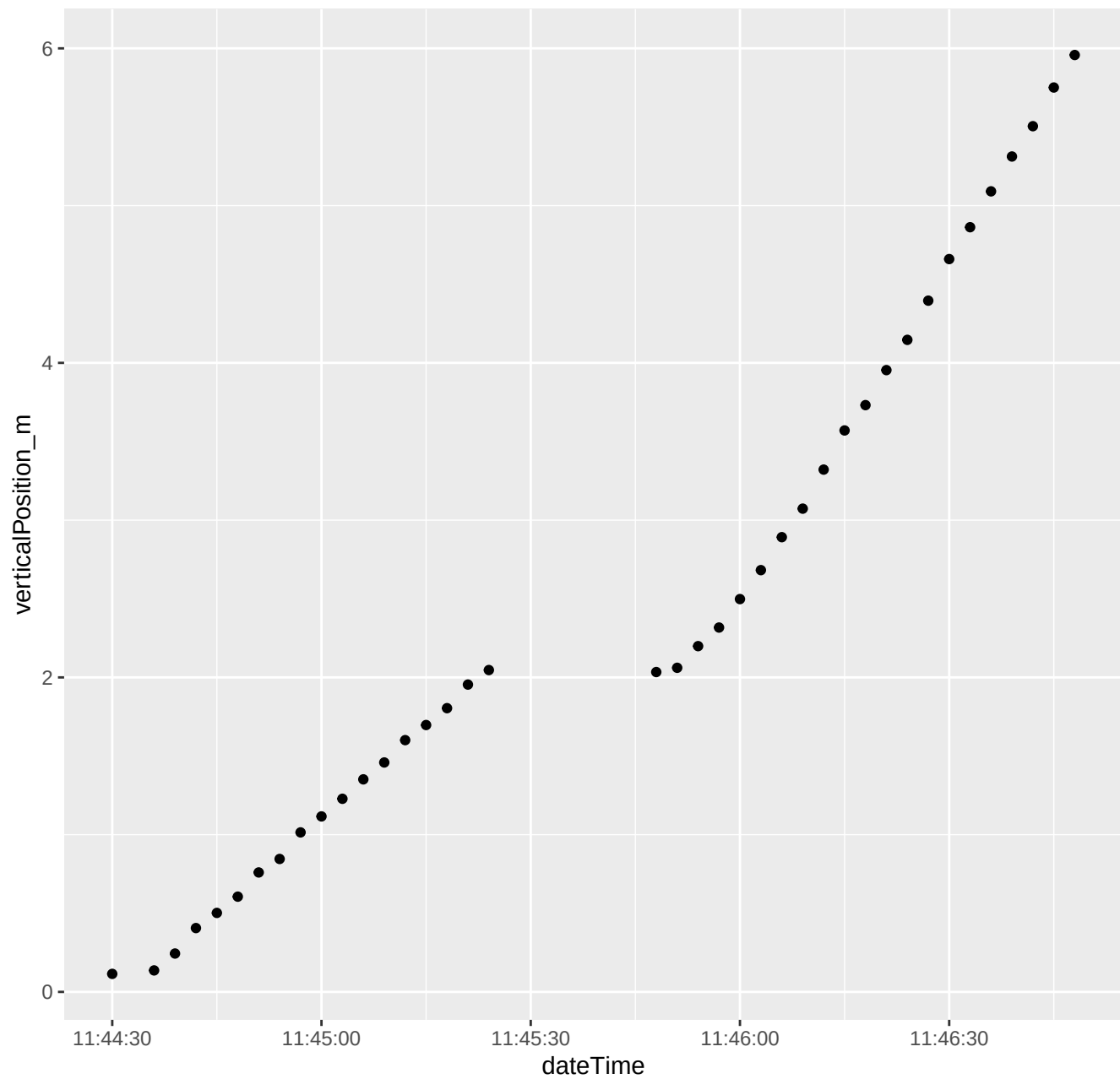
411_2024_06_06_Level1.csv ****Depth vs. time
