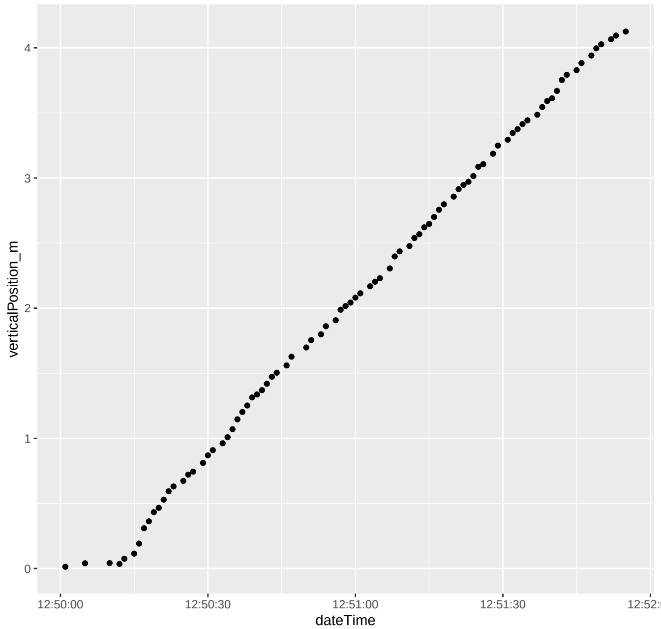
219_2024_09_06_Level1.csv ****Depth vs. time
