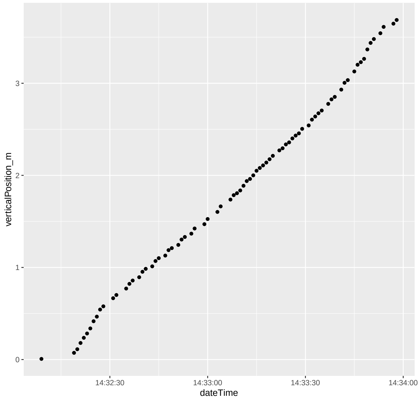
195_2024_07_08_Level1.csv ****Depth vs. time
