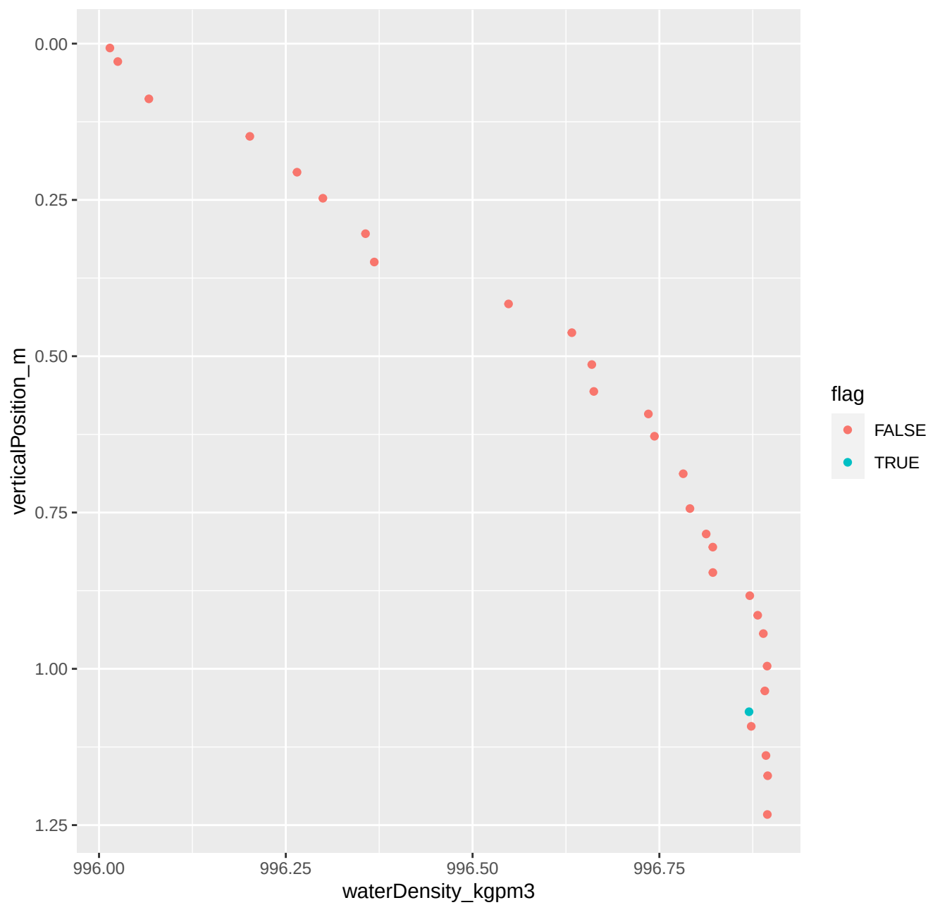
272_2024_07_22_Level1.csv ****Non-monotonic densities
