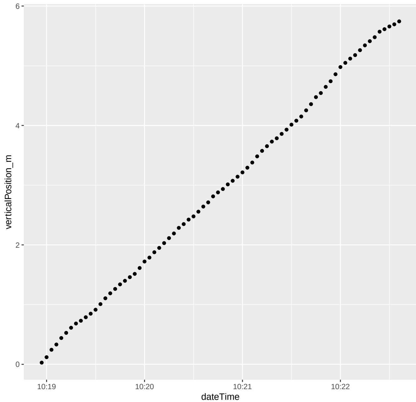
185_2024_07_09_Level1.csv ****Depth vs. time
