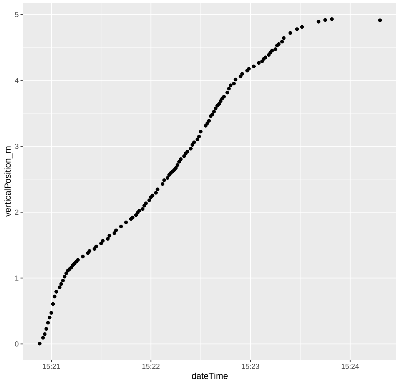
186_2025_05_28_Level1.csv ****Depth vs. time
