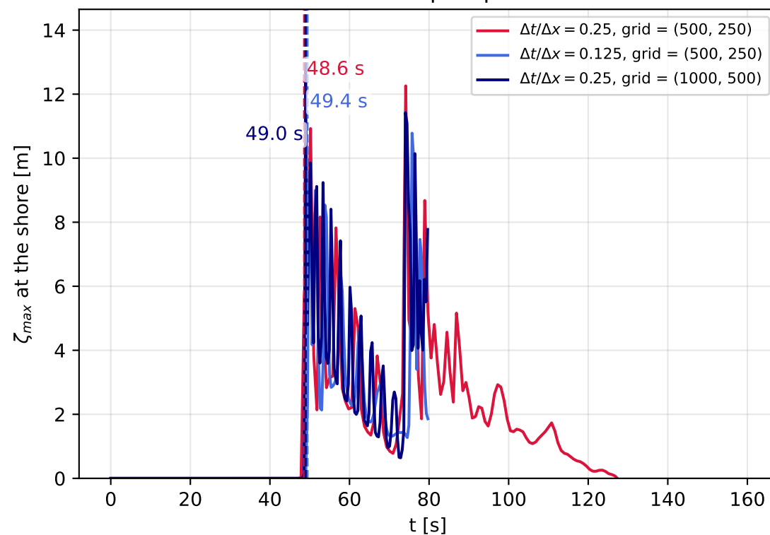
Two-step slope
