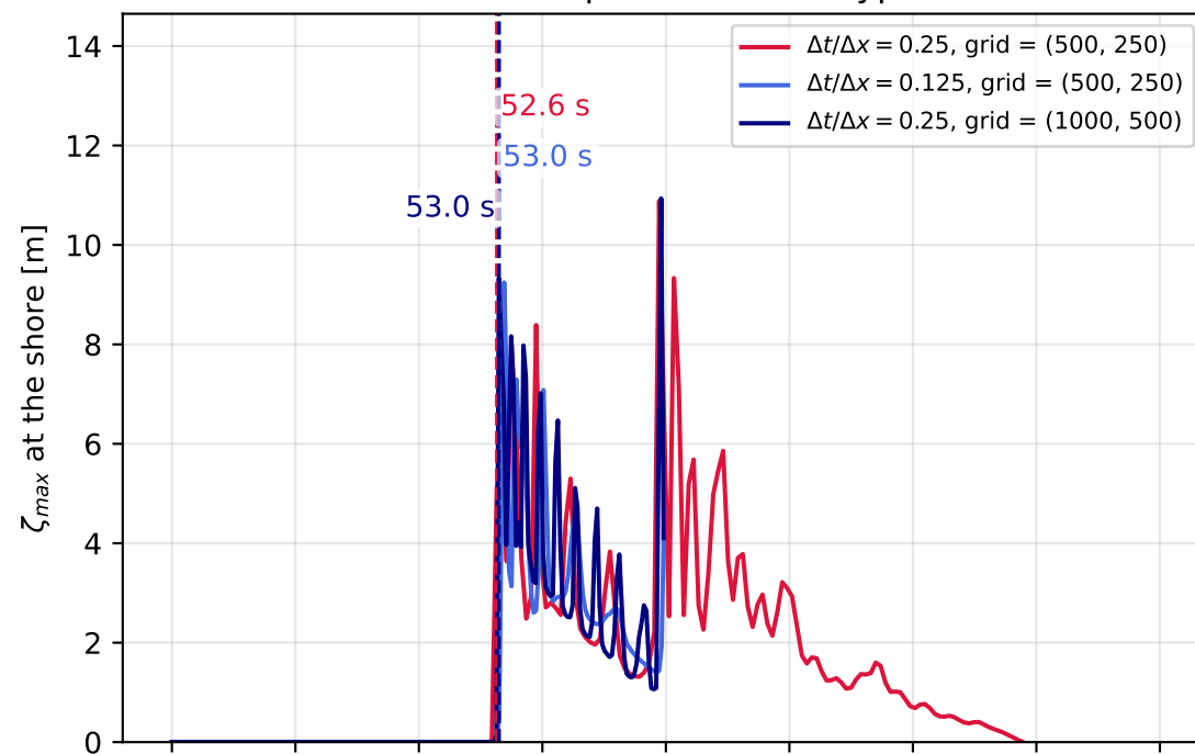
Two-step slope
