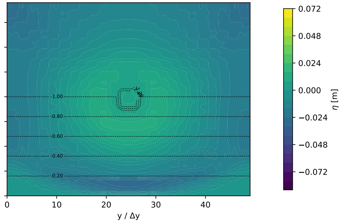
Case 2: \eta(x, y) , t=12.00 s
