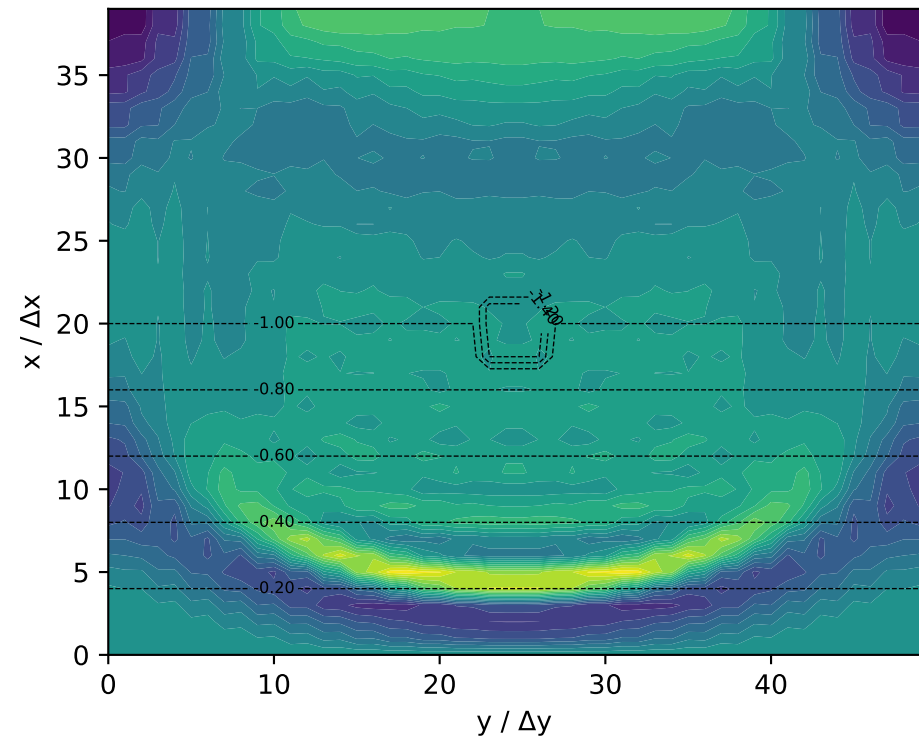
Case 1: \eta(x, y) , t=12.00 s
