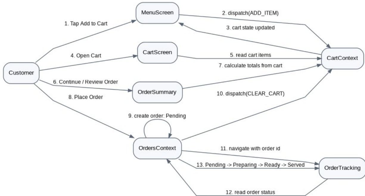
Figure 3. Sequence Diagram - Customer Places an Order
