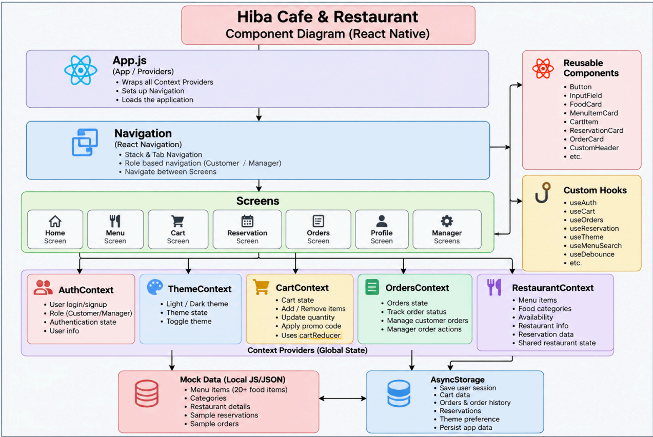
Figure 5. Component Diagram
