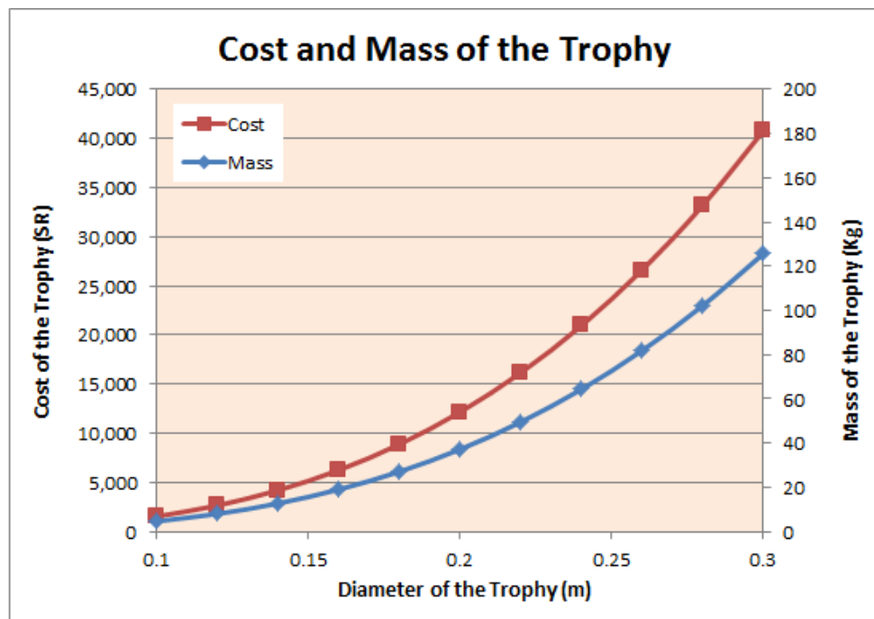
Fig. 6 calculated mass and cost of the trophy according to its diameter
