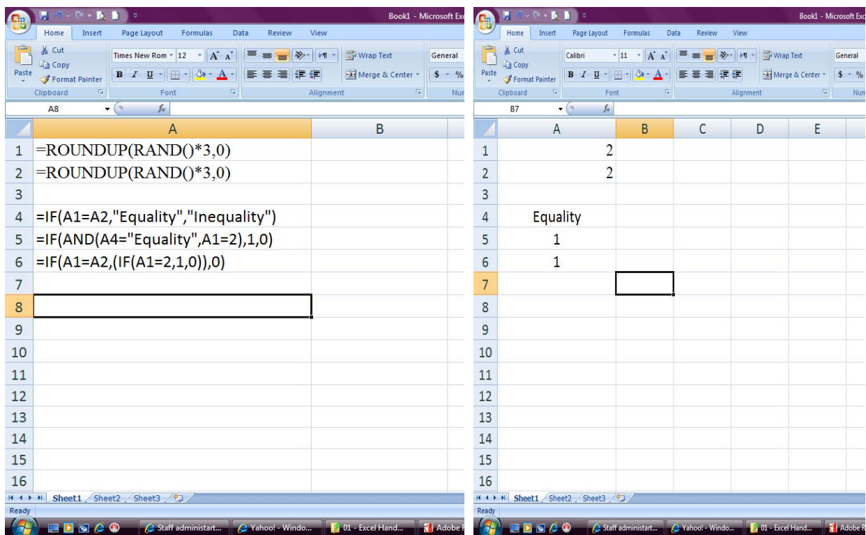
Figure (8) Example 4, IF logical function
