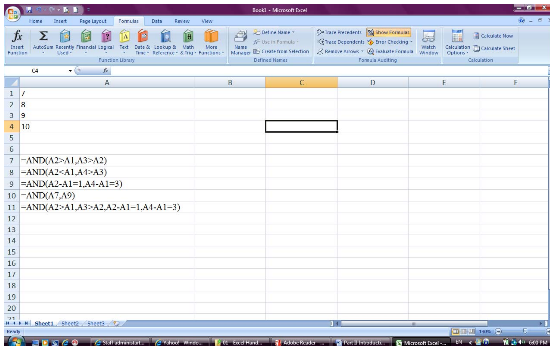
Figure (2) Spreadsheet Example for the “And” logic (Formula option)
