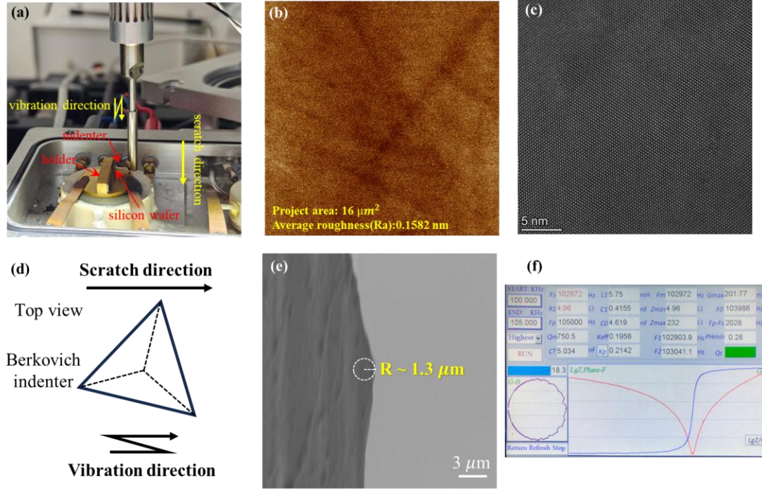
Fig. 1. Experimental setup and initial material characterization for the vibration-assisted scratch tests. (a) Configuration of the custom ultrasonic vibration device integrated with the multifunctional tribometer. (b) Initial surface morphology of the pristine monocrystalline silicon wafer. (c) HRTEM image confirming the defect-free lattice structure prior to testing. (d) Schematic of the indenter orientation relative to the [110] crystallographic scratch direction. (e) Profile of the Berkovich diamond indenter. (f) Resonant characteristics of the ultrasonic device, displaying the admittance circle and frequency sweep.
