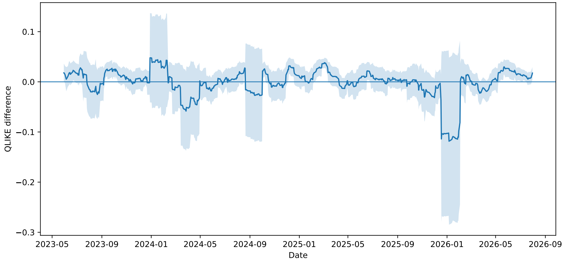
Regime-Calibrated TGARCH-X minus Baseline TGARCH-X
