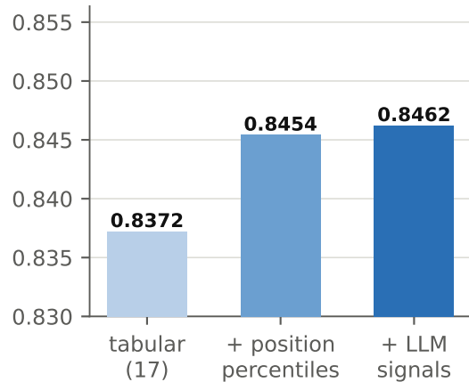
Row accuracy
