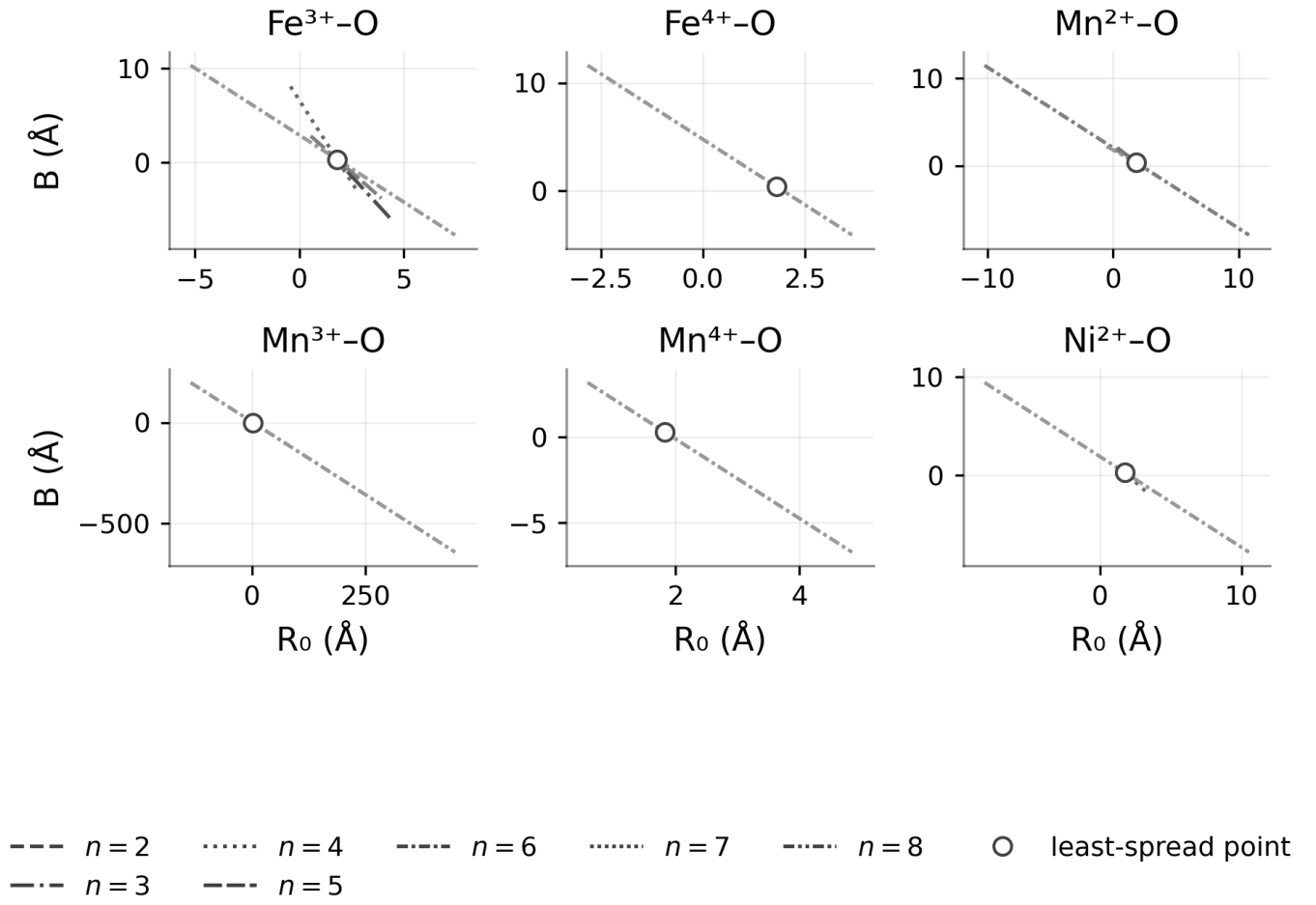
FIG. S6. n -resolved B vs. R_0 for oxidation-state-resolved 3d X-O pairs ( \text{Fe}^{3+} , \text{Fe}^{4+} , \text{Mn}^{2+} , \text{Mn}^{3+} , \text{Mn}^{4+} , \text{Ni}^{2+} ).
