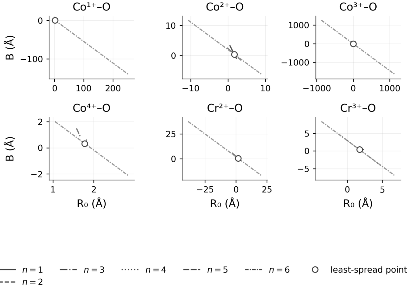
FIG. S4. n -resolved B vs. R_0 for oxidation-state-resolved 3d X-O pairs ( \text{Co}^{1+} , \text{Co}^{2+} , \text{Co}^{3+} , \text{Co}^{4+} , \text{Cr}^{2+} , \text{Cr}^{3+} ).
