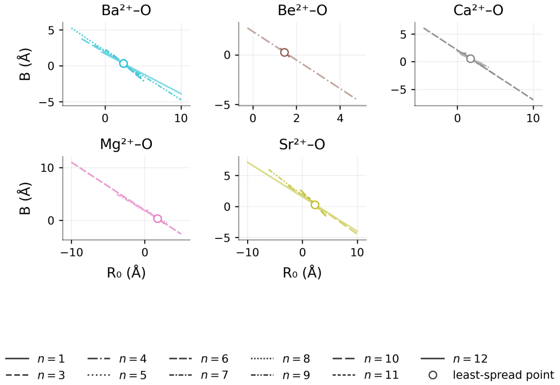
FIG. S3. n -resolved B vs. R_0 fit lines for Group 2 X-O pairs (Ba, Be, Ca, Mg, Sr).
