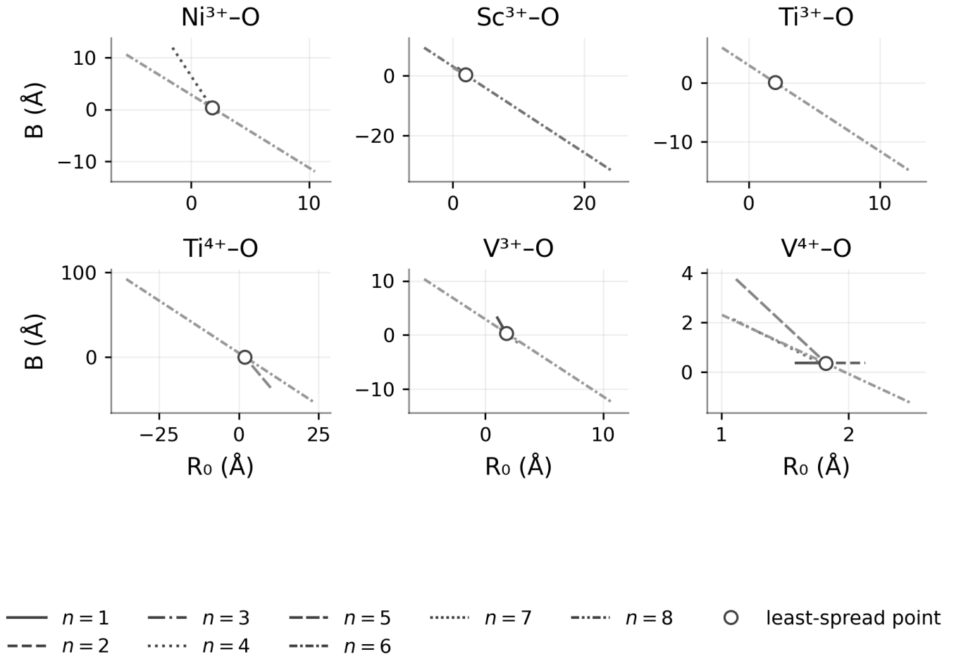
FIG. S7. n -resolved B vs. R_0 for oxidation-state-resolved 3d X-O pairs ( \text{Ni}^{3+} , \text{Sc}^{3+} , \text{Ti}^{3+} , \text{Ti}^{4+} , \text{V}^{3+} , \text{V}^{4+} ).
