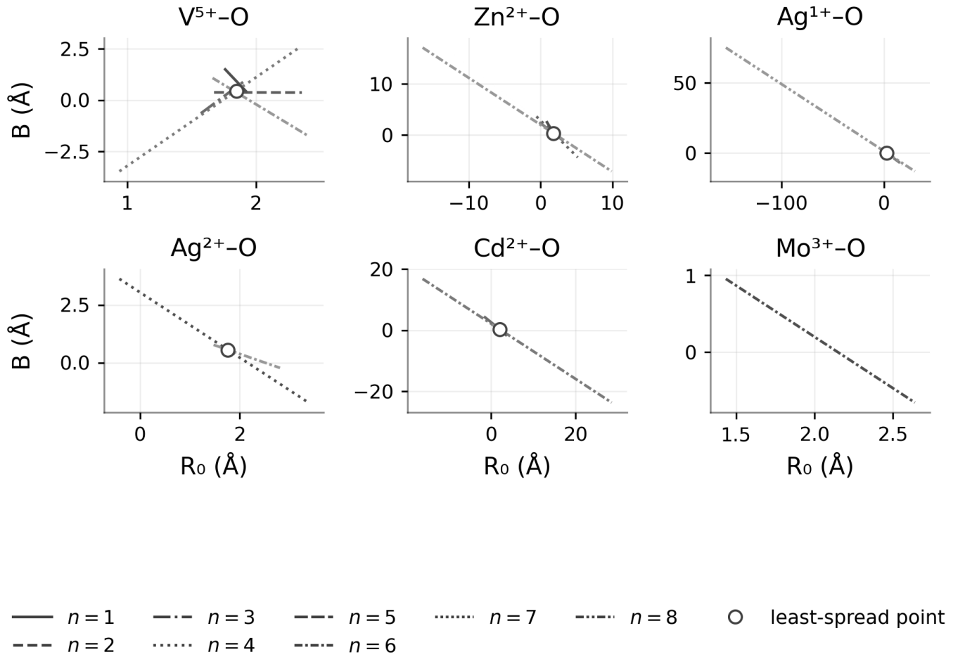
FIG. S8. n -resolved B vs. R_0 for oxidation-state-resolved 3d/4d X-O pairs ( V^{5+} , Zn^{2+} , Ag^{1+} , Ag^{2+} , Cd^{2+} , Mo^{3+} ).
