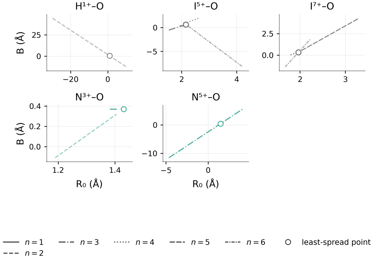
FIG. S14. n -resolved B vs. R_0 for the remaining p -block and hydrogen X-O pairs ( H^{1+} , I^{5+} , I^{7+} , N^{3+} , N^{5+} ).
