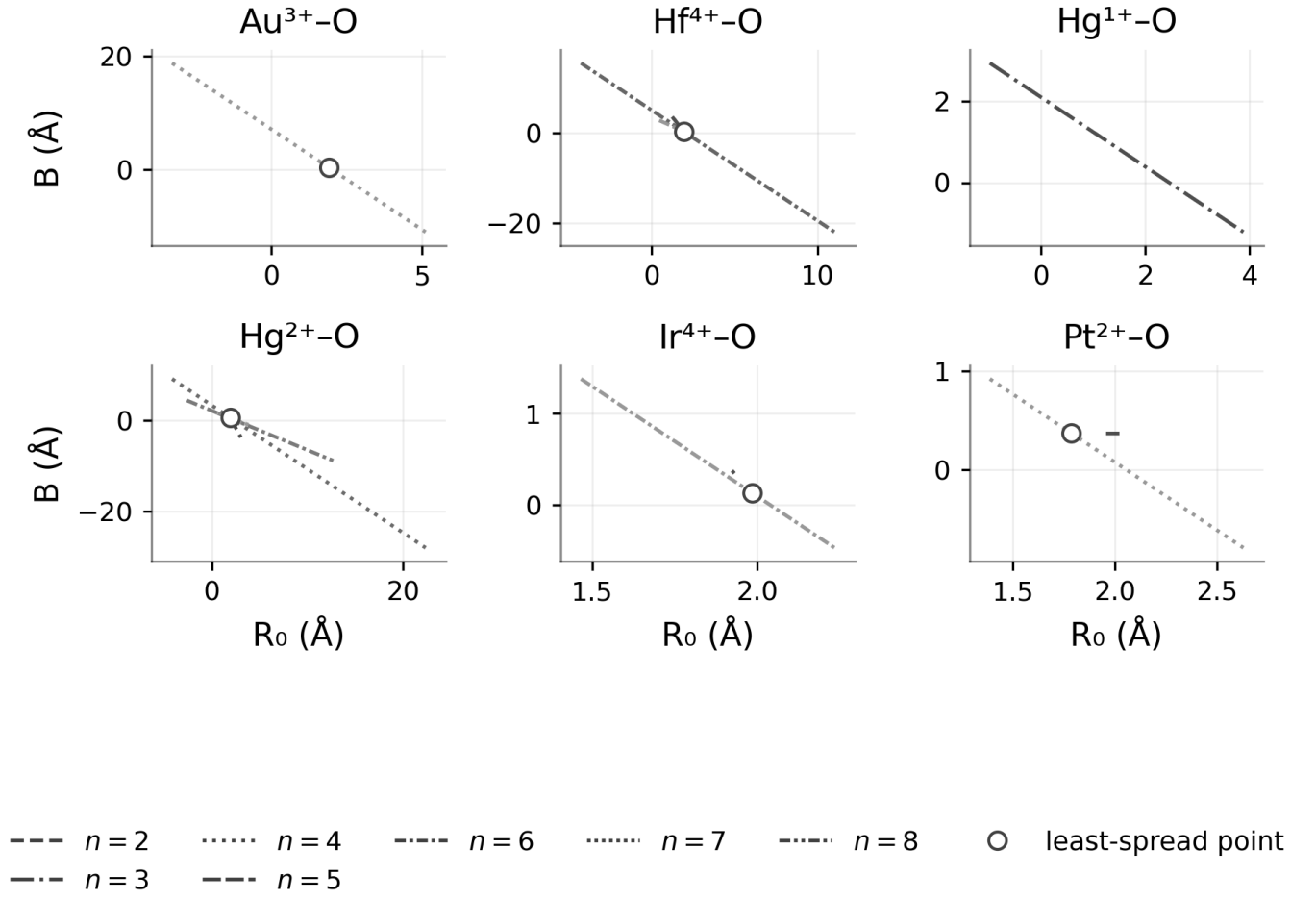
FIG. S10. n -resolved B vs. R_0 for oxidation-state-resolved 5d X-O pairs ( \text{Au}^{3+} , \text{Hf}^{4+} , \text{Hg}^{1+} , \text{Hg}^{2+} , \text{Ir}^{4+} , \text{Pt}^{2+} ).
