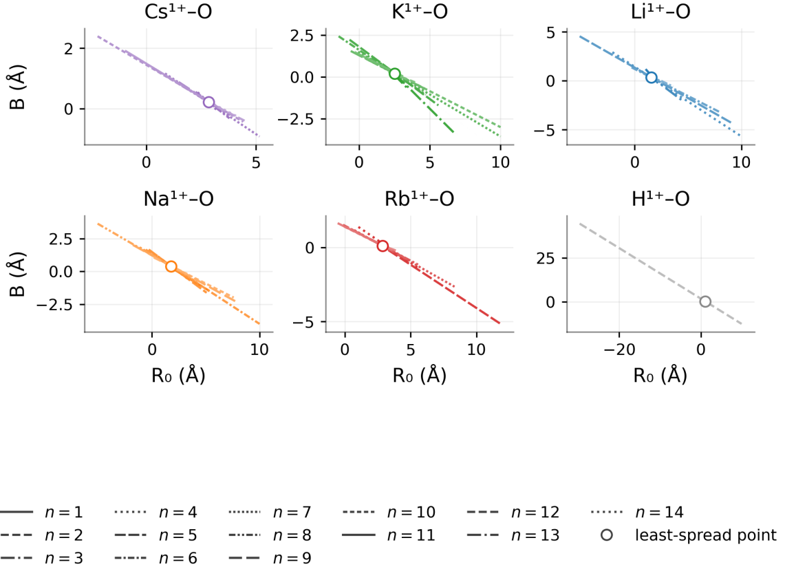
FIG. S2. n -resolved B vs. R_0 fit lines for Group 1 X-O pairs (Cs, K, Li, Na, Rb, H). Line styles distinguish coordination numbers n (legend), and the open circle marks the least-spread intersection point. The convergence of the lines defines the characteristic pair (R_0^*, B^*) for each cation.
