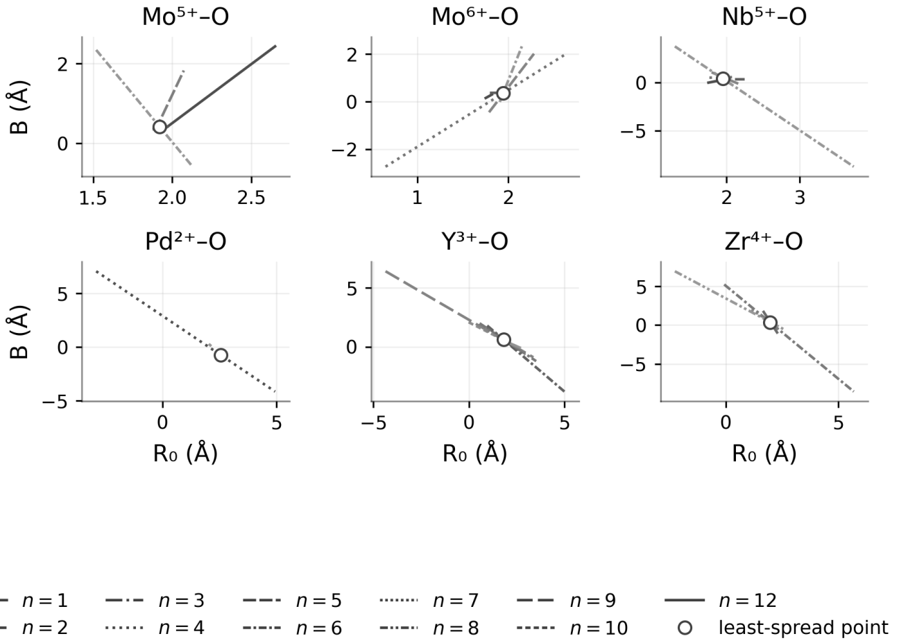
FIG. S8. n -resolved B vs. R_0 for oxidation-state-resolved 4d X-O pairs ( \text{Mo}^{5+} , \text{Mo}^{6+} , \text{Nb}^{5+} , \text{Pd}^{2+} , \text{Y}^{3+} , \text{Zr}^{4+} ).
