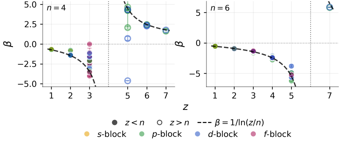
FIG. S16. Fitted slope \beta versus formal charge z for the individual cation–oxygen species summarized in main-text Fig. 1, at n = 4 (left) and n = 6 (right). Filled markers show species with z < n (negative \beta ), open markers species with z > n (positive \beta ), and dashed curves the parameter-free prediction \beta = 1/\ln(z/n) . Markers are colored by cation block and drawn semi-transparent, so darker points mark loci where the fitted slopes of multiple species coincide. Error bars show the standard error \sigma_\beta of each fitted slope. Most are smaller than the marker.
