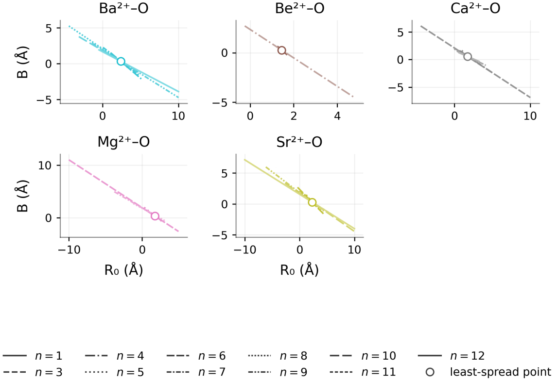
FIG. S2. n -resolved B vs. R_0 fit lines for Group 2 X-O pairs (Ba, Be, Ca, Mg, Sr).
