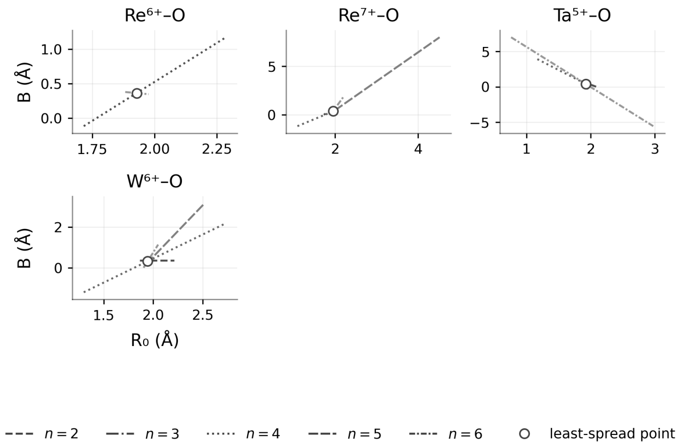
FIG. S10. n -resolved B vs. R_0 for oxidation-state-resolved 5d X-O pairs ( \text{Re}^{6+} , \text{Re}^{7+} , \text{Ta}^{5+} , \text{W}^{6+} ).
