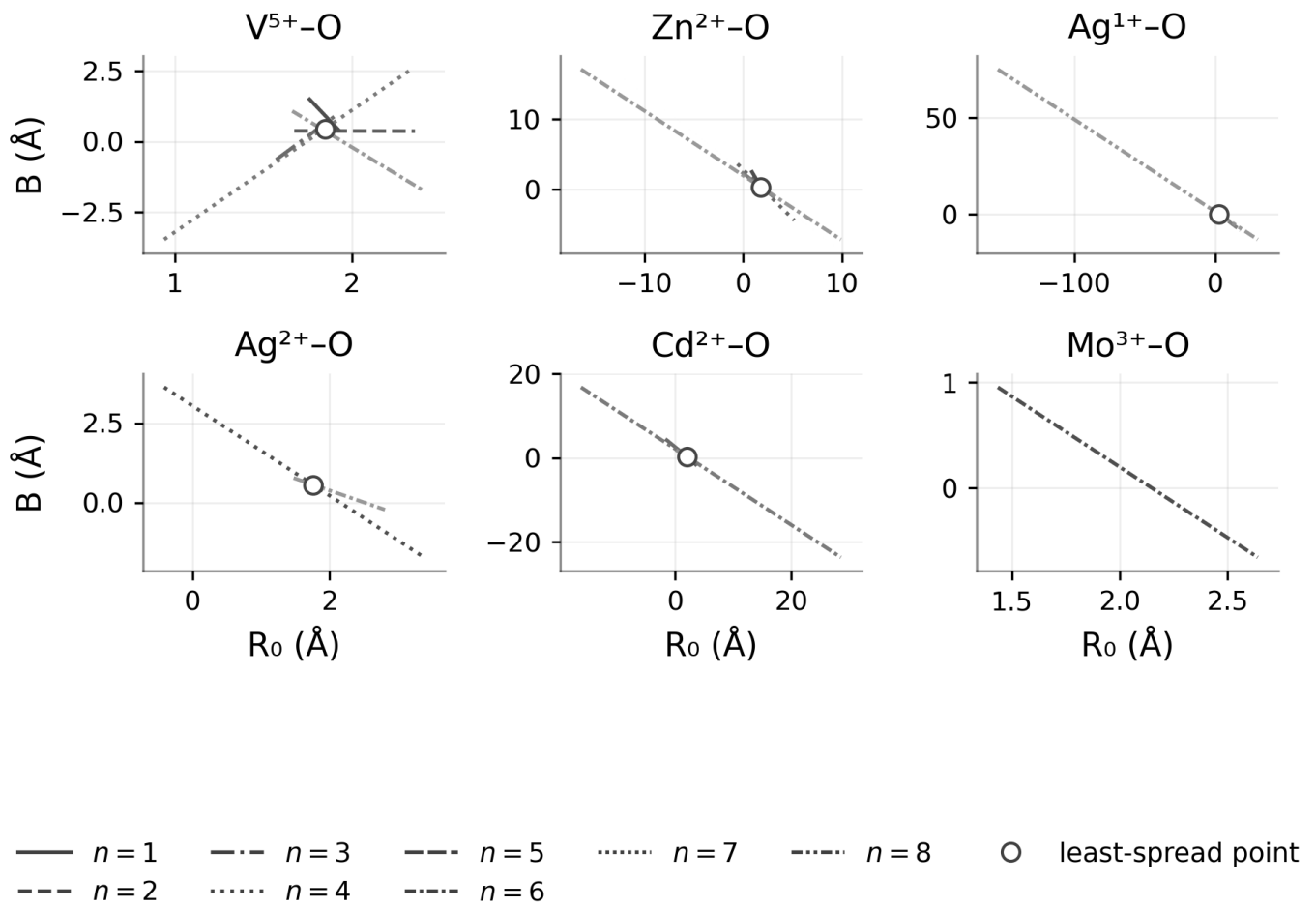
FIG. S7. n -resolved B vs. R_0 for oxidation-state-resolved 3d/4d X-O pairs ( V^{5+} , Zn^{2+} , Ag^{1+} , Ag^{2+} , Cd^{2+} , Mo^{3+} ).
