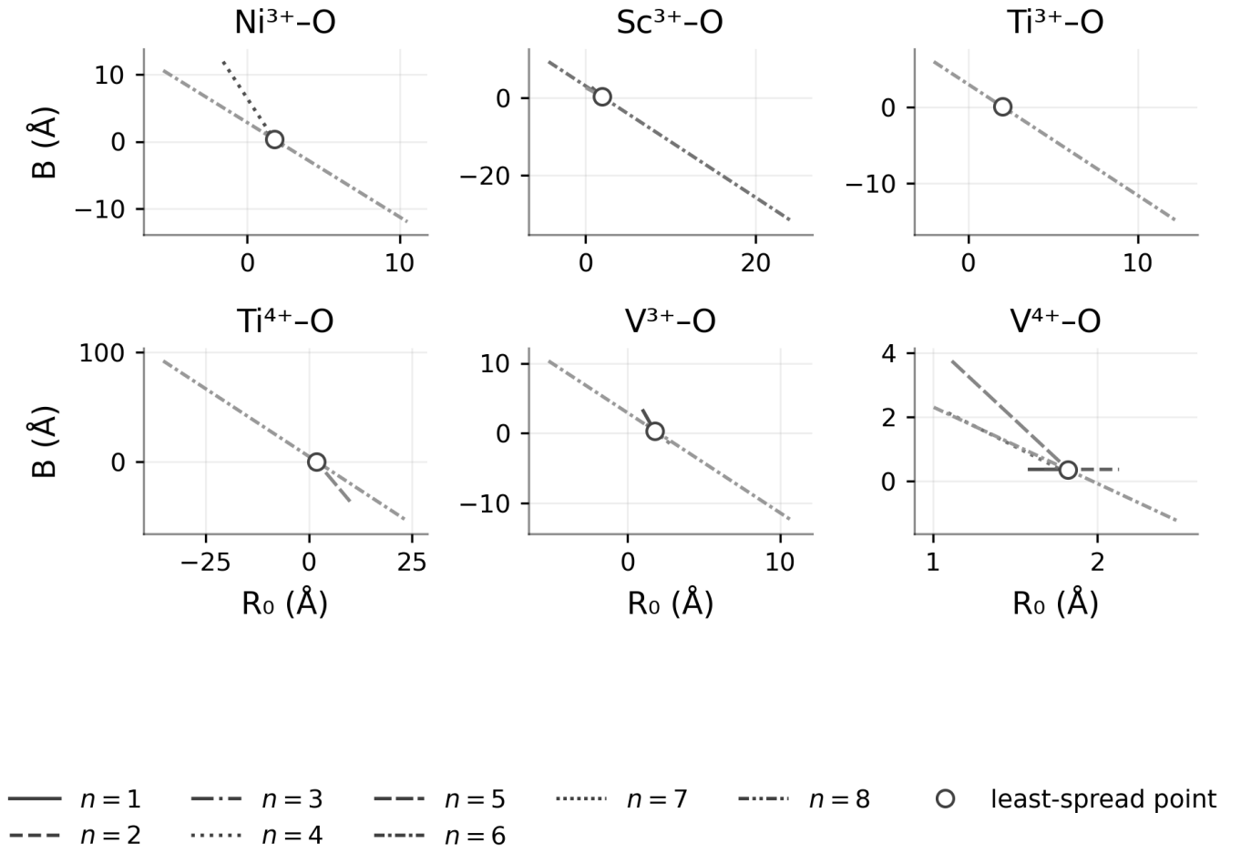
FIG. S6. n -resolved B vs. R_0 for oxidation-state-resolved 3d X-O pairs ( \text{Ni}^{3+} , \text{Sc}^{3+} , \text{Ti}^{3+} , \text{Ti}^{4+} , \text{V}^{3+} , \text{V}^{4+} ).
