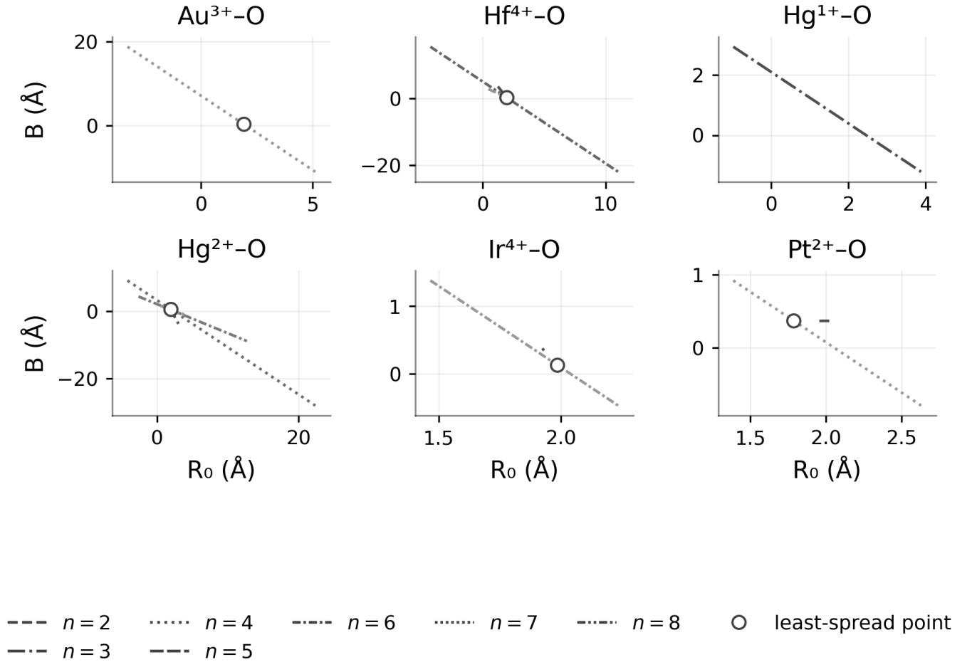
FIG. S9. n -resolved B vs. R_0 for oxidation-state-resolved 5d X-O pairs ( \text{Au}^{3+} , \text{Hf}^{4+} , \text{Hg}^{1+} , \text{Hg}^{2+} , \text{Ir}^{4+} , \text{Pt}^{2+} ).
