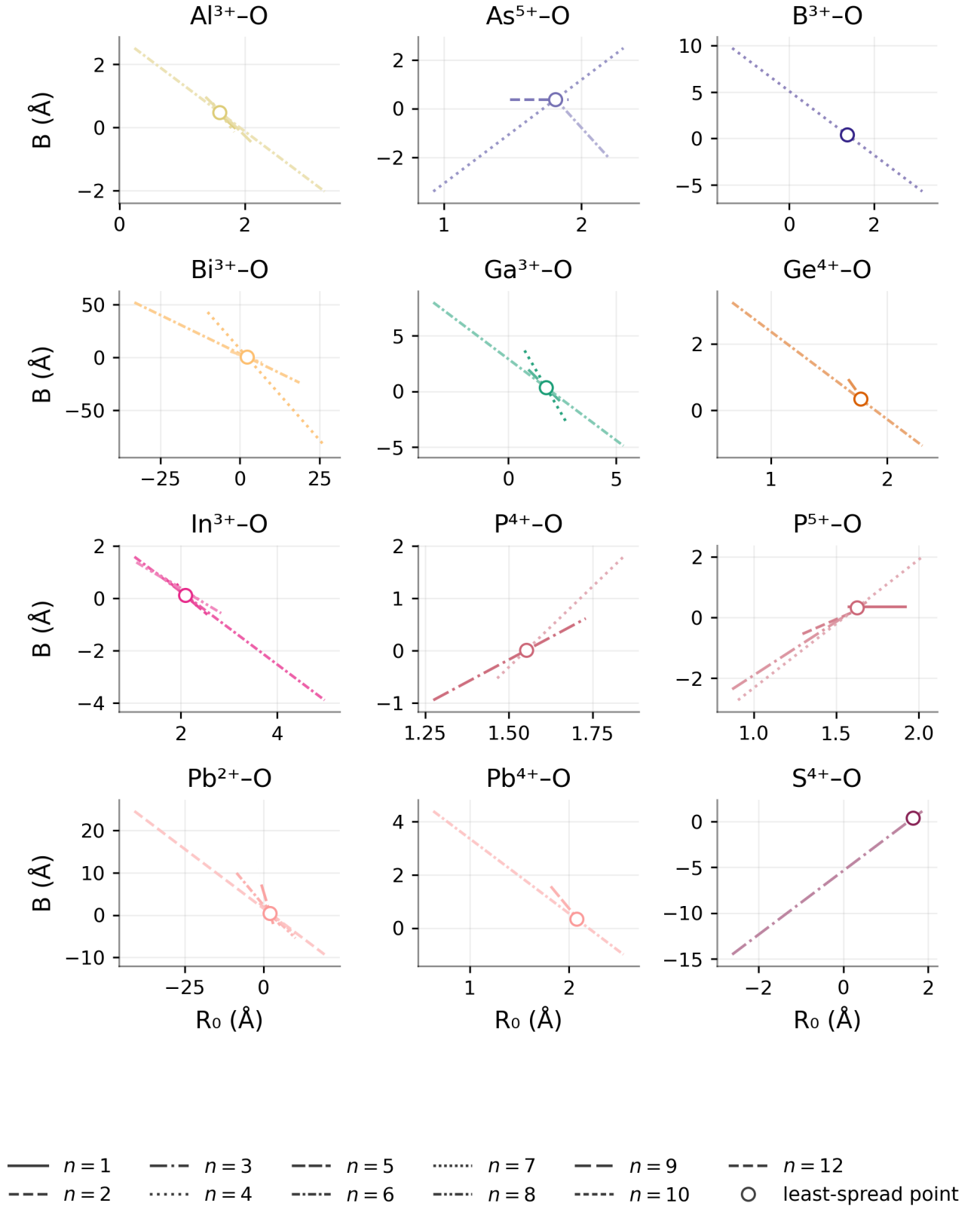
FIG. S11. n -resolved B vs. R_0 for oxidation-state-resolved p -block X-O pairs ( \text{Al}^{3+} - \text{S}^{4+} ).
