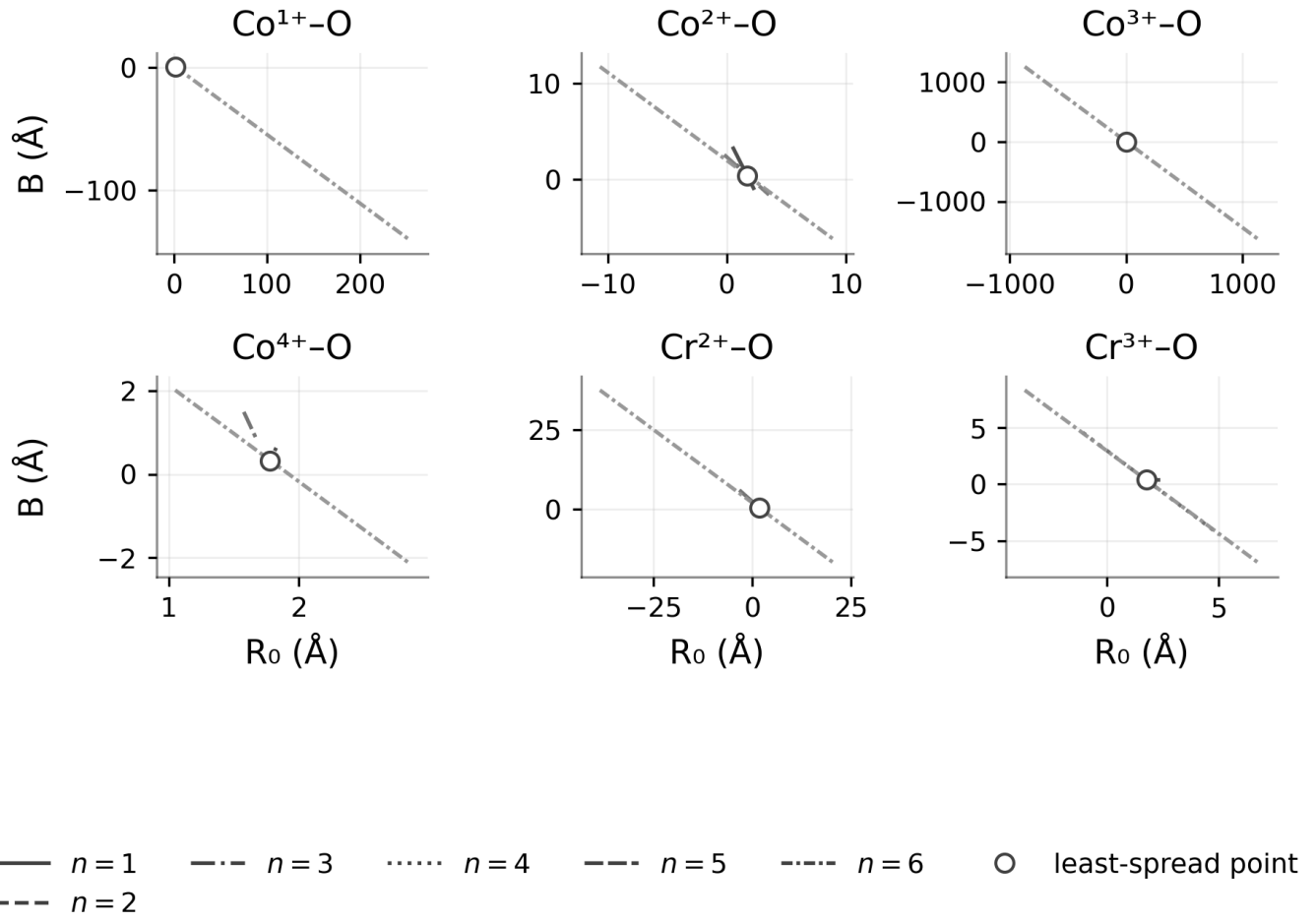
FIG. S3. n -resolved B vs. R_0 for oxidation-state-resolved 3d X-O pairs ( \text{Co}^{1+} , \text{Co}^{2+} , \text{Co}^{3+} , \text{Co}^{4+} , \text{Cr}^{2+} , \text{Cr}^{3+} ).
