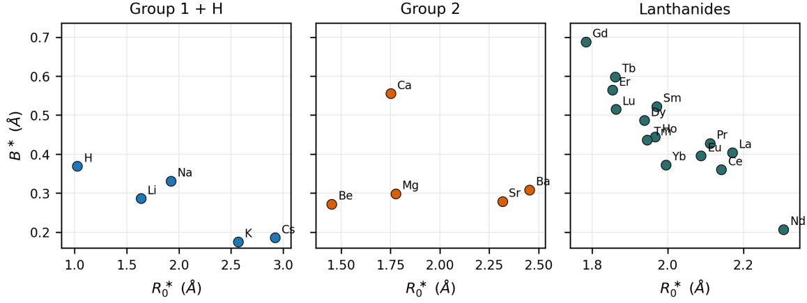
FIG. S17. Characteristic (R_0^*, B^*) for Group 1 including H^+ (left), Group 2 (center), and trivalent lanthanides (right).
