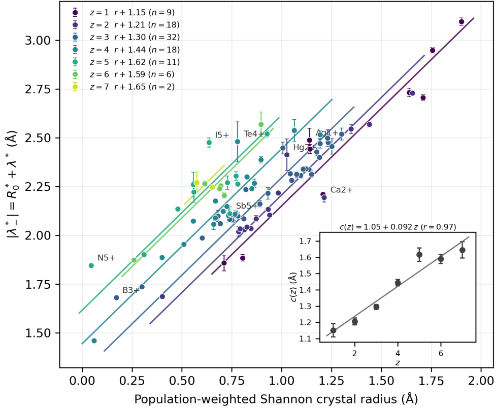
FIG. S20. Magnitude of the second inversion root, |\lambda^*| = R_0^* + \lambda^* , versus the population-weighted Shannon crystal radius [7] for 96 screening-branch cation species. Lines are unit-slope fits |\lambda^*| = r_{cr} + c(z) for each formal charge z . Error bars are the propagated \sigma_\lambda of Table S1. The inset shows the fitted offsets c(z) with standard errors and the linear law c(z) = 1.05 + 0.092z ( r = 0.97 ). Labels mark the largest per-class residuals.
