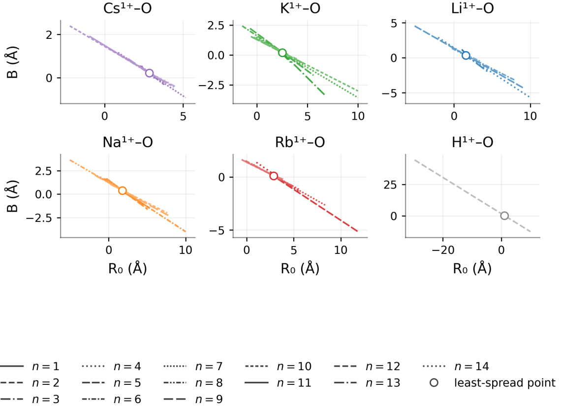
FIG. S1. n -resolved B vs. R_0 fit lines for Group 1 X-O pairs (Cs, K, Li, Na, Rb, H). Line styles distinguish coordination numbers n (legend), and the open circle marks the least-spread intersection point. The convergence of the lines defines the characteristic pair (R_0^*, B^*) for each cation.
