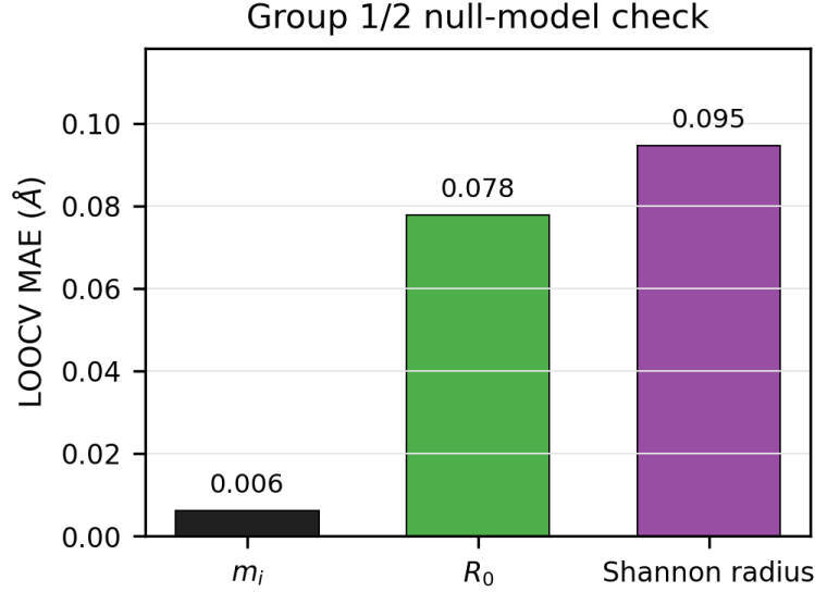
FIG. S19. Leave-one-out null-model check for the ten Group 1/Group 2 binary oxides used in Fig. 2 of the main text. Bars report the mean absolute error of linear regressions against the bond-valence shell centroid m_i , the fitted intercept R_0 , and the Shannon cation radius.
