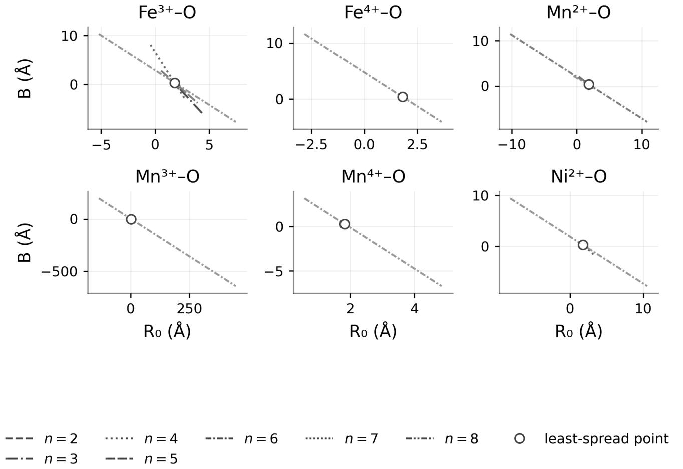
FIG. S5. n -resolved B vs. R_0 for oxidation-state-resolved 3d X-O pairs ( \text{Fe}^{3+} , \text{Fe}^{4+} , \text{Mn}^{2+} , \text{Mn}^{3+} , \text{Mn}^{4+} , \text{Ni}^{2+} ).
