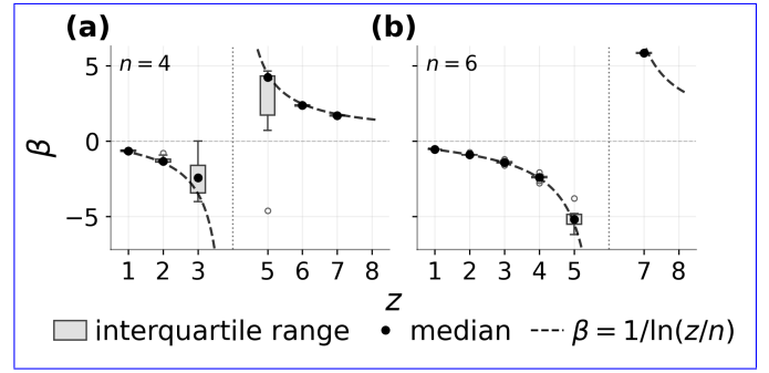
FIG. 1. Fitted slope \beta vs. formal charge z for 94 cation–oxygen species at (a) n = 4 (68 cations) and (b) n = 6 (82 cations). 56 cations contribute at both coordinations, giving 150 fitted slopes in total. Boxes span the interquartile range of the per-species slopes at each z , black points mark the median, whiskers extend to the most extreme slopes within 1.5\times the interquartile range, and open circles mark slopes beyond the whiskers. Dashed curves: \beta = 1/\ln(z/n) . The pole at z = n separates the negative-slope ( z < n ) and positive-slope ( z > n ) branches of Eq. (5). Species at z = n are omitted. Per-species slopes are resolved in the Supplemental Material [18].
